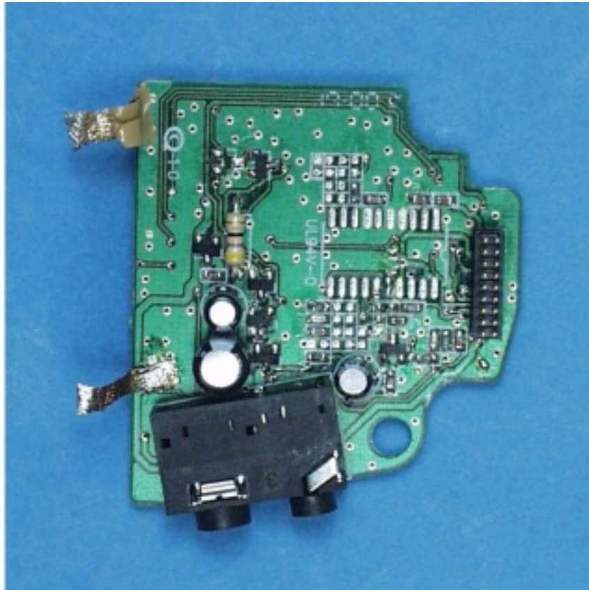
RF Board, Rear
