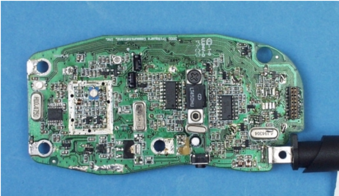
Top Main w/o Shields
