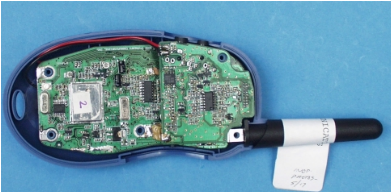
Top Main/RF Board
