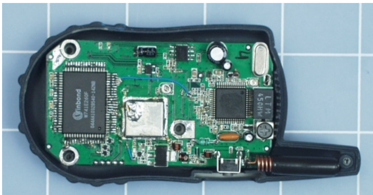
Top View Circuit Board
