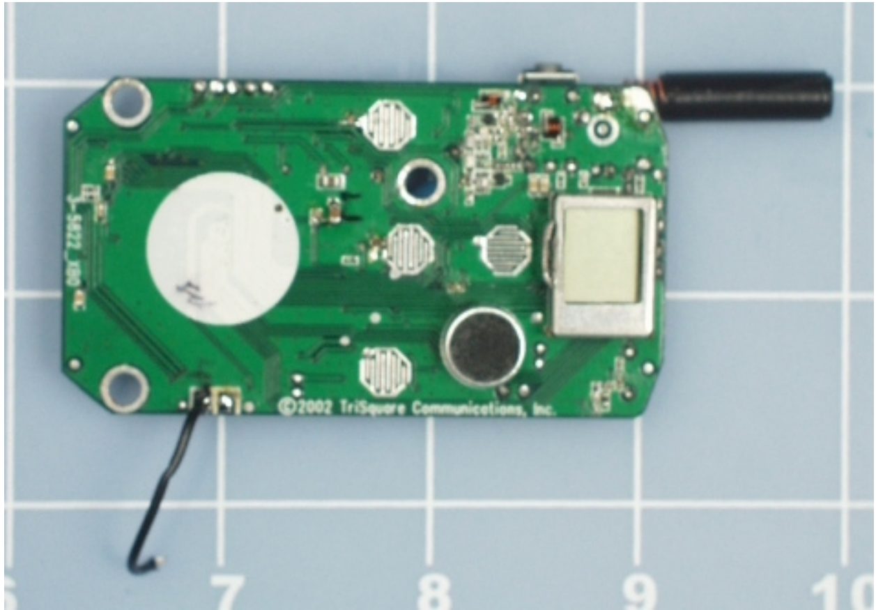
Bottom View Circuit Board
