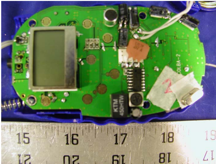
Main Board - Solder View
