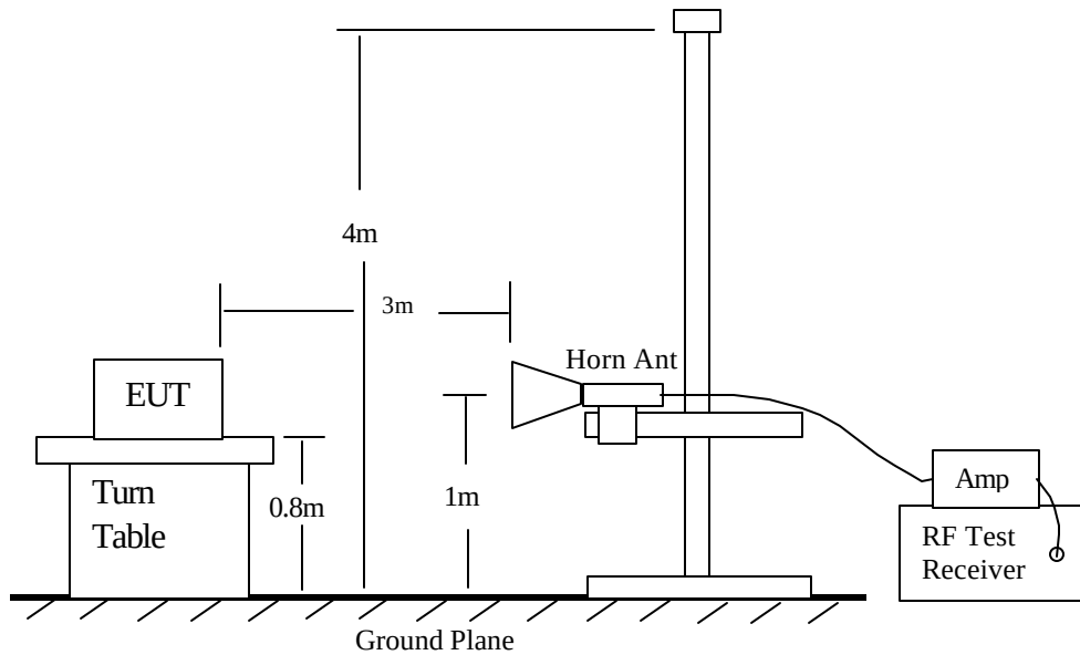
Figure 2: Radiated Emission Above 1000 MHz
