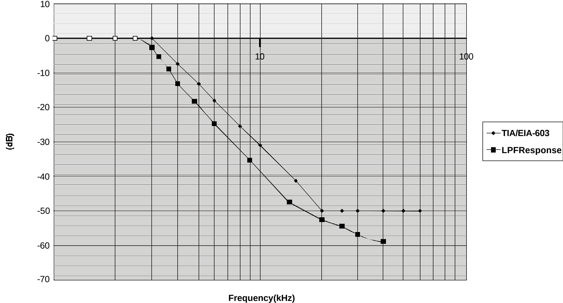
AudioLowPassFilterResponse
