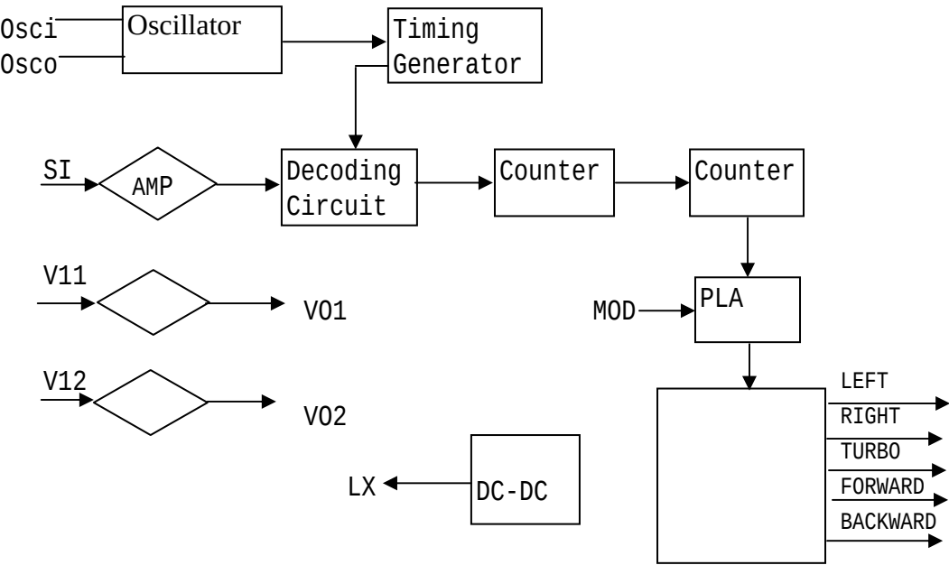
RX-2B Block diagram
