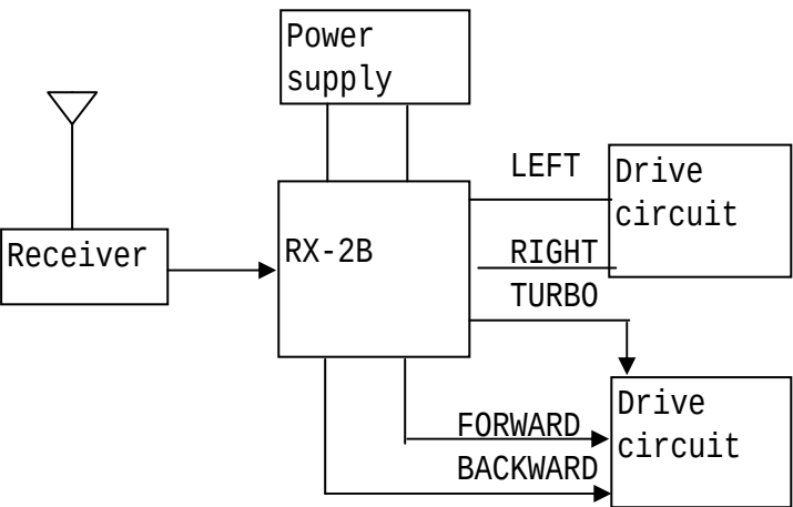
Receiver block diagram
