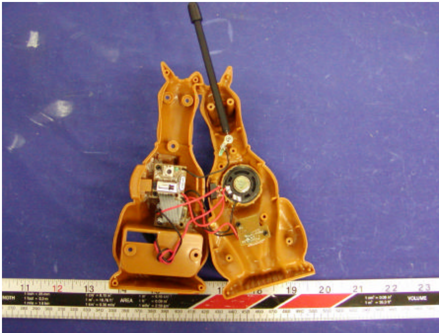
Chassis – Cover off View
