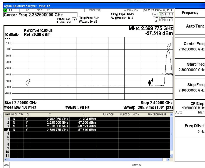
2DH5_Ant1_Low_2402_Peak
