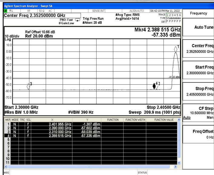
3DH5_Ant1_Low_2402_Peak
