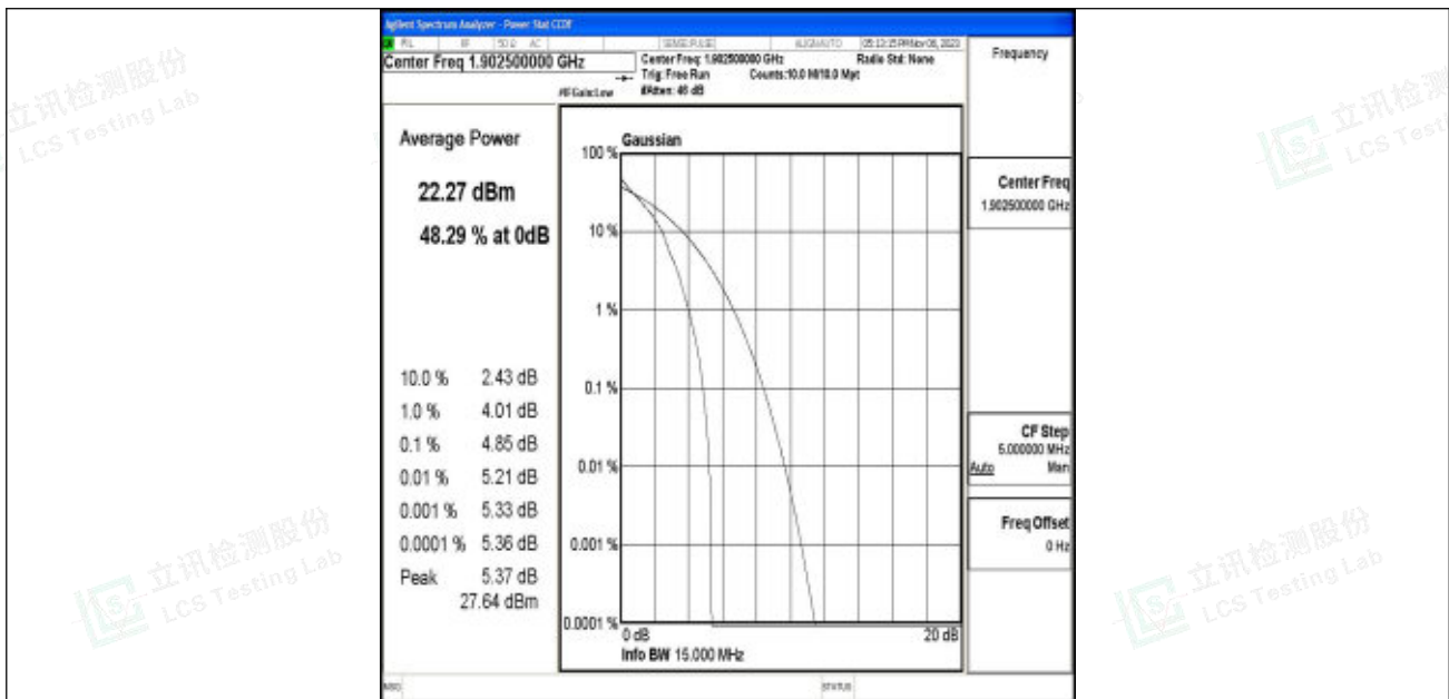
Band2-15MHz-64QAM-19125-1RB#0-PASS
