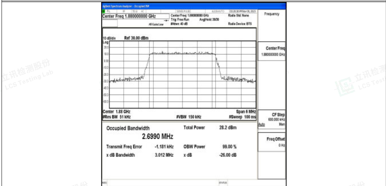
Band2-3MHz-16QAM-18900-15RB#0-PASS
