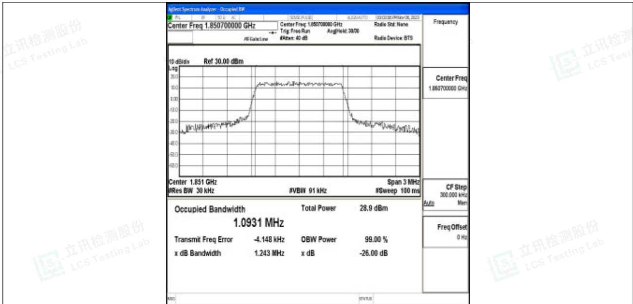
Band2-1.4MHz-64QAM-18607-6RB#0-PASS
