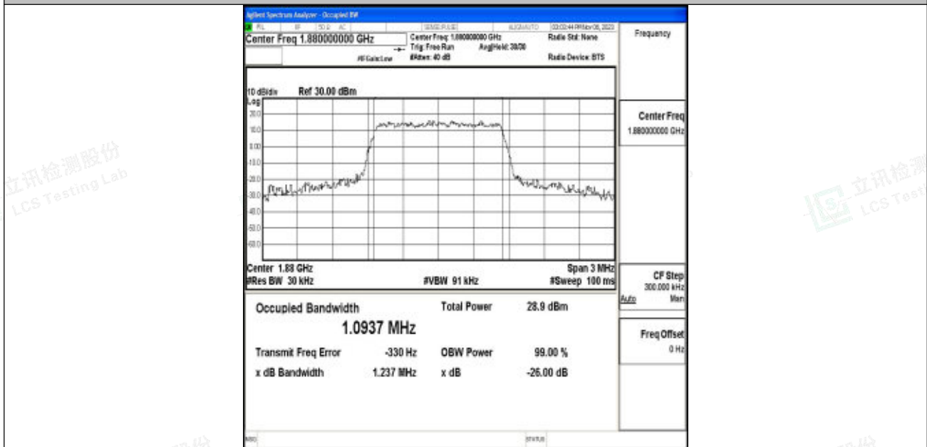
Band2-1.4MHz-64QAM-18900-6RB#0-PASS
