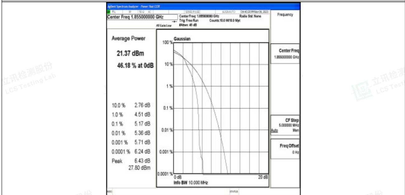
Band2-10MHz-16QAM-18650-1RB#0-PASS
