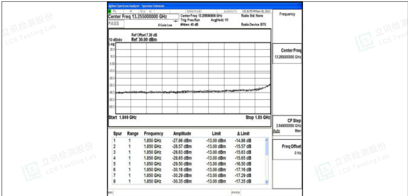
Band2_3MHz_64QAM_18615_15RB#0
