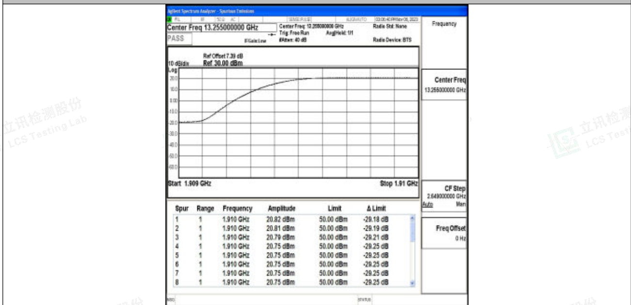
Band2_1.4MHz_16QAM_19193_1RB#5
