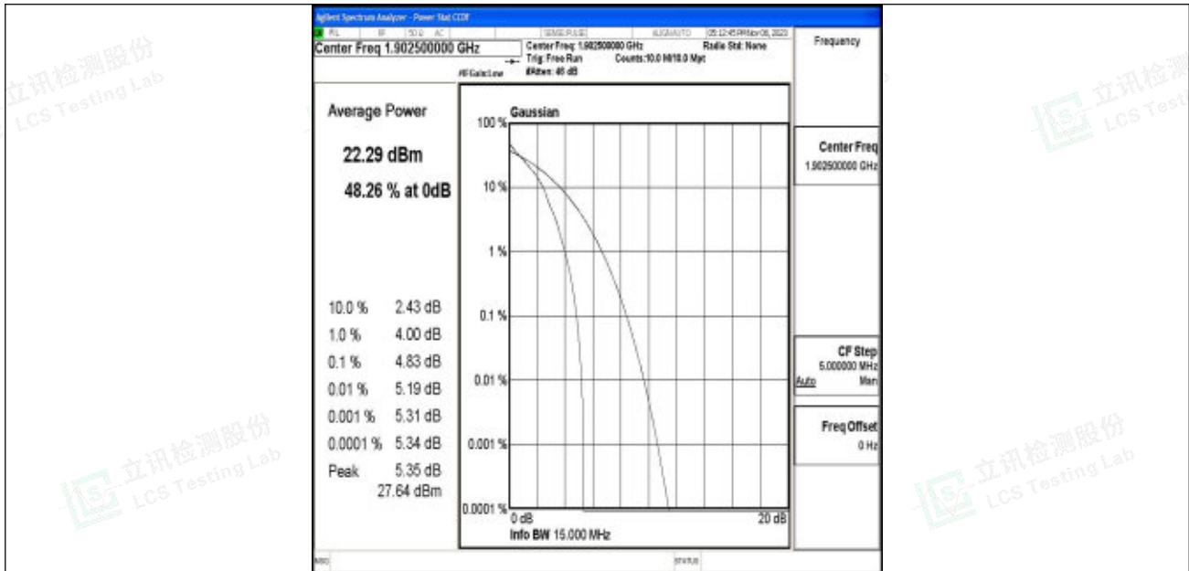
Band2-15MHz-QPSK-19125-1RB#0-PASS
