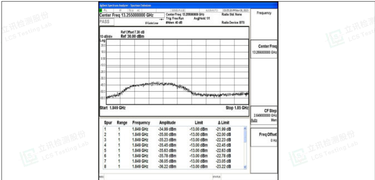
Band2_1.4MHz_16QAM_18607_1RB#5
