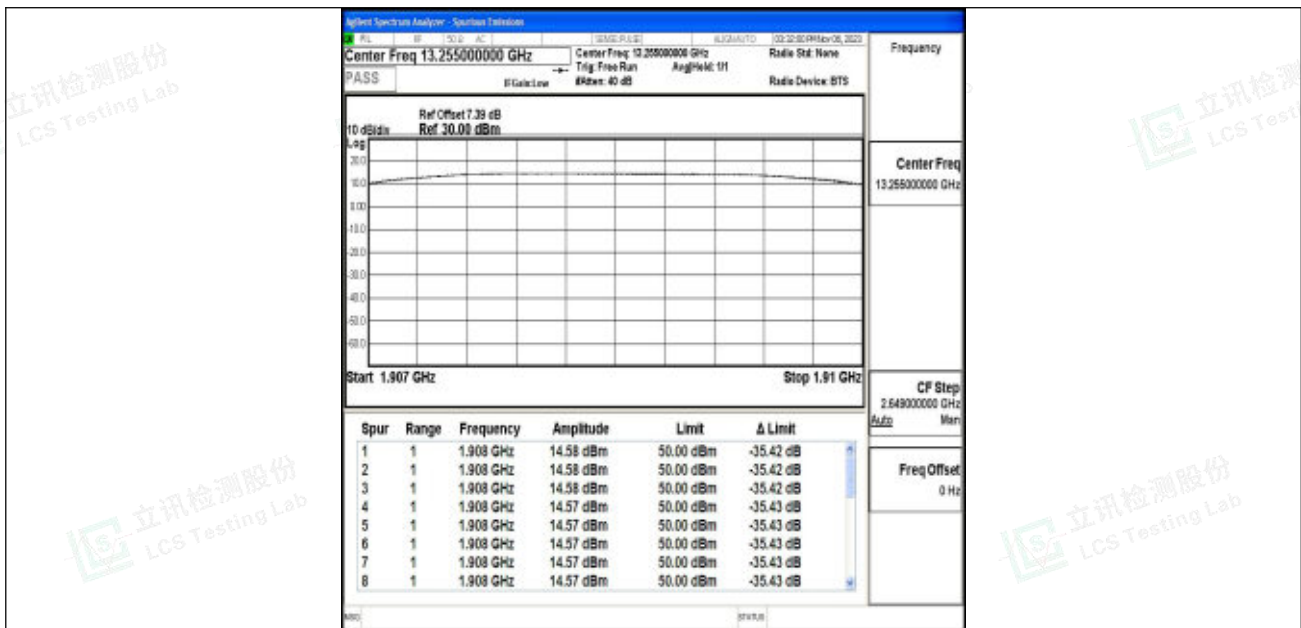
Band2_3MHz_16QAM_19185_15RB#0
