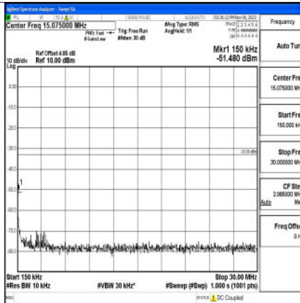
Band2_3MHz_64QAM_18900_1RB#0_0.15~30_0.15~30
