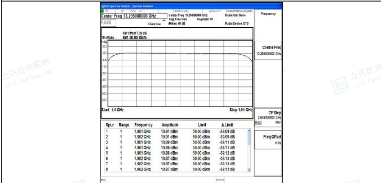
Band2_10MHz_QPSK_19150_50RB#0
