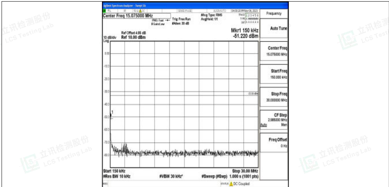
Band2_5MHz_QPSK_18625_1RB#0_0.15~30_0.15~30
