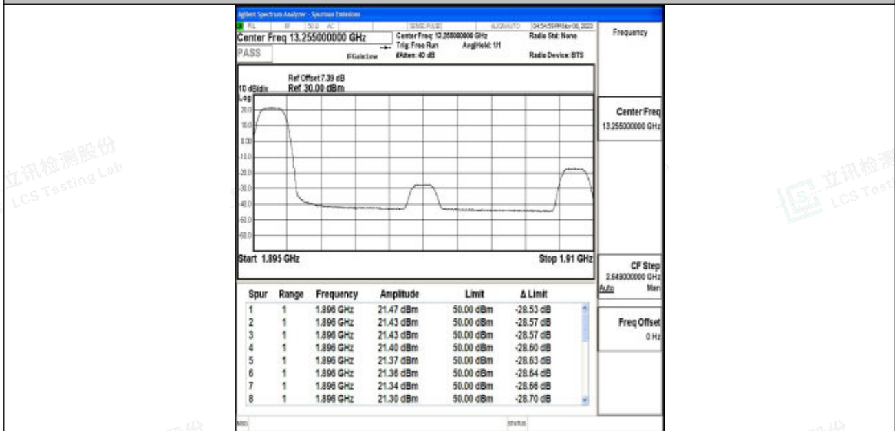
Band2_15MHz_64QAM_19125_1RB#0
