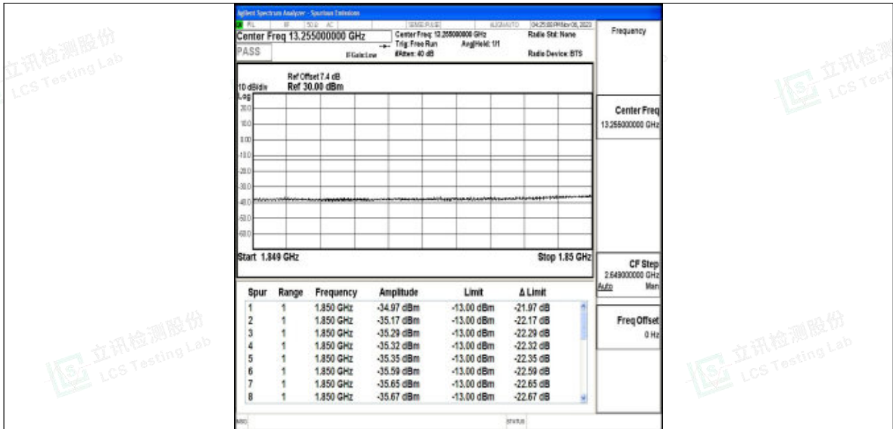
Band2_10MHz_64QAM_18650_50RB#0
