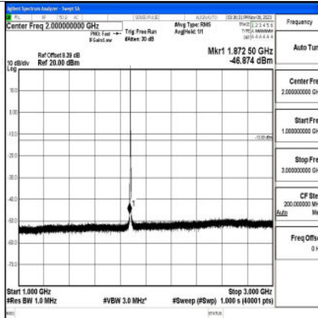
Band2_3MHz_64QAM_18900_1RB#0_1000~3000_1000~3000
