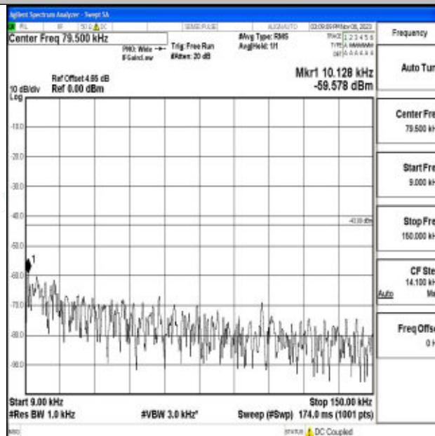
Band2_1.4MHz_64QAM_18607_1RB#0_0.009~0.15_0.009~0.15
