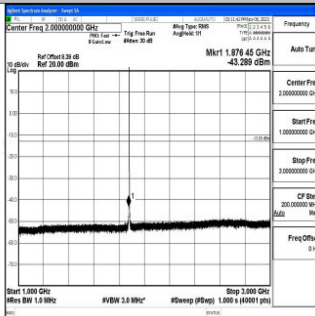
Band2_1.4MHz_64QAM_18900_1RB#0_1000~3000_1000~3000
