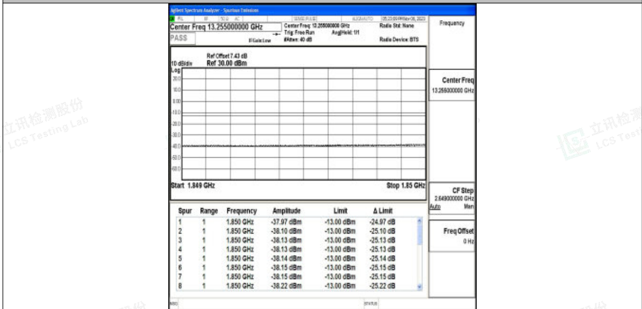
Band2_20MHz_16QAM_18700_100RB#0
