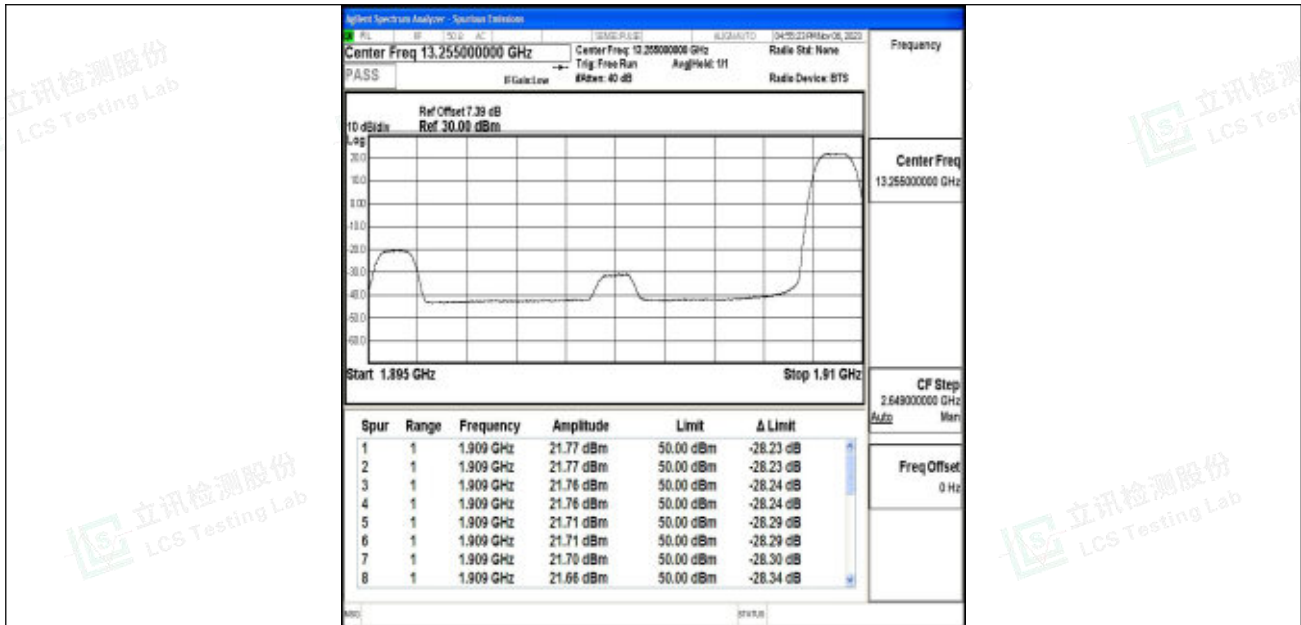
Band2_15MHz_64QAM_19125_1RB#74
