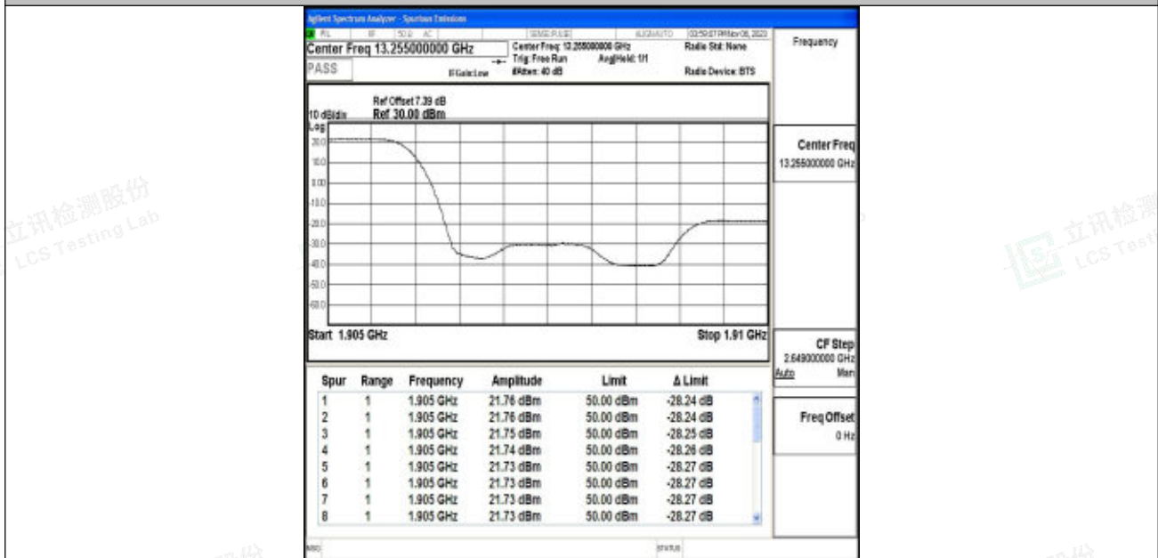
Band2_5MHz_64QAM_19175_1RB#0
