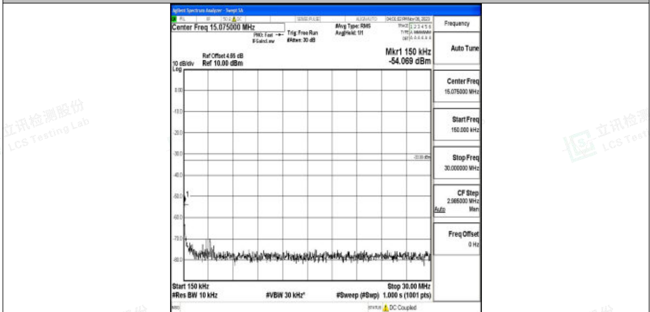
Band2_5MHz_16QAM_18625_1RB#0_0.15~30_0.15~30
