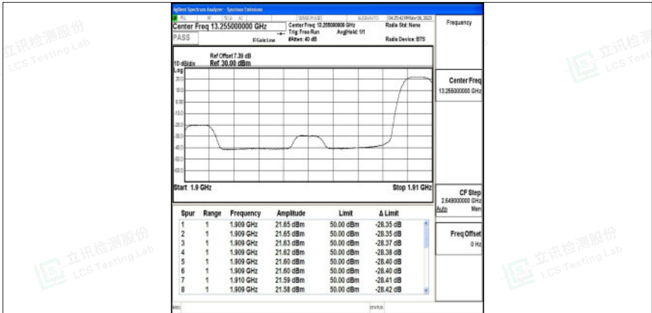
Band2_10MHz_QPSK_19150_1RB#49
