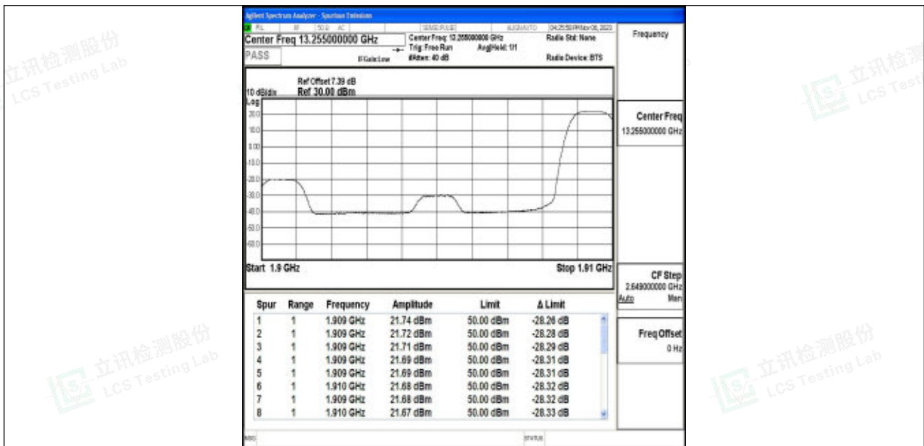
Band2_10MHz_64QAM_19150_1RB#49
