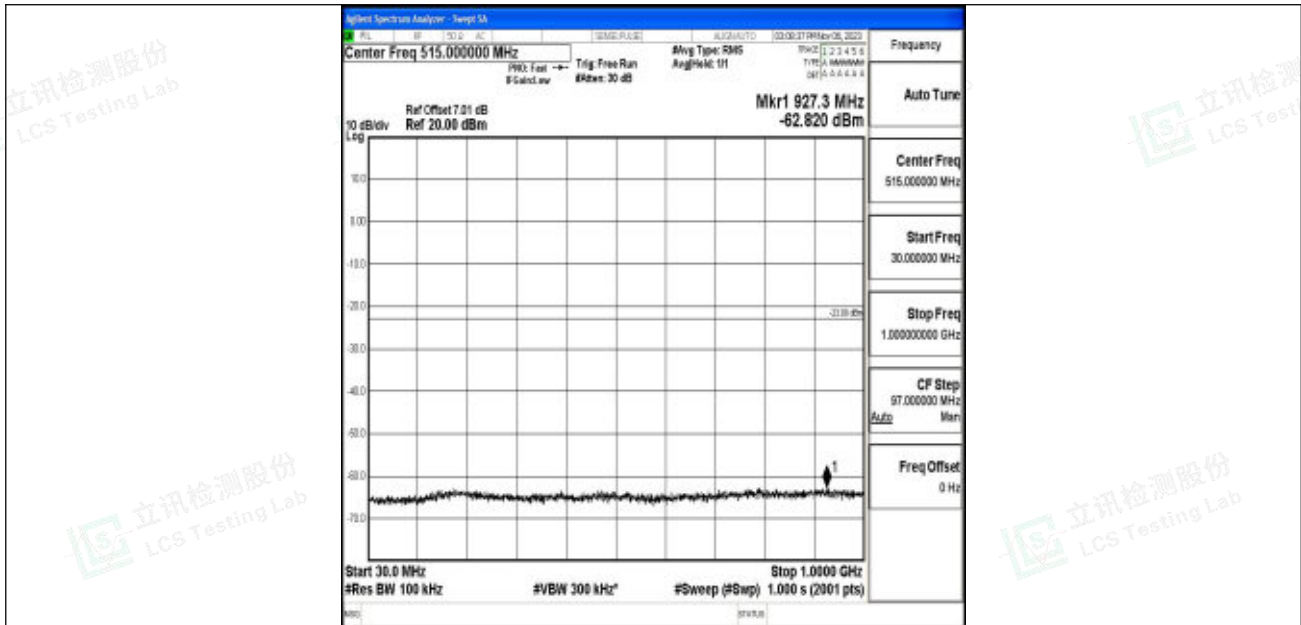
Band2_1.4MHz_16QAM_18607_1RB#0_30~1000_30~1000
