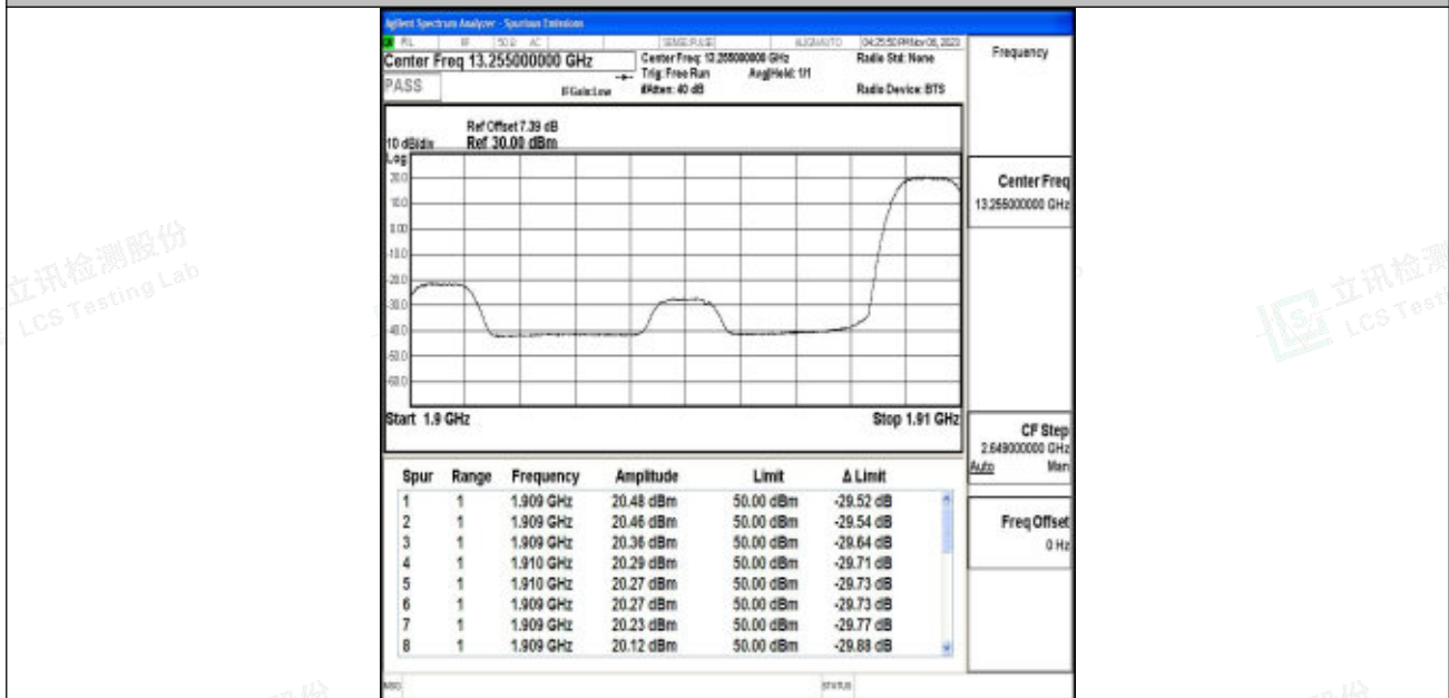
Band2_10MHz_16QAM_19150_1RB#49
