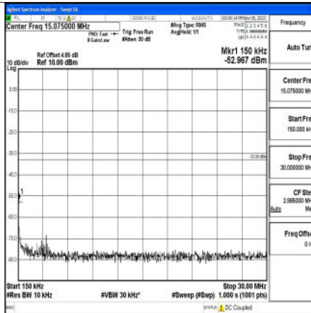
Band2_1.4MHz_64QAM_18607_1RB#0_0.15~30_0.15~30
