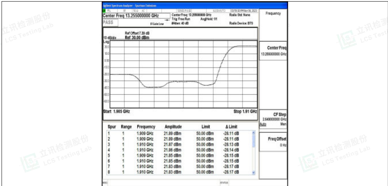
Band2_5MHz_64QAM_19175_1RB#24
