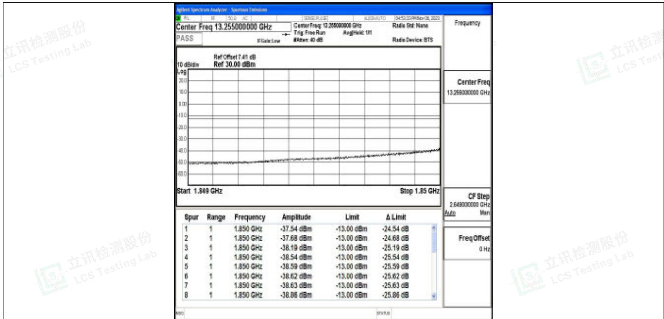
Band2_15MHz_QPSK_18675_1RB#0
