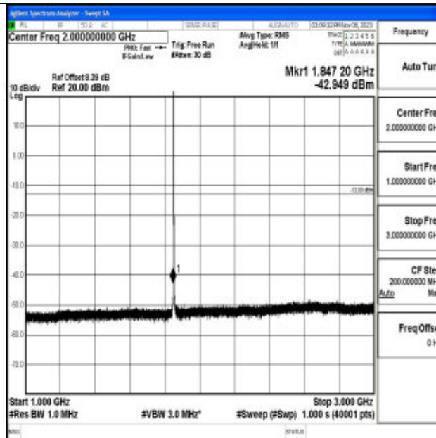
Band2_1.4MHz_64QAM_18607_1RB#0_1000~3000_1000~3000
