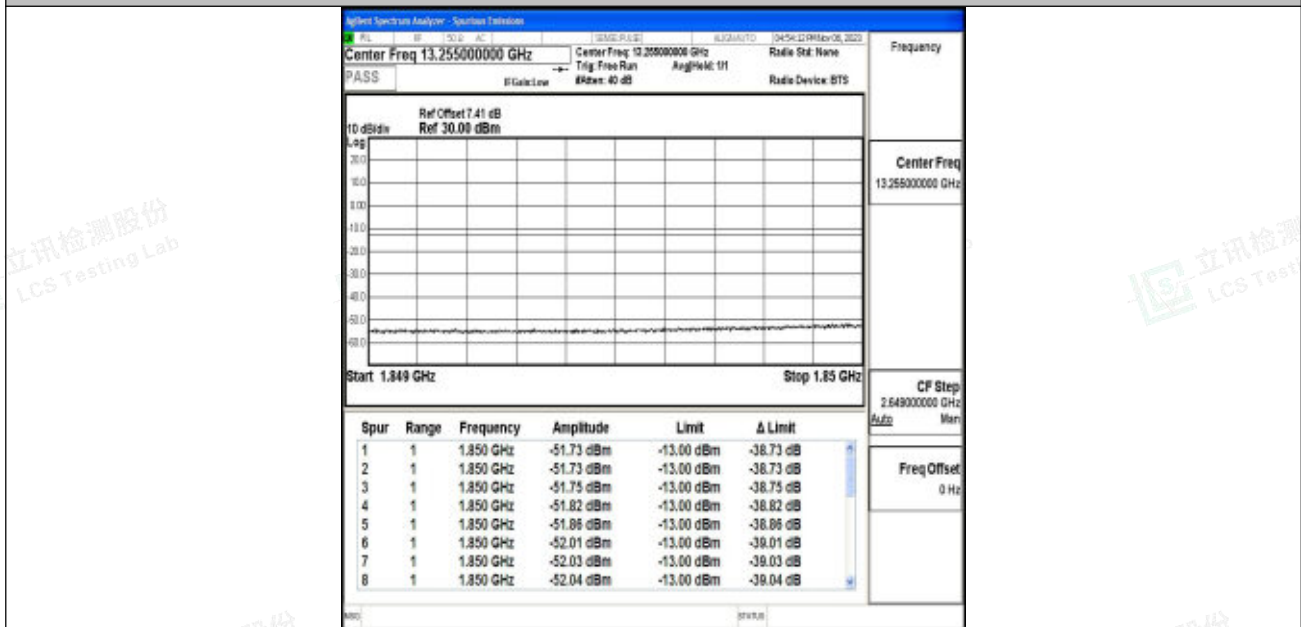
Band2_15MHz_64QAM_18675_1RB#74
