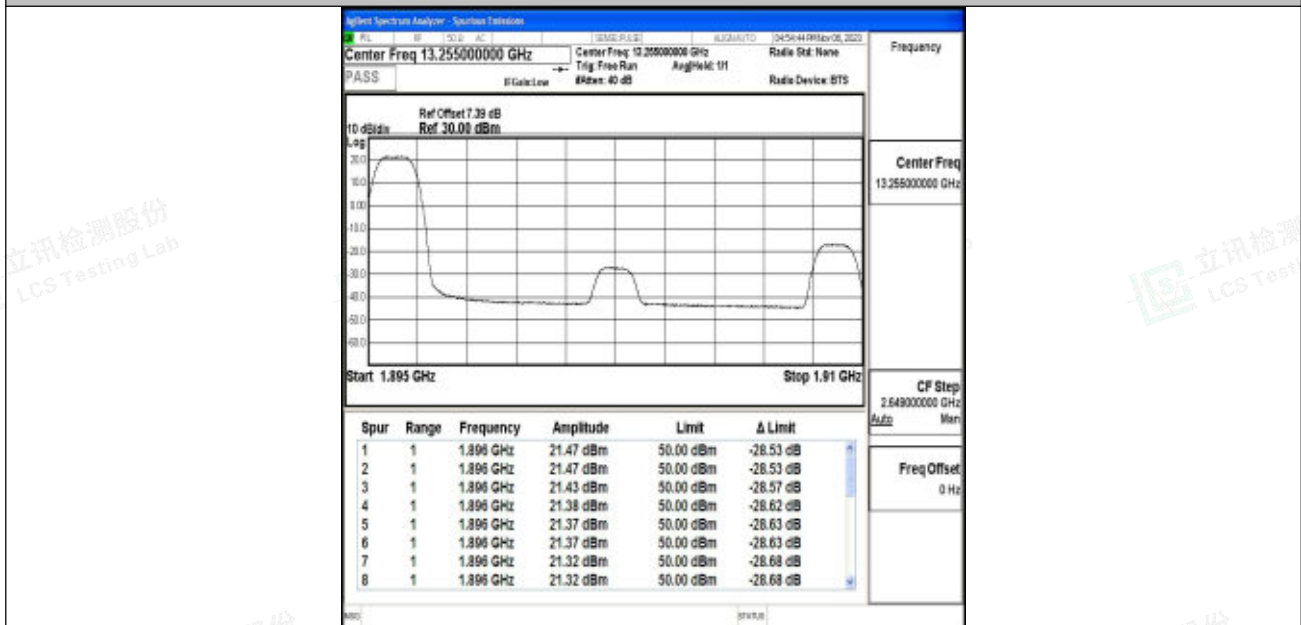
Band2_15MHz_QPSK_19125_1RB#0
