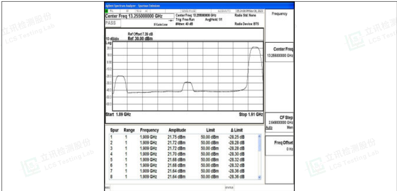
Band2_20MHz_64QAM_19100_1RB#99
