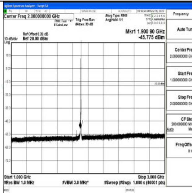
Band2_3MHz_64QAM_19185_1RB#0_1000~3000_1000~3000
