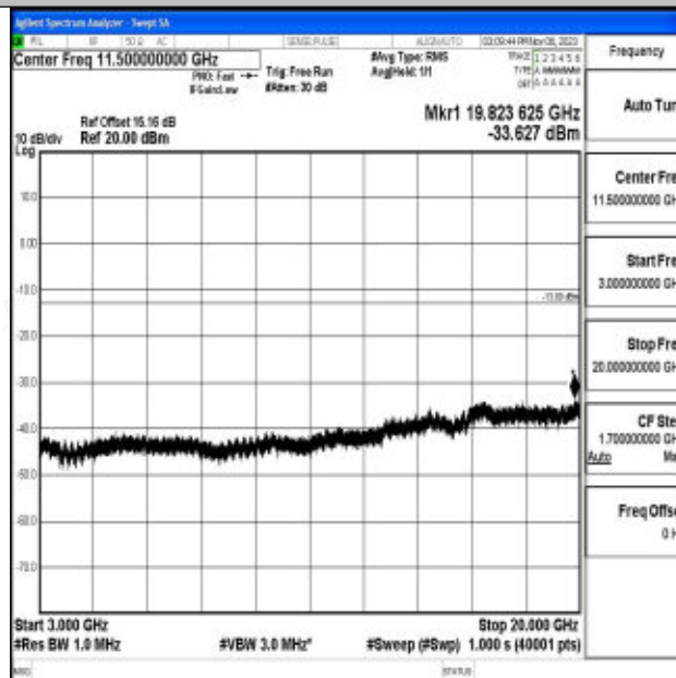
Band2_1.4MHz_64QAM_18607_1RB#0_3000~20000_3000~20000
