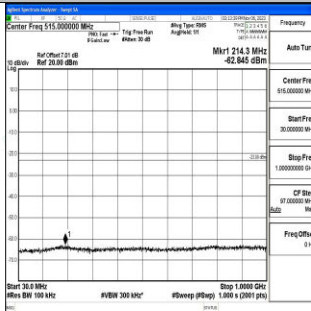
Band2_1.4MHz_64QAM_19193_1RB#0_30~1000_30~1000
