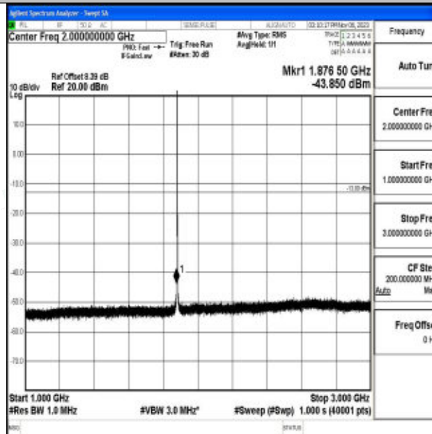
Band2_1.4MHz_QPSK_18900_1RB#0_1000~3000_1000~3000
