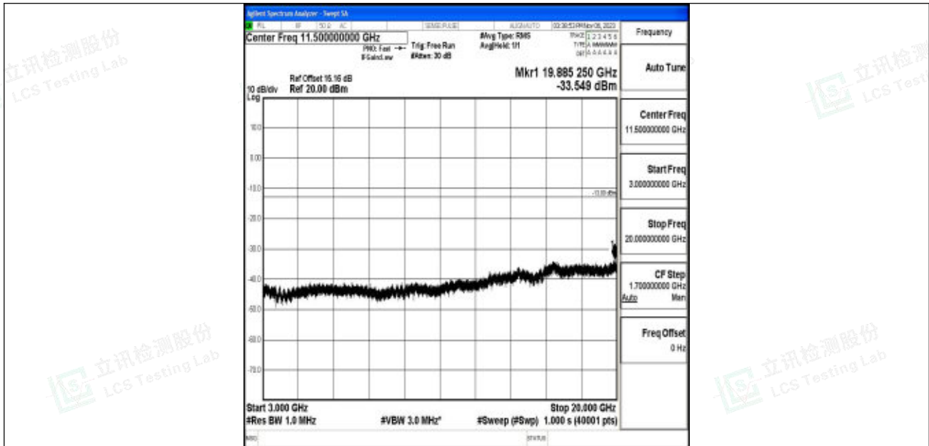
Band2_3MHz_64QAM_19185_1RB#0_3000~20000_3000~20000
