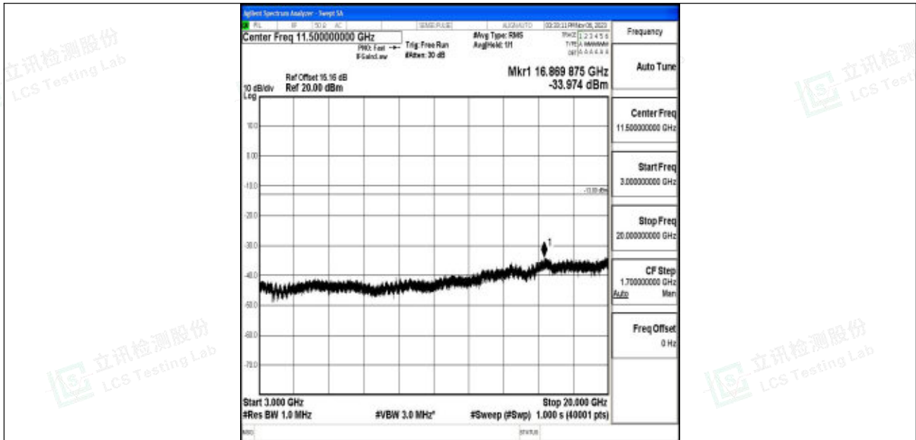
Band2_3MHz_QPSK_18615_1RB#0_3000~20000_3000~20000
