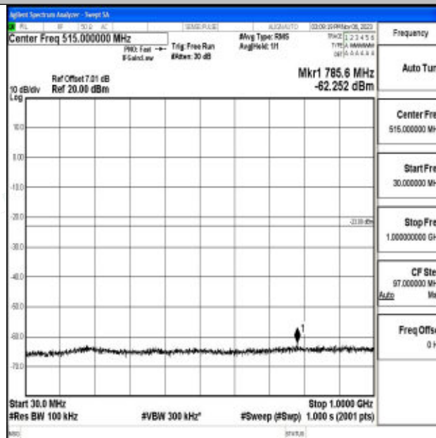
Band2_1.4MHz_64QAM_18607_1RB#0_30~1000_30~1000
