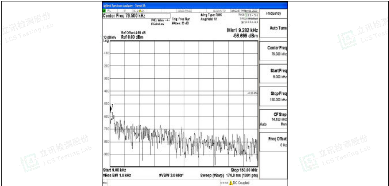
Band2_5MHz_16QAM_18625_1RB#0_0.009~0.15_0.009~0.15
