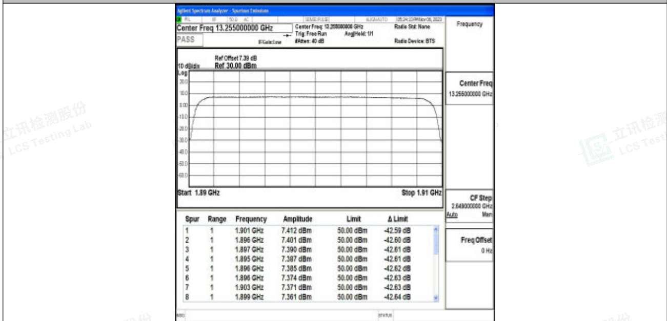
Band2_20MHz_QPSK_19100_100RB#0
