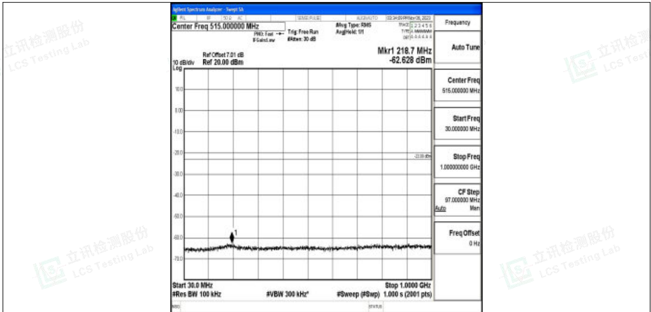
Band2_3MHz_64QAM_18615_1RB#0_30~1000_30~1000
