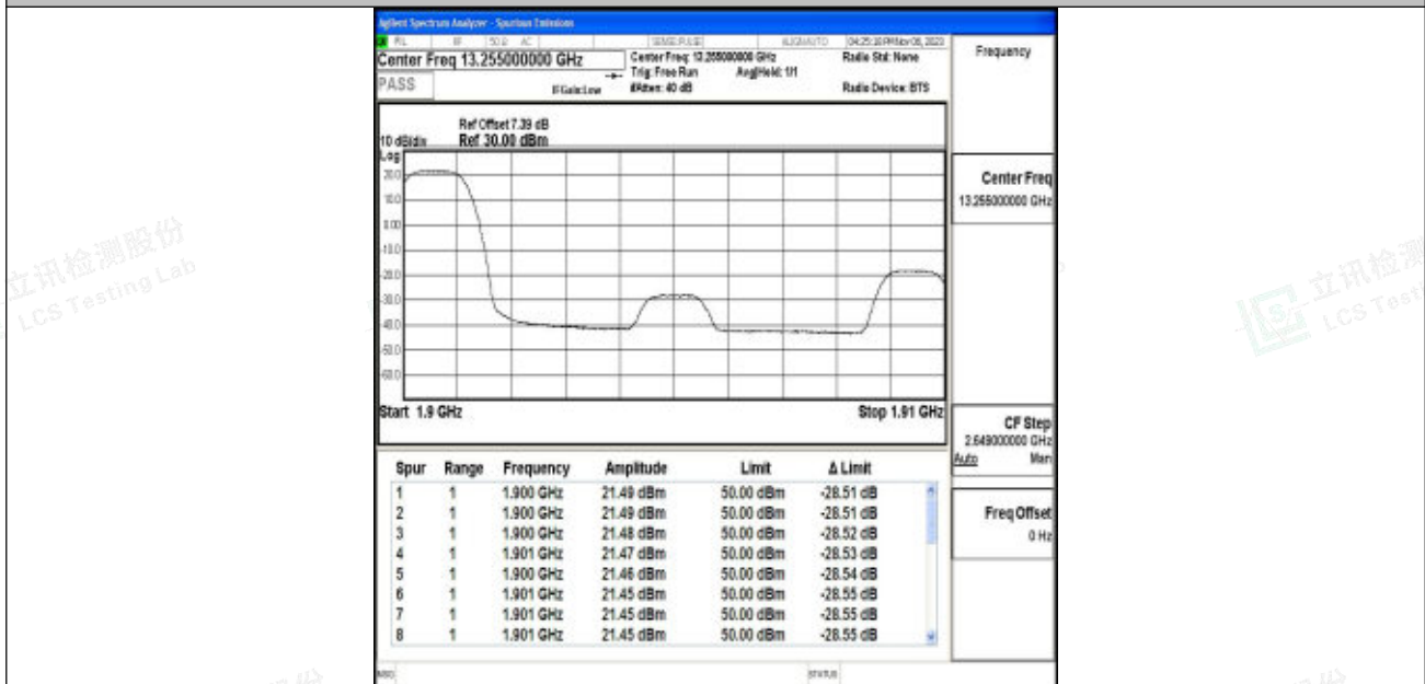
Band2_10MHz_QPSK_19150_1RB#0
