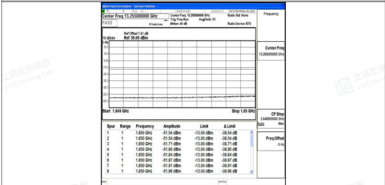
Band2_15MHz_QPSK_18675_1RB#74
