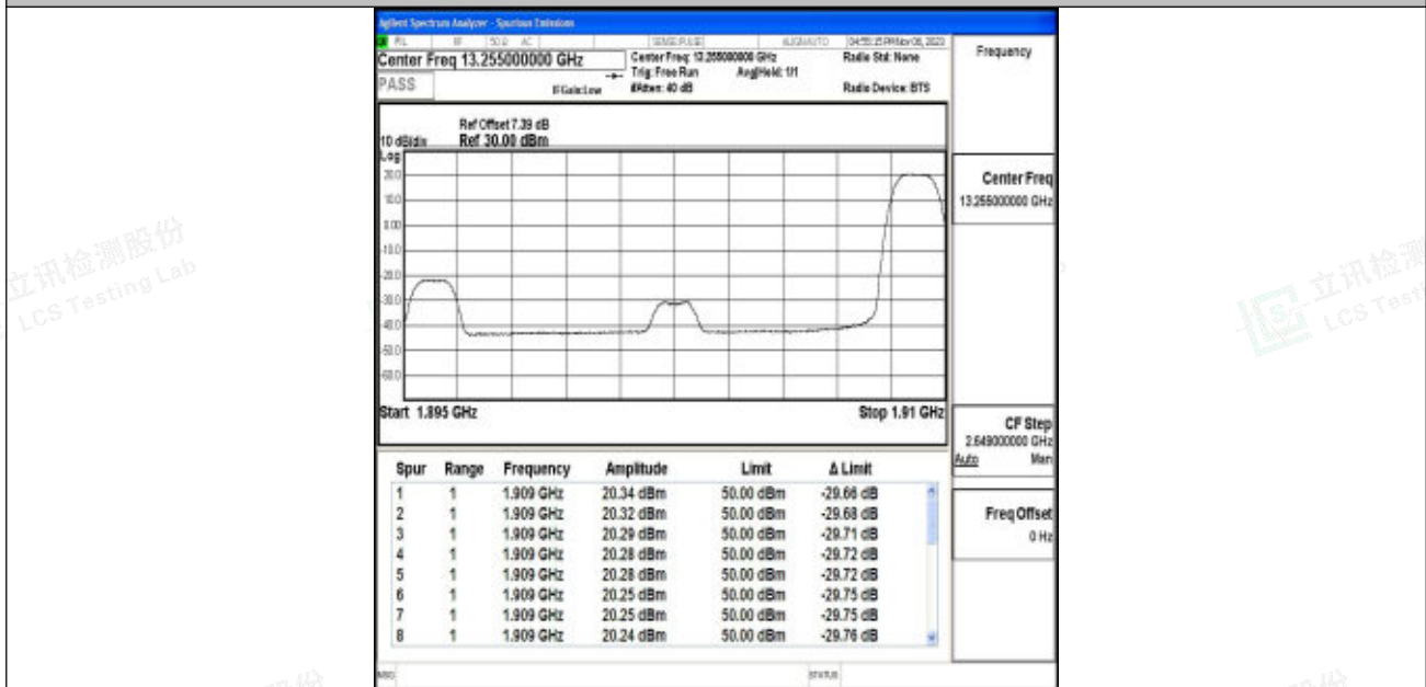
Band2_15MHz_16QAM_19125_1RB#74
