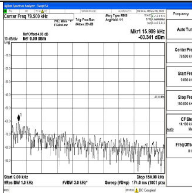
Band2_3MHz_QPSK_18900_1RB#0_0.009~0.15_0.009~0.15
