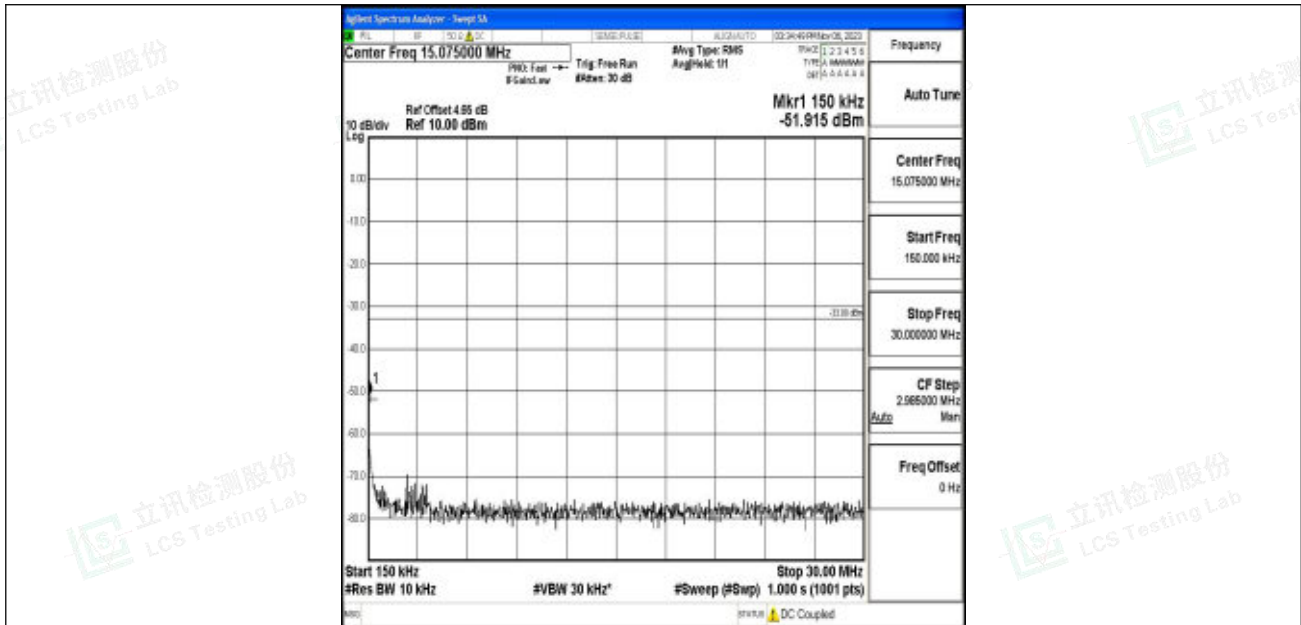
Band2_3MHz_QPSK_18900_1RB#0_0.15~30_0.15~30
