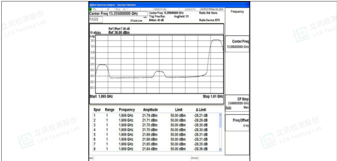
Band2_15MHz_QPSK_19125_1RB#74
