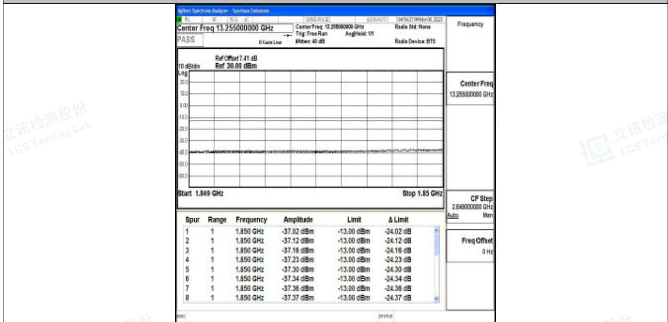
Band2_15MHz_16QAM_18675_75RB#0
