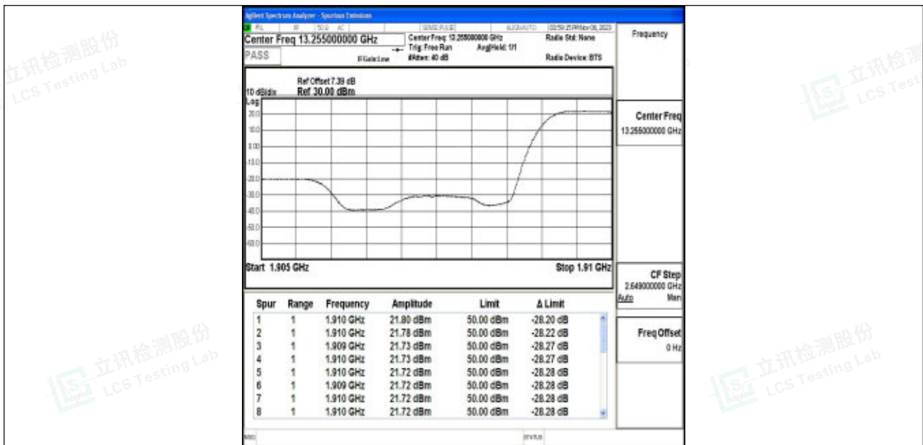
Band2_5MHz_QPSK_19175_1RB#24
