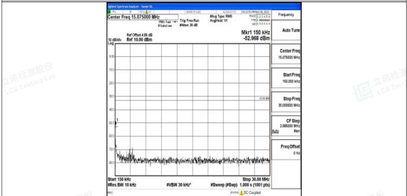
Band2_1.4MHz_16QAM_19193_1RB#0_0.15~30_0.15~30
