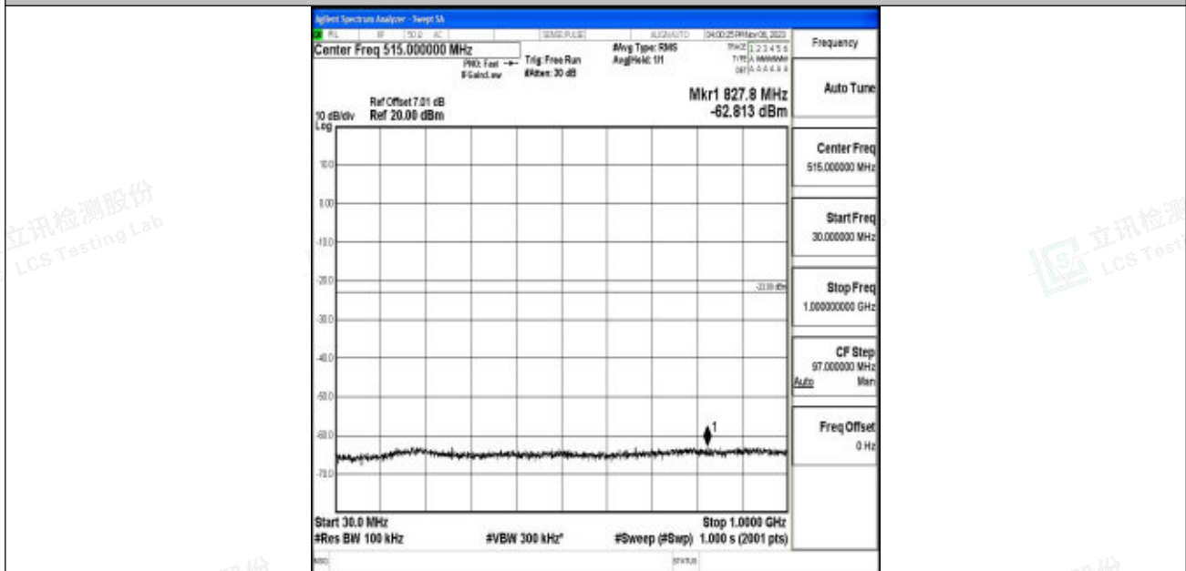
Band2_5MHz_QPSK_18625_1RB#0_30~1000_30~1000
