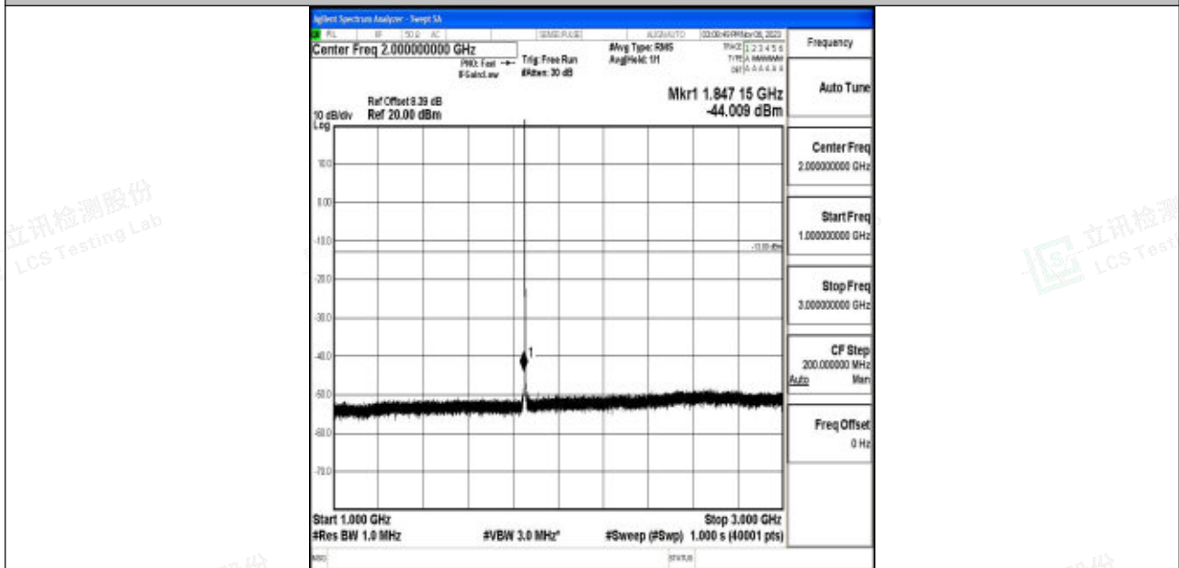
Band2_1.4MHz_16QAM_18607_1RB#0_1000~3000_1000~3000
