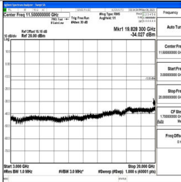
Band2_3MHz_64QAM_18615_1RB#0_3000~20000_3000~20000
