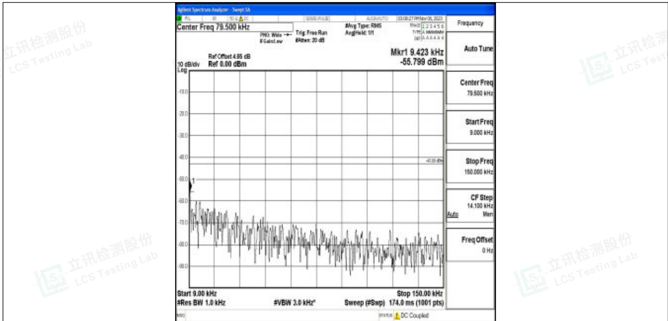
Band2_1.4MHz_16QAM_18607_1RB#0_0.009~0.15_0.009~0.15
