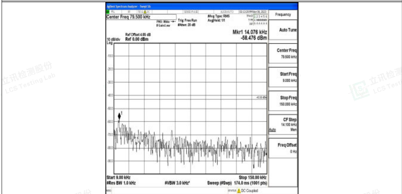
Band2_1.4MHz_64QAM_19193_1RB#0_0.009~0.15_0.009~0.15
