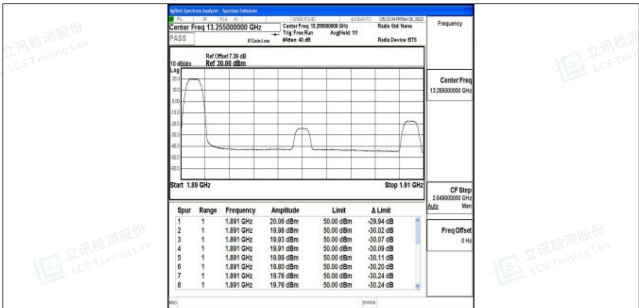
Band2_20MHz_16QAM_19100_1RB#0
