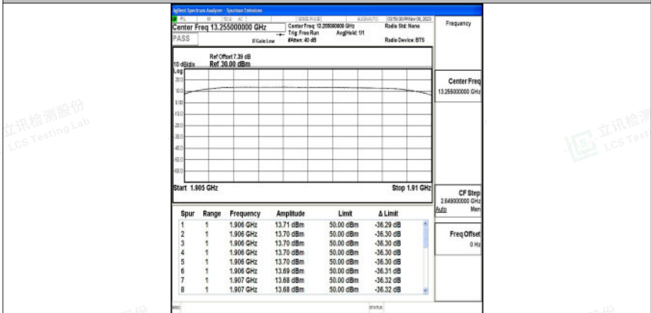
Band2_5MHz_QPSK_19175_25RB#0
