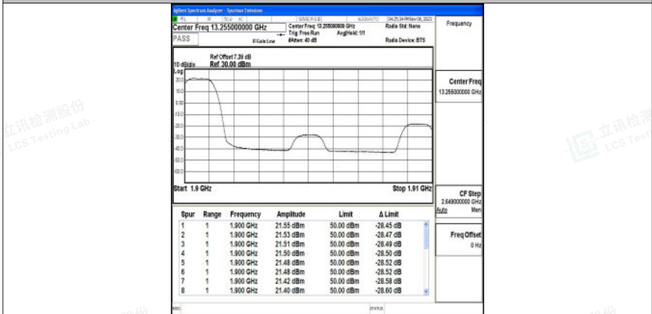
Band2_10MHz_64QAM_19150_1RB#0
