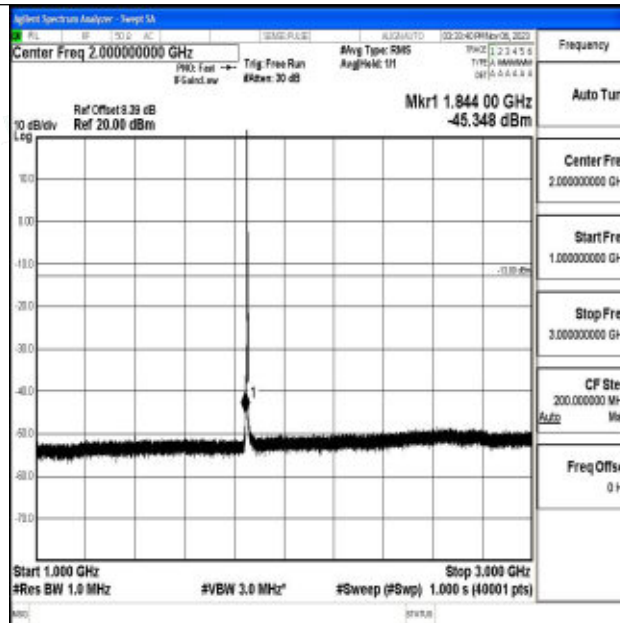
Band2_3MHz_16QAM_18615_1RB#0_1000~3000_1000~3000
