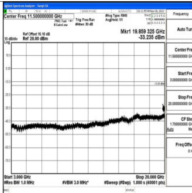
Band2_1.4MHz_64QAM_18900_1RB#0_3000~20000_3000~20000
