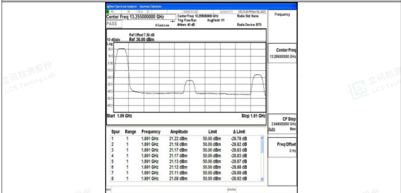
Band2_20MHz_QPSK_19100_1RB#0
