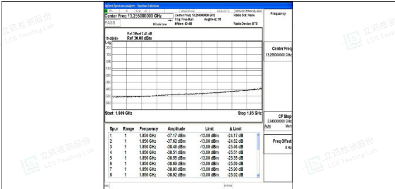
Band2_15MHz_64QAM_18675_1RB#0
