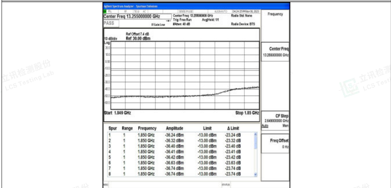
Band2_10MHz_16QAM_18650_1RB#0
