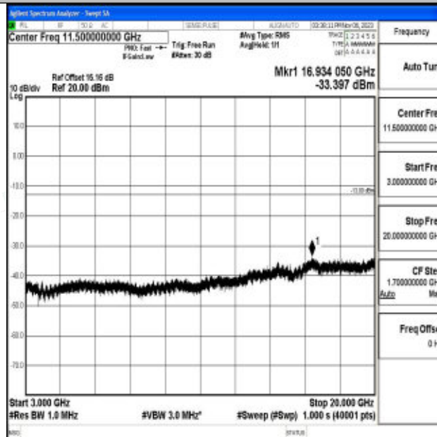
Band2_3MHz_16QAM_19185_1RB#0_3000~20000_3000~20000
