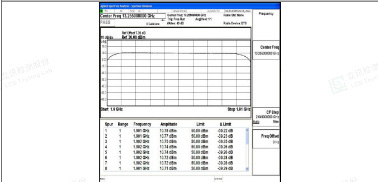
Band2_10MHz_64QAM_19150_50RB#0
