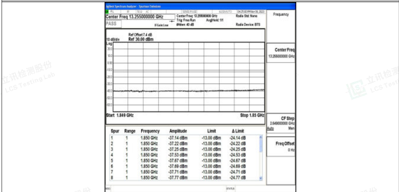
Band2_10MHz_16QAM_18650_50RB#0
