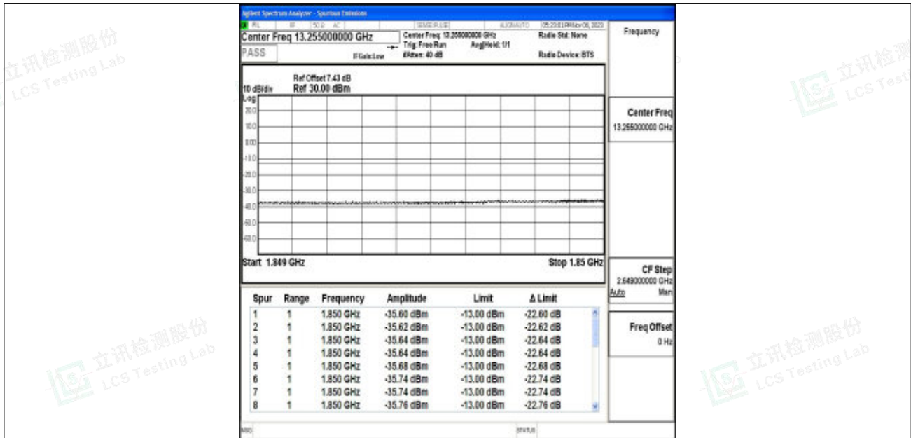
Band2_20MHz_QPSK_18700_100RB#0
