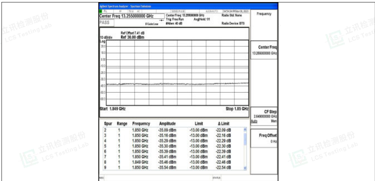
Band2_15MHz_64QAM_18675_75RB#0
