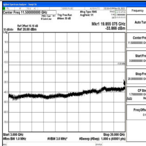
Band2_3MHz_64QAM_18900_1RB#0_3000~20000_3000~20000
