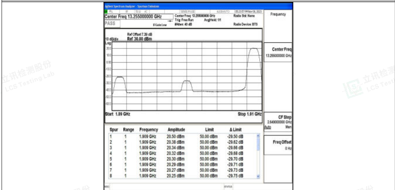
Band2_20MHz_16QAM_19100_1RB#99
