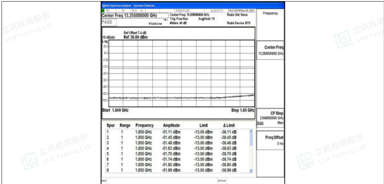
Band2_10MHz_16QAM_18650_1RB#49
