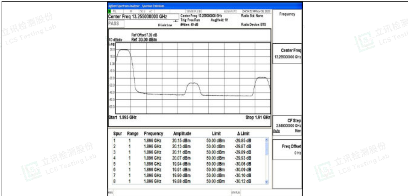
Band2_15MHz_16QAM_19125_1RB#0
