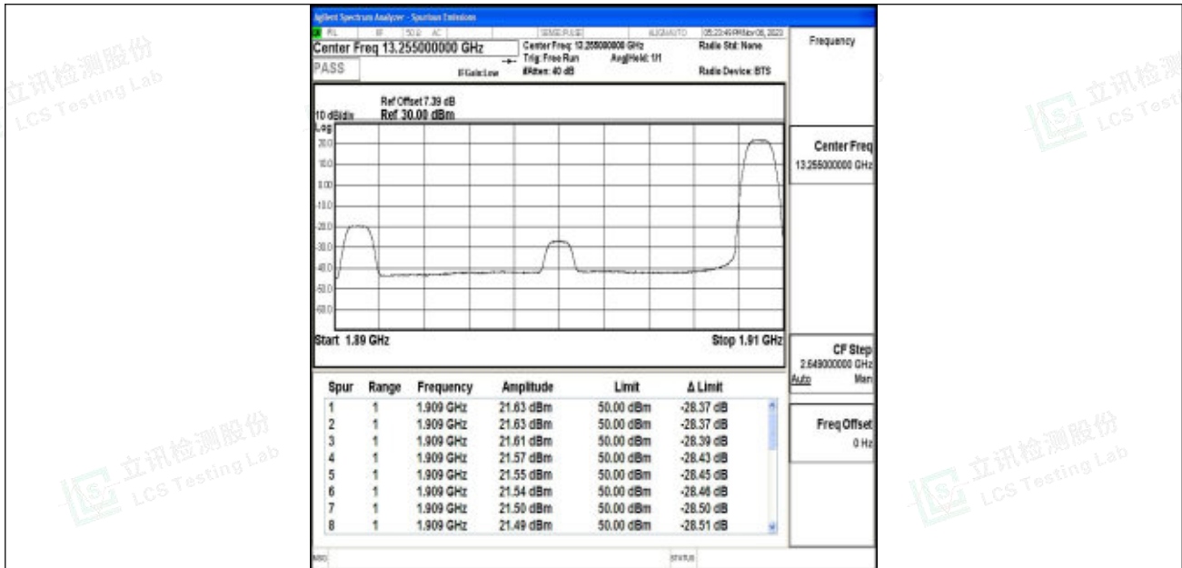
Band2_20MHz_QPSK_19100_1RB#99
