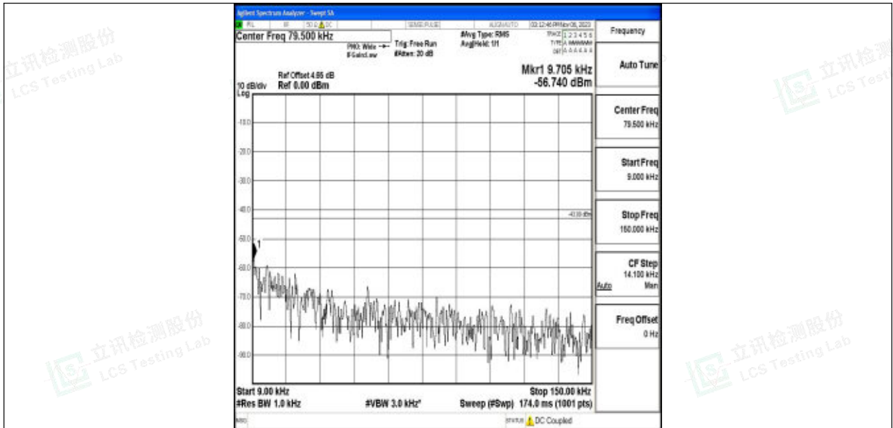
Band2_1.4MHz_16QAM_19193_1RB#0_0.009~0.15_0.009~0.15
