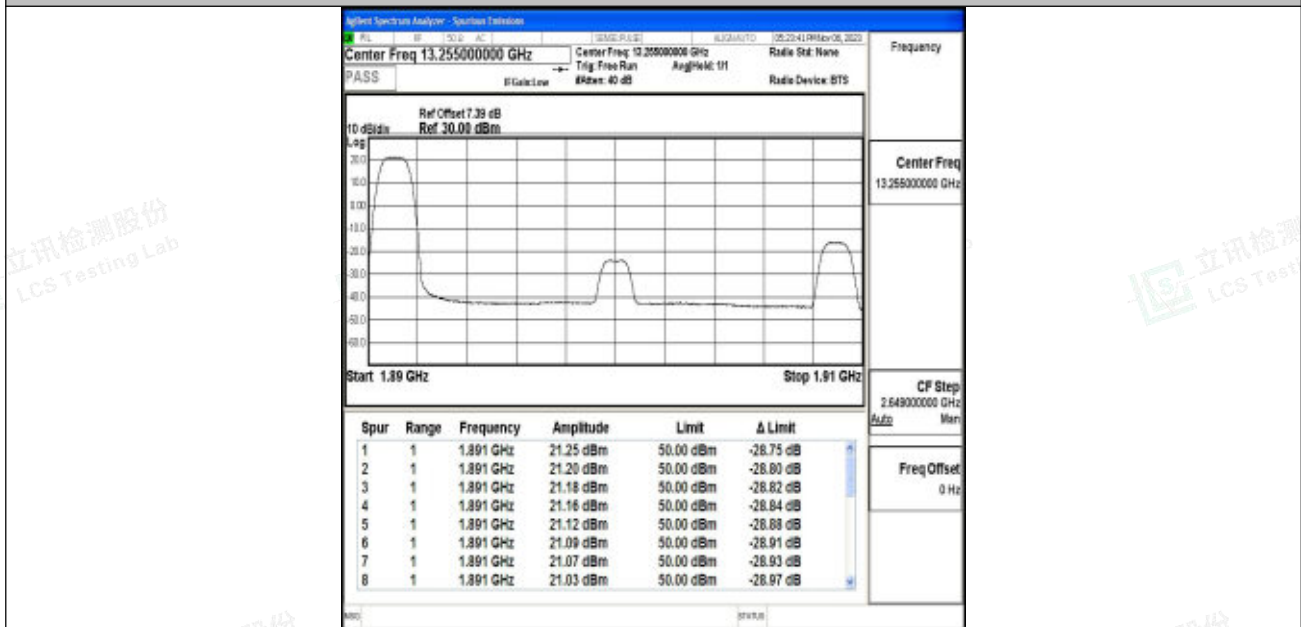
Band2_20MHz_64QAM_19100_1RB#0
