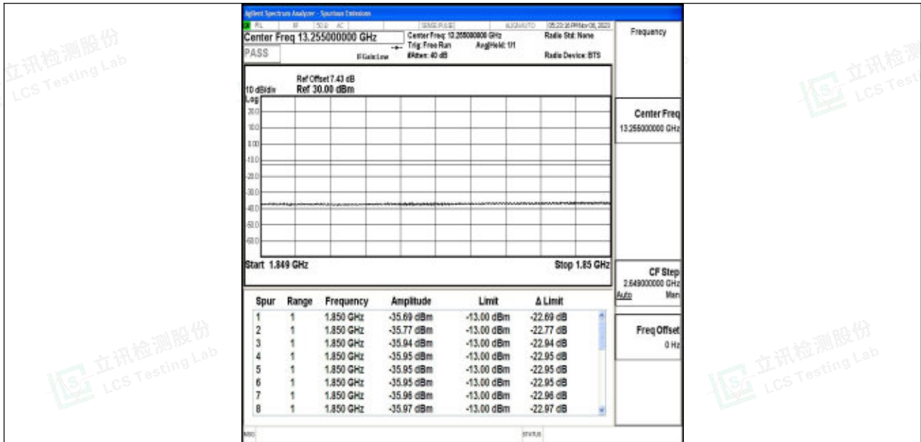
Band2_20MHz_64QAM_18700_100RB#0
