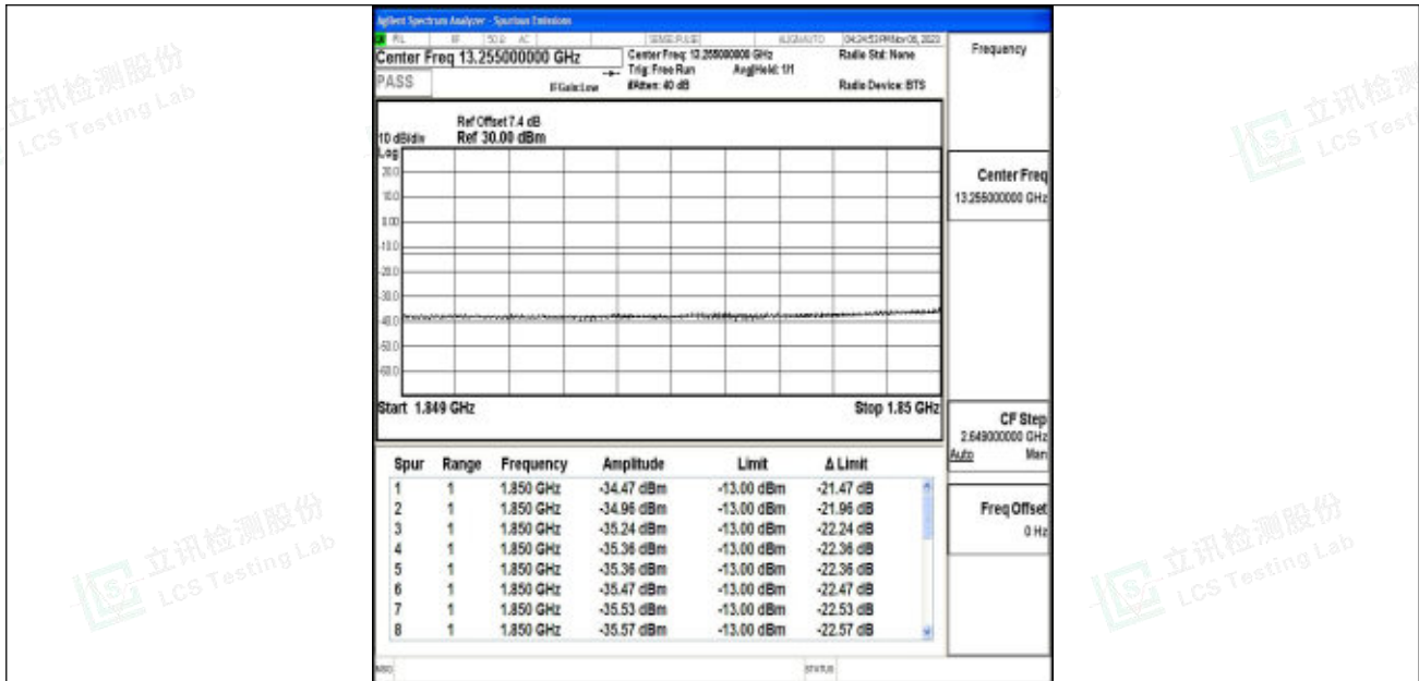
Band2_10MHz_QPSK_18650_50RB#0
