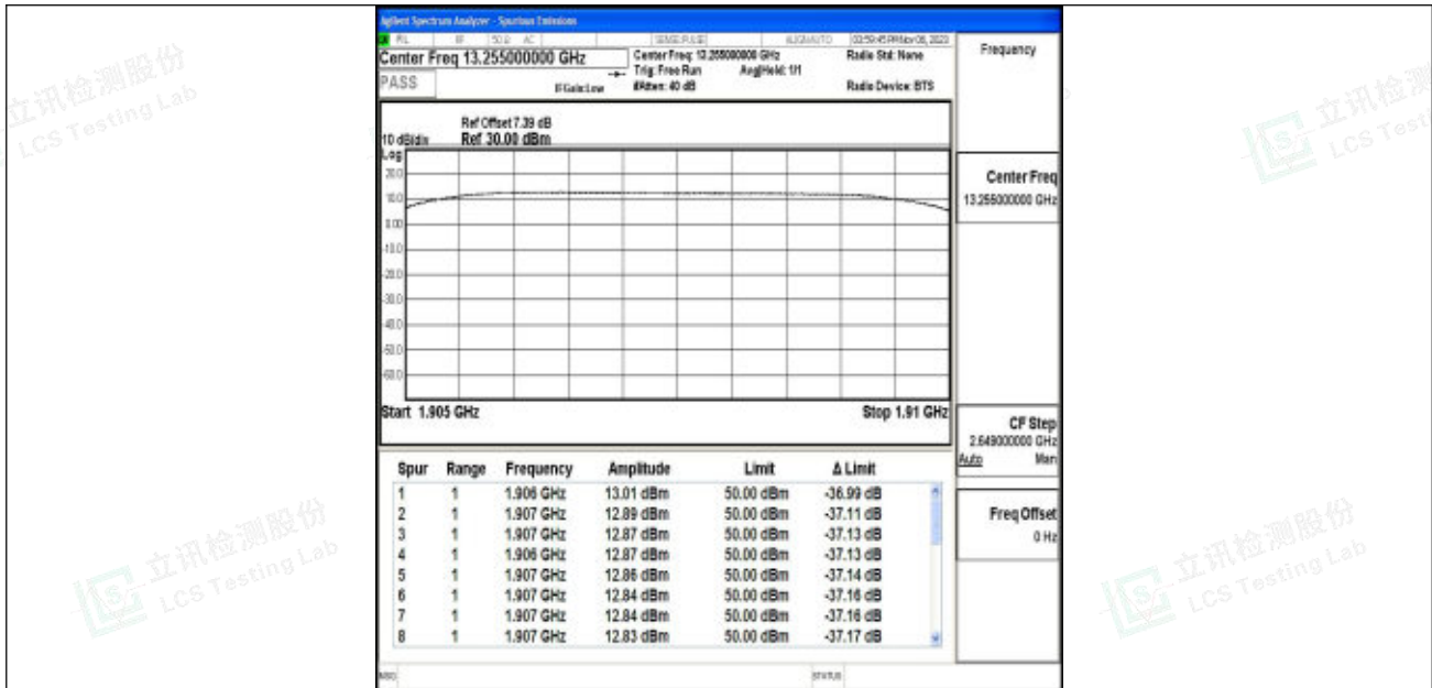
Band2_5MHz_16QAM_19175_25RB#0
