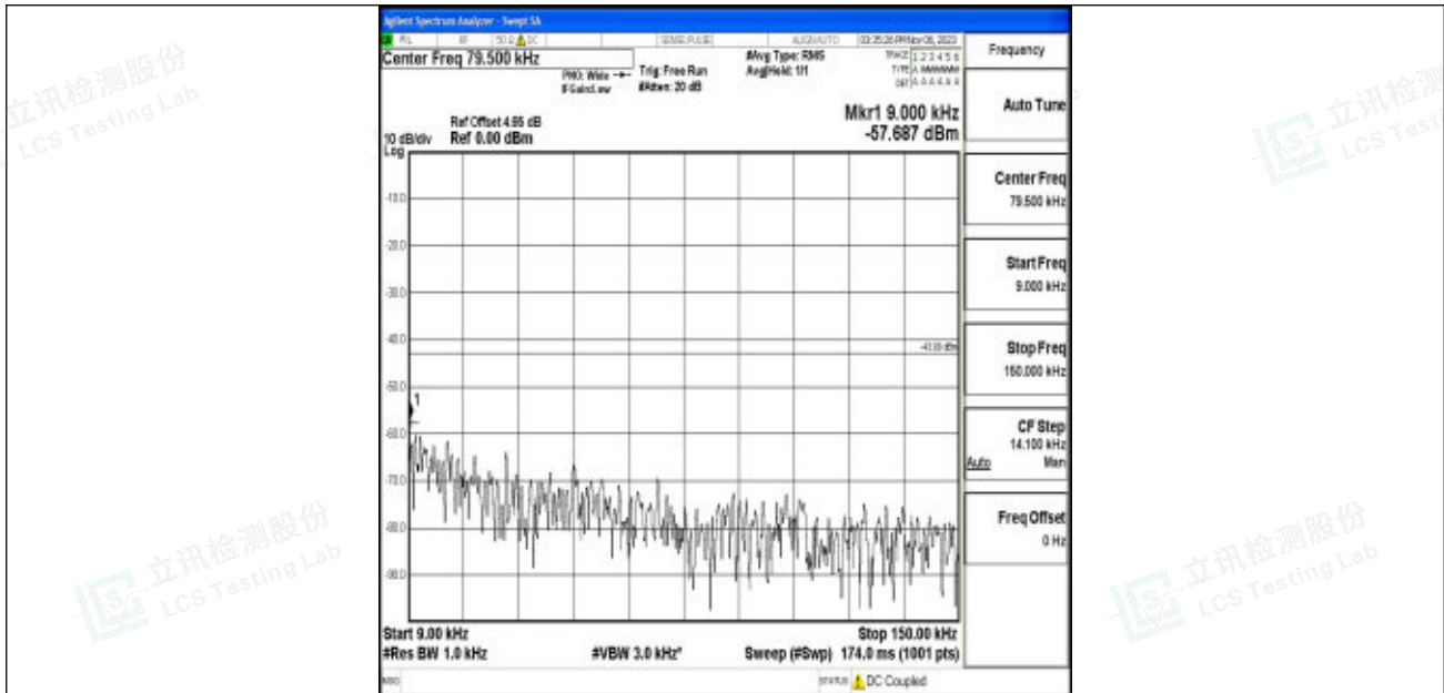
Band2_3MHz_16QAM_18900_1RB#0_0.009~0.15_0.009~0.15
