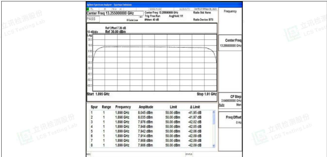
Band2_15MHz_16QAM_19125_75RB#0
