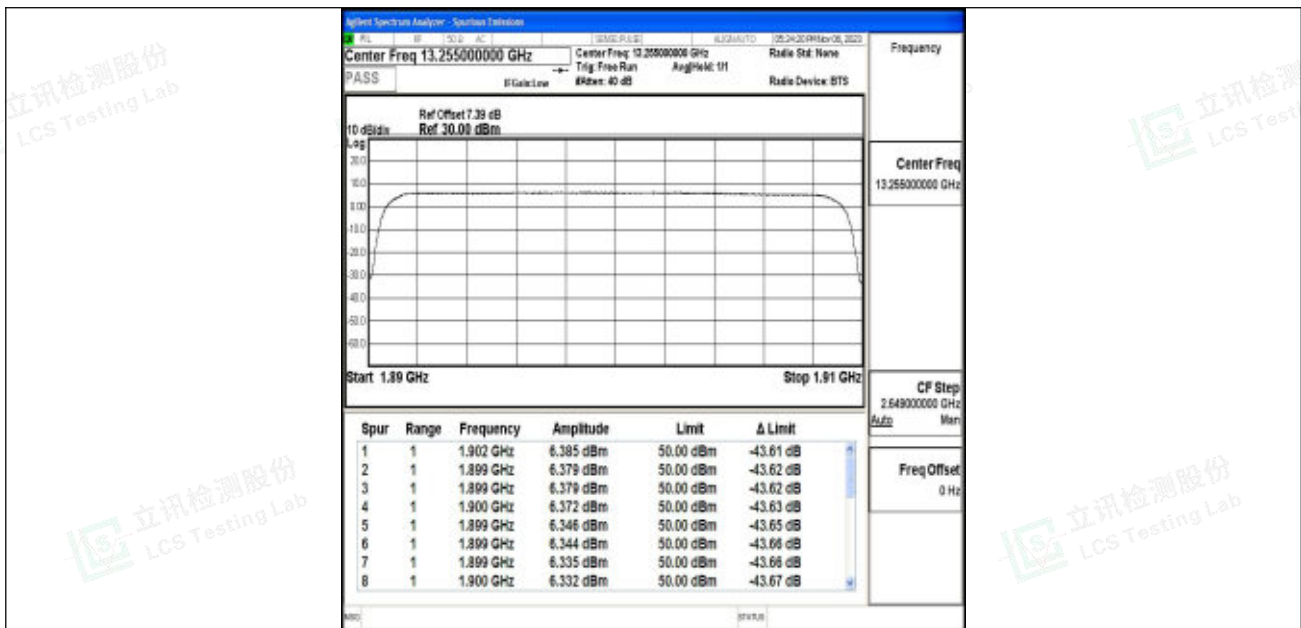
Band2_20MHz_16QAM_19100_100RB#0
