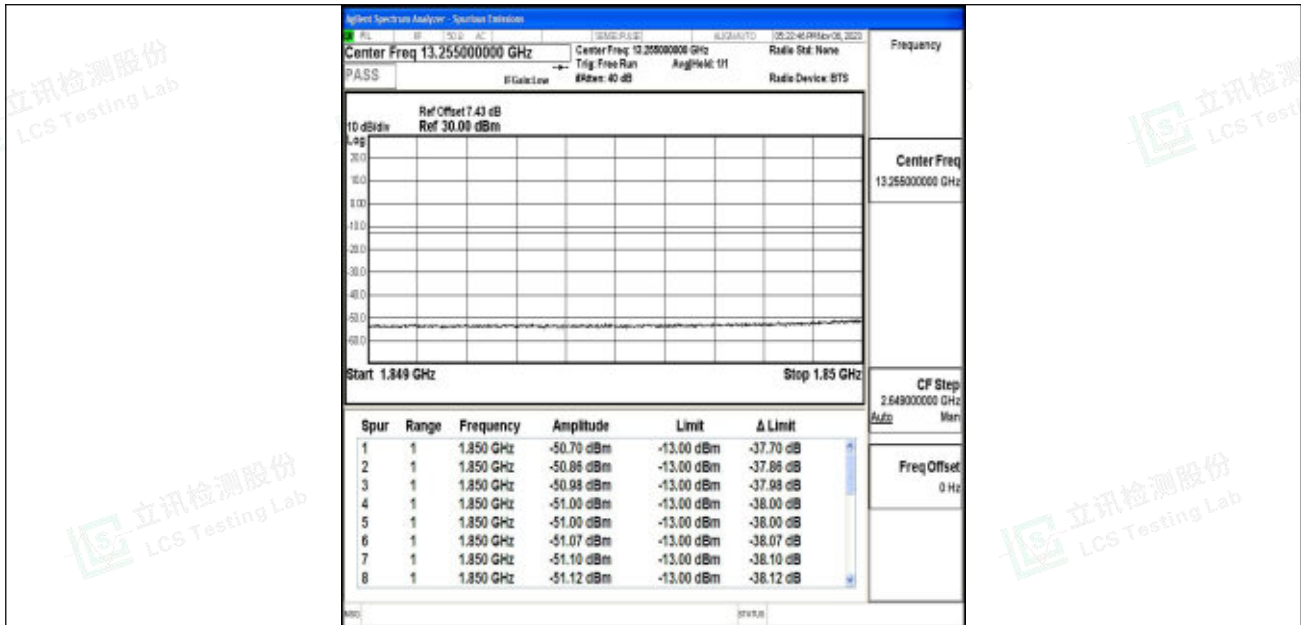
Band2_20MHz_16QAM_18700_1RB#99
