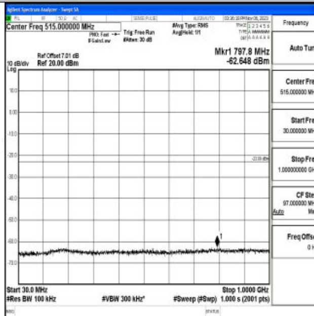
Band2_3MHz_64QAM_18900_1RB#0_30~1000_30~1000
