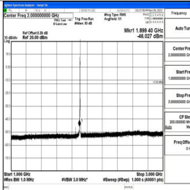
Band2_3MHz_16QAM_19185_1RB#0_1000~3000_1000~3000
