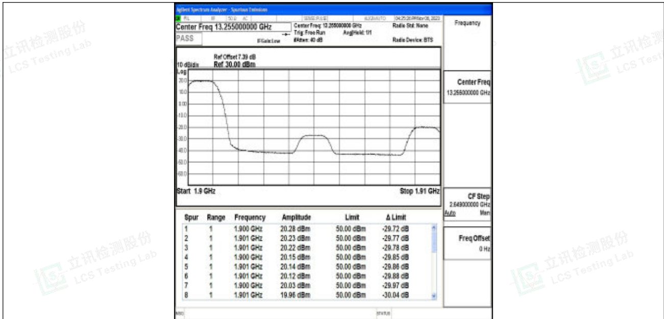
Band2_10MHz_16QAM_19150_1RB#0
