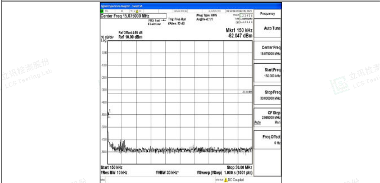
Band2_3MHz_64QAM_18615_1RB#0_0.15~30_0.15~30
