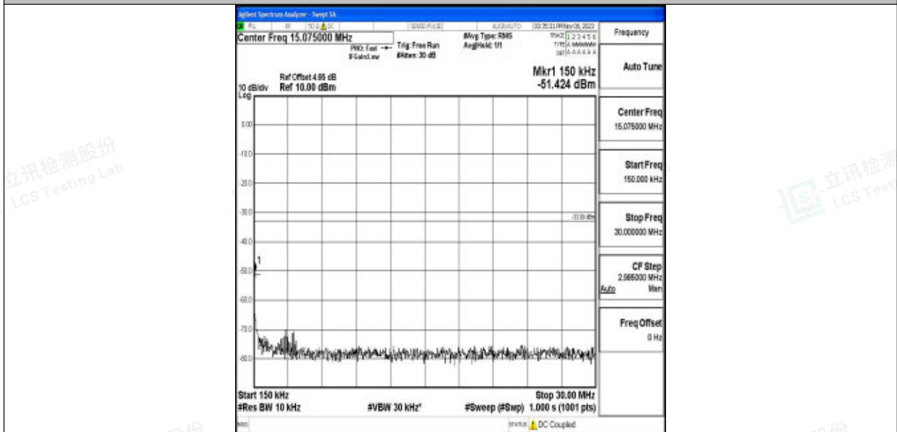
Band2_3MHz_16QAM_18900_1RB#0_0.15~30_0.15~30
