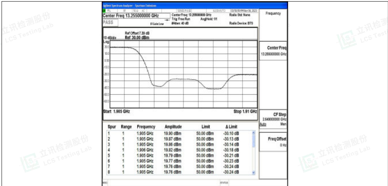
Band2_5MHz_16QAM_19175_1RB#0
