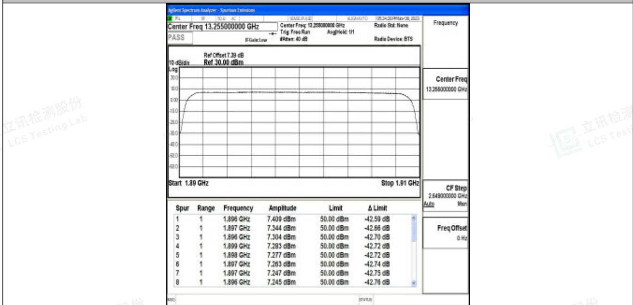
Band2_20MHz_64QAM_19100_100RB#0
