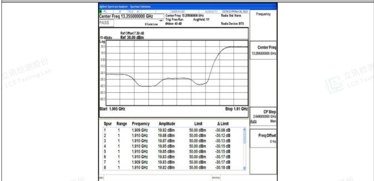
Band2_5MHz_16QAM_19175_1RB#24
