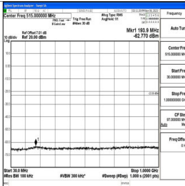
Band2_1.4MHz_64QAM_18900_1RB#0_30~1000_30~1000
