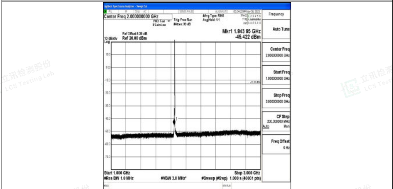
Band2_3MHz_64QAM_18615_1RB#0_1000~3000_1000~3000
