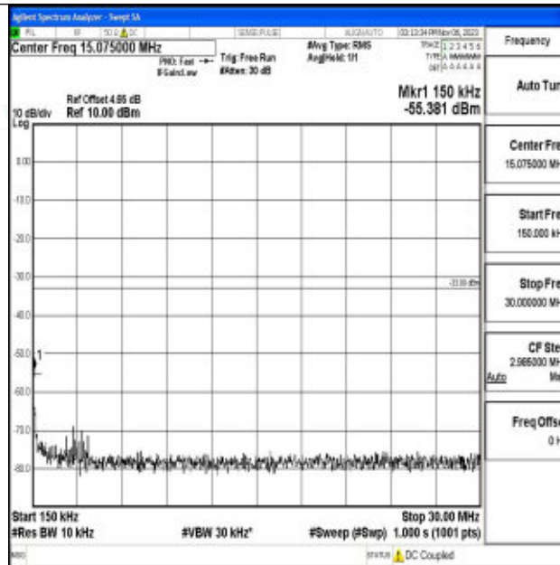
Band2_1.4MHz_64QAM_19193_1RB#0_0.15~30_0.15~30
