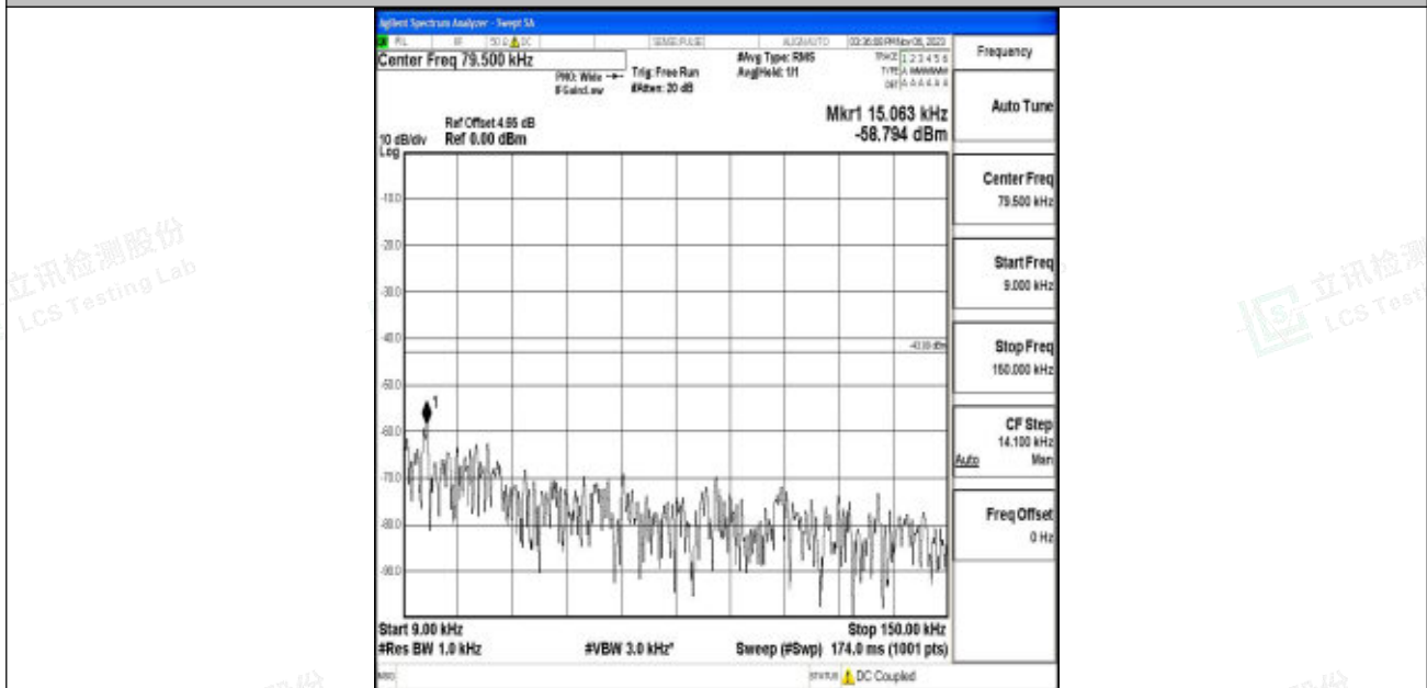
Band2_3MHz_64QAM_18900_1RB#0_0.009~0.15_0.009~0.15
