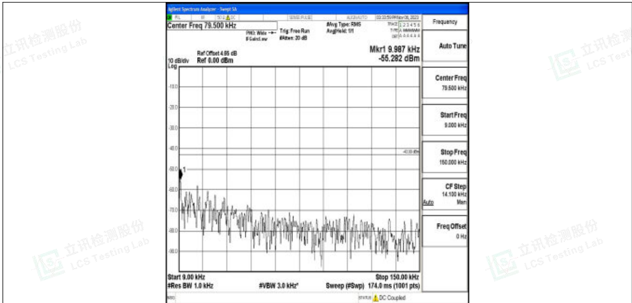
Band2_3MHz_64QAM_18615_1RB#0_0.009~0.15_0.009~0.15
