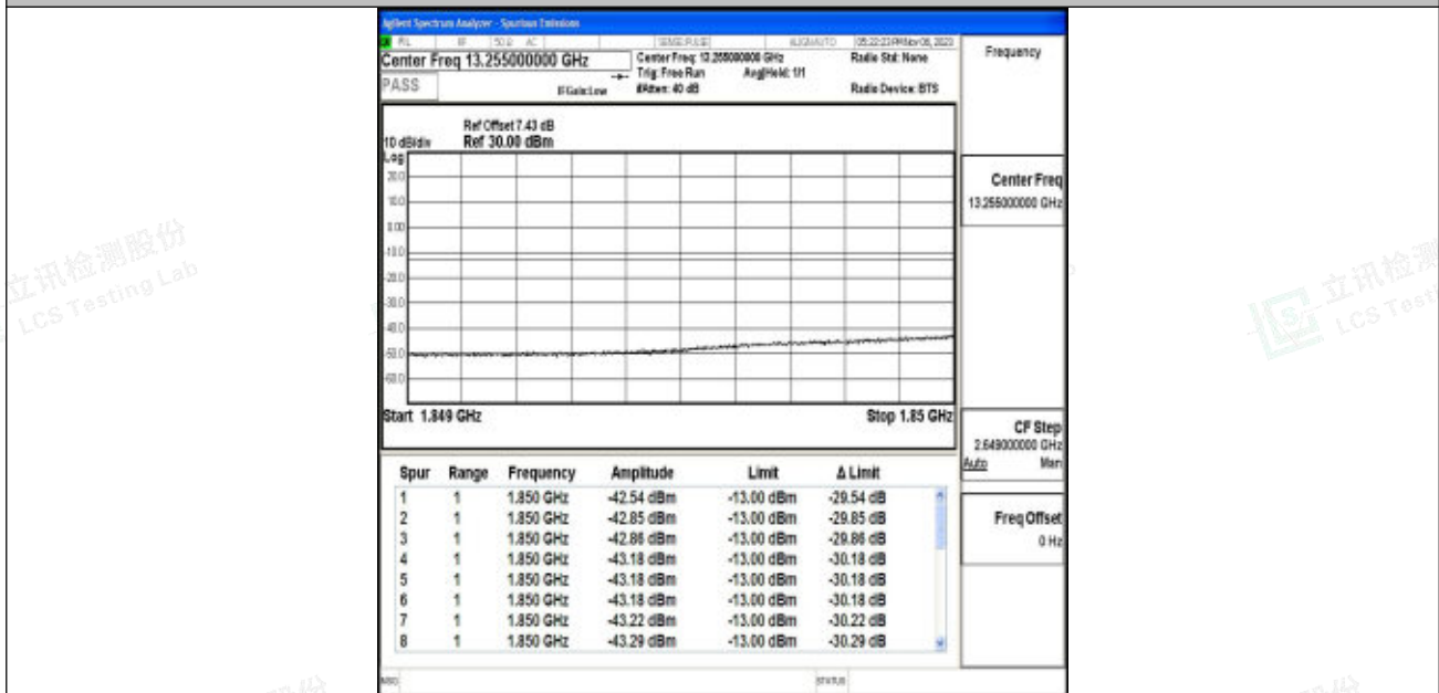
Band2_20MHz_16QAM_18700_1RB#0
