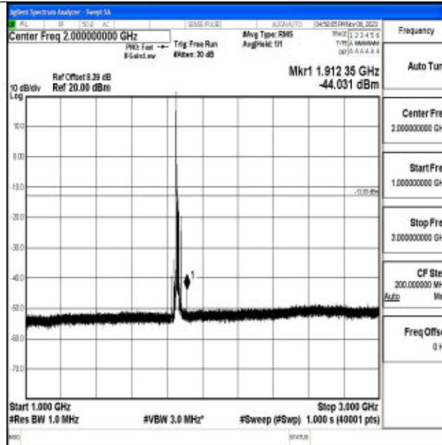
Band2_15MHz_64QAM_18675_1RB#0_1000~3000_1000~3000
