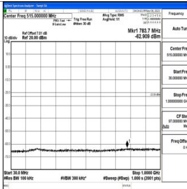
Band2_5MHz_64QAM_18900_1RB#0_30~1000_30~1000
