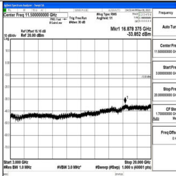
Band2_5MHz_16QAM_18900_1RB#0_3000~20000_3000~20000
