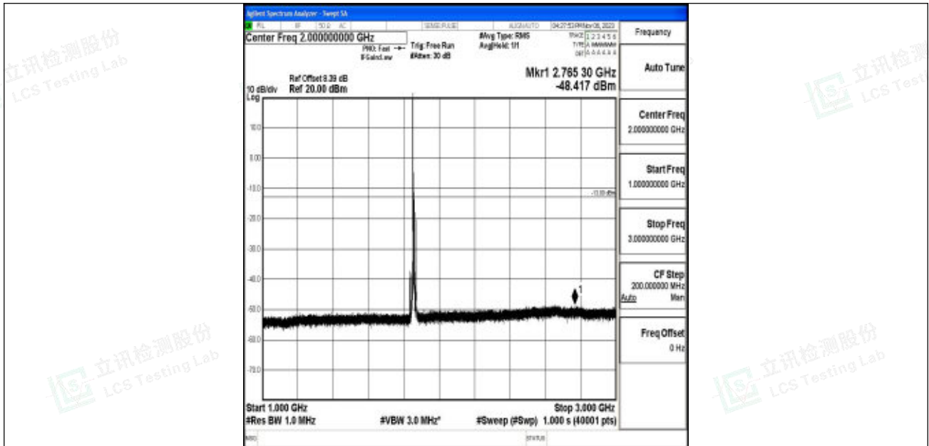
Band2_10MHz_16QAM_18650_1RB#0_1000~3000_1000~3000
