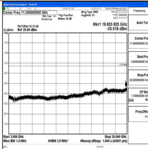
Band2_15MHz_64QAM_18675_1RB#0_3000~20000_3000~20000
