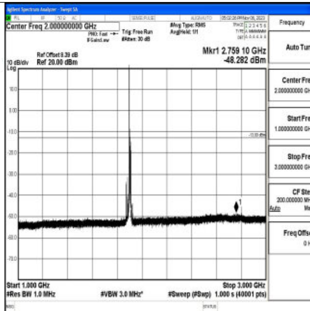
Band2_15MHz_64QAM_19125_1RB#0_1000~3000_1000~3000
