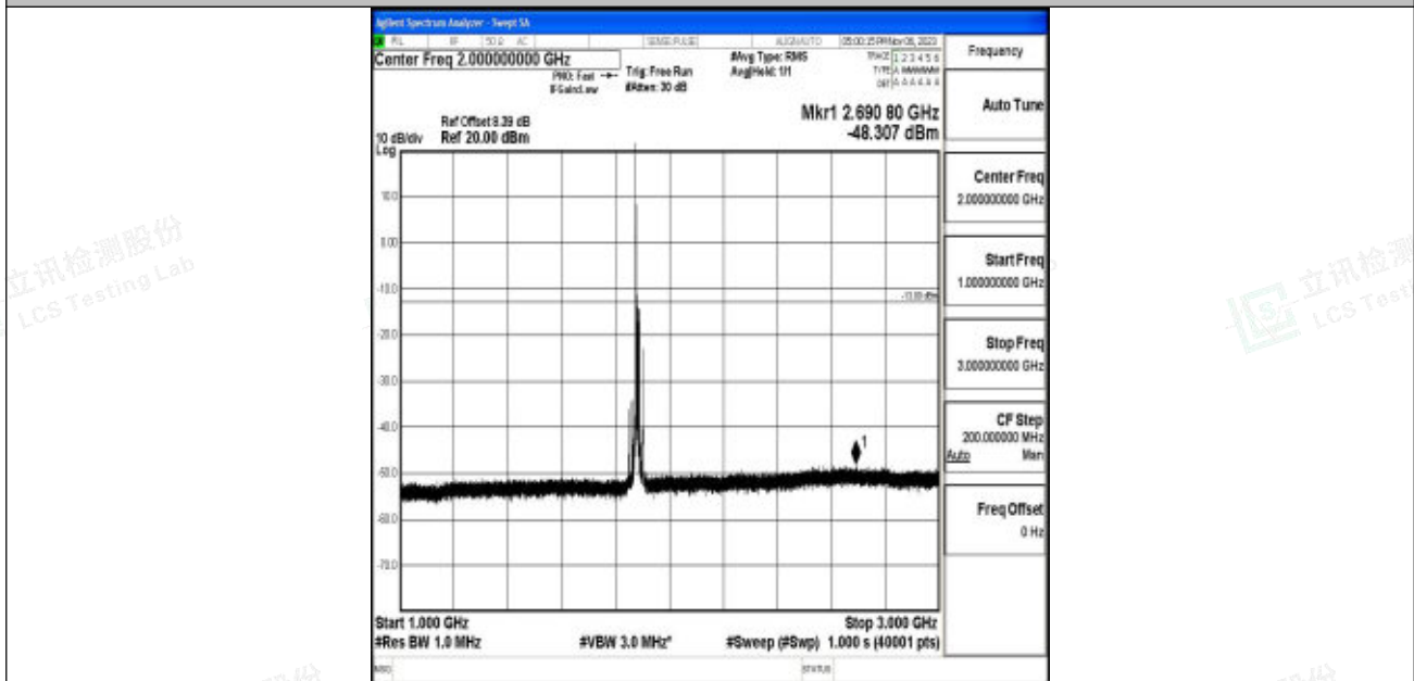
Band2_15MHz_64QAM_18900_1RB#0_1000~3000_1000~3000
