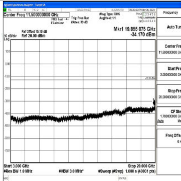
Band2_20MHz_16QAM_18900_1RB#0_3000~20000_3000~20000
