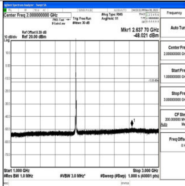
Band2_5MHz_16QAM_18900_1RB#0_1000~3000_1000~3000
