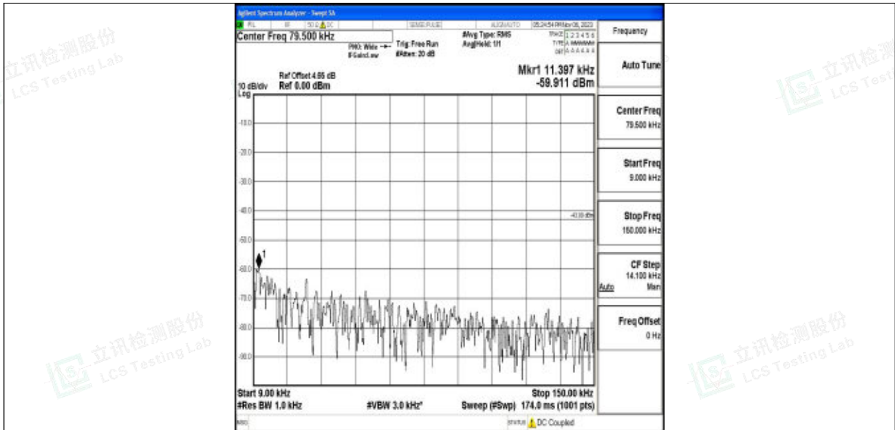
Band2_20MHz_QPSK_18700_1RB#0_0.009~0.15_0.009~0.15
