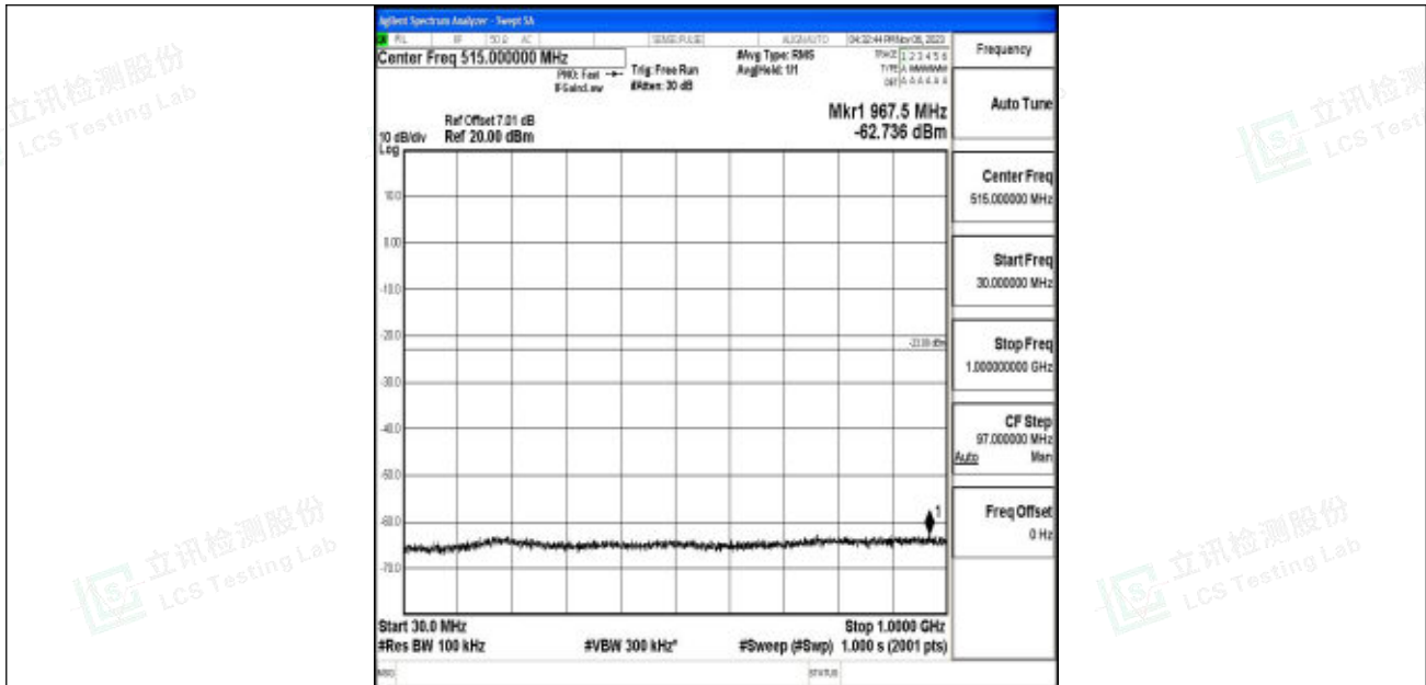
Band2_10MHz_64QAM_19150_1RB#0_30~1000_30~1000
