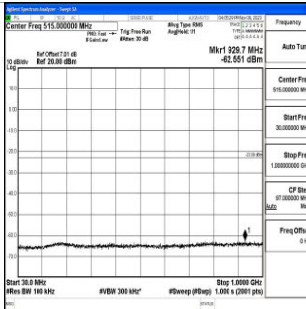
Band2_5MHz_16QAM_19175_1RB#0_30~1000_30~1000
