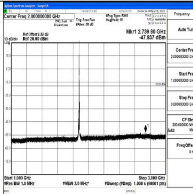
Band2_5MHz_64QAM_18900_1RB#0_1000~3000_1000~3000
