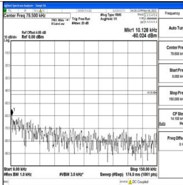
Band2_10MHz_64QAM_18650_1RB#0_0.009~0.15_0.009~0.15
