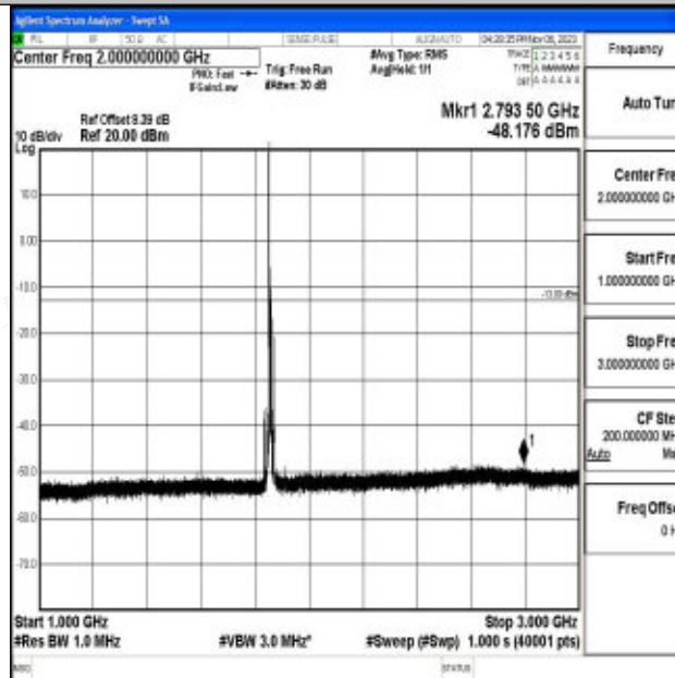
Band2_10MHz_64QAM_18650_1RB#0_1000~3000_1000~3000
