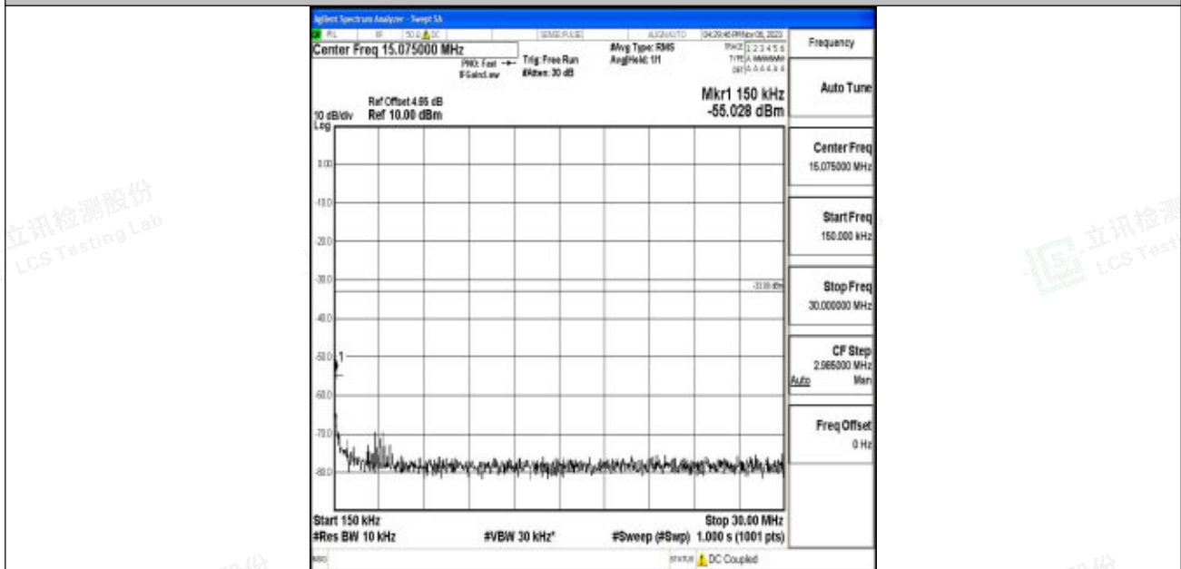
Band2_10MHz_16QAM_18900_1RB#0_0.15~30_0.15~30
