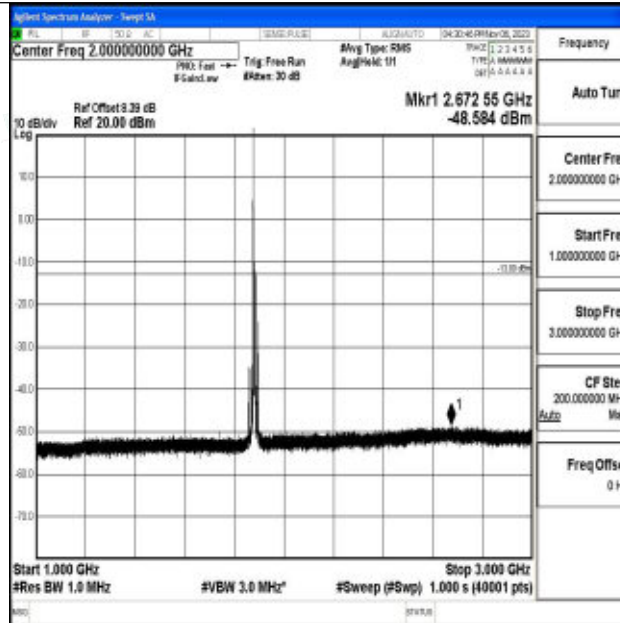
Band2_10MHz_64QAM_18900_1RB#0_1000~3000_1000~3000
