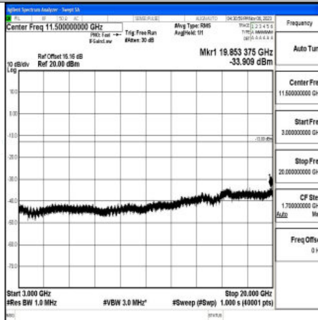
Band2_10MHz_64QAM_18900_1RB#0_3000~20000_3000~20000
