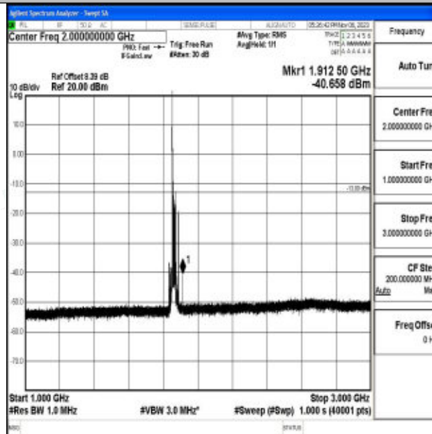
Band2_20MHz_64QAM_18700_1RB#0_1000~3000_1000~3000
