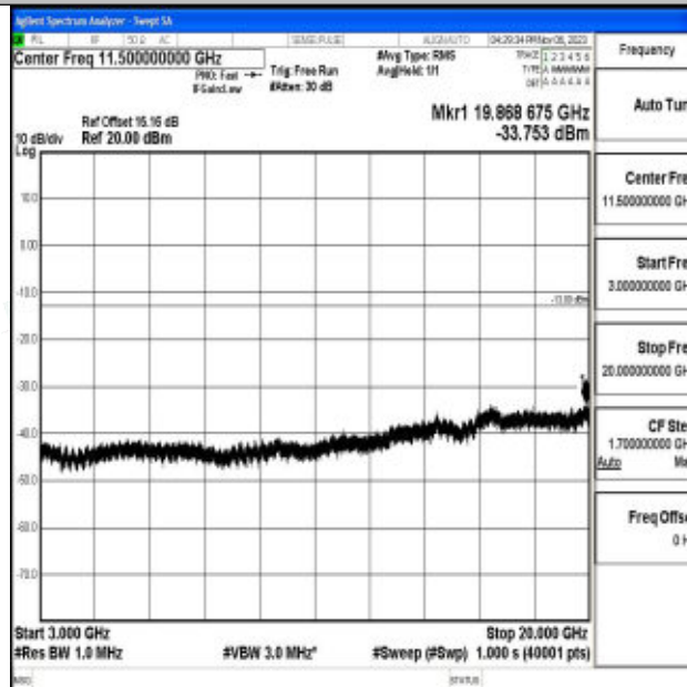
Band2_10MHz_QPSK_18900_1RB#0_3000~20000_3000~20000
