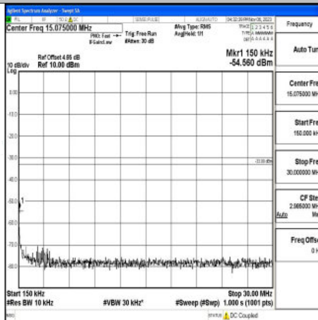
Band2_10MHz_64QAM_19150_1RB#0_0.15~30_0.15~30
