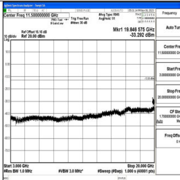
Band2_15MHz_QPSK_19125_1RB#0_3000~20000_3000~20000
