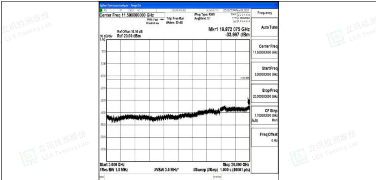
Band2_20MHz_64QAM_18700_1RB#0_3000~20000_3000~20000
