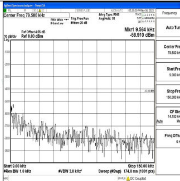
Band2_20MHz_64QAM_18900_1RB#0_0.009~0.15_0.009~0.15
