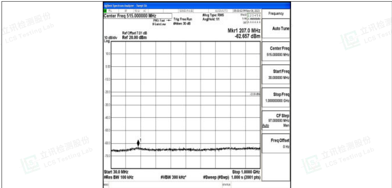
Band2_15MHz_64QAM_18900_1RB#0_30~1000_30~1000
