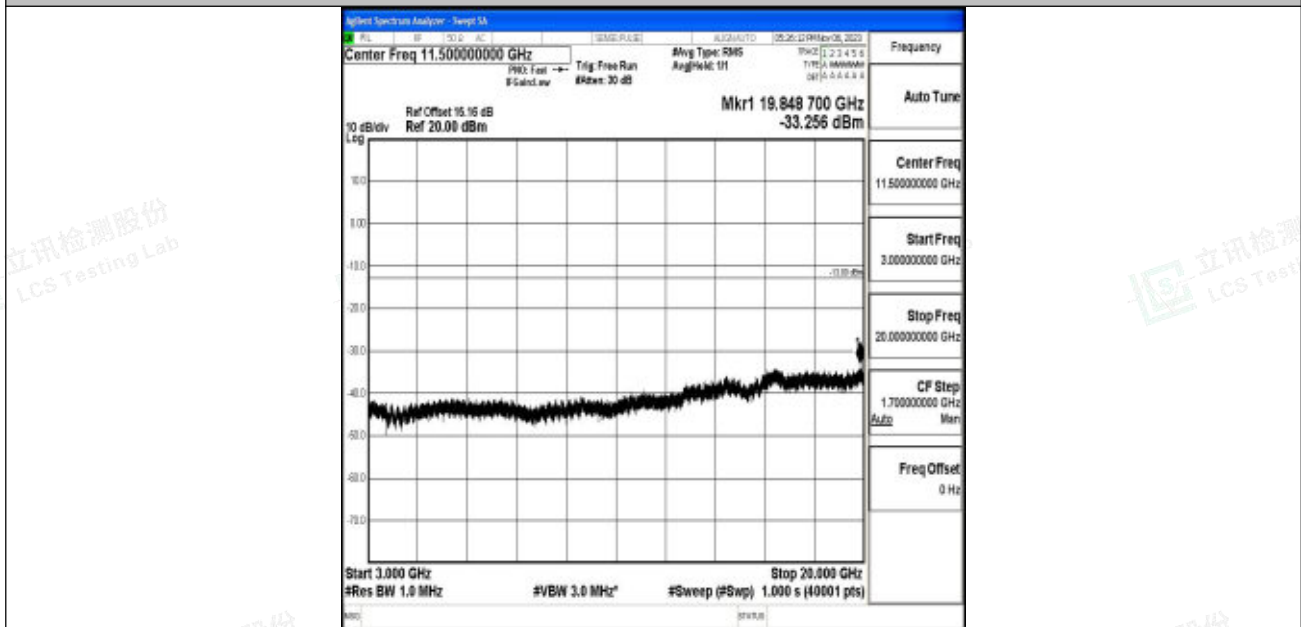
Band2_20MHz_16QAM_18700_1RB#0_3000~20000_3000~20000
