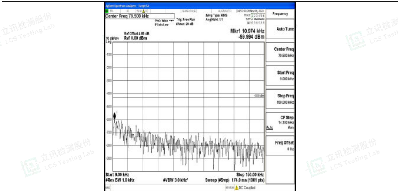
Band2_15MHz_16QAM_18675_1RB#0_0.009~0.15_0.009~0.15
