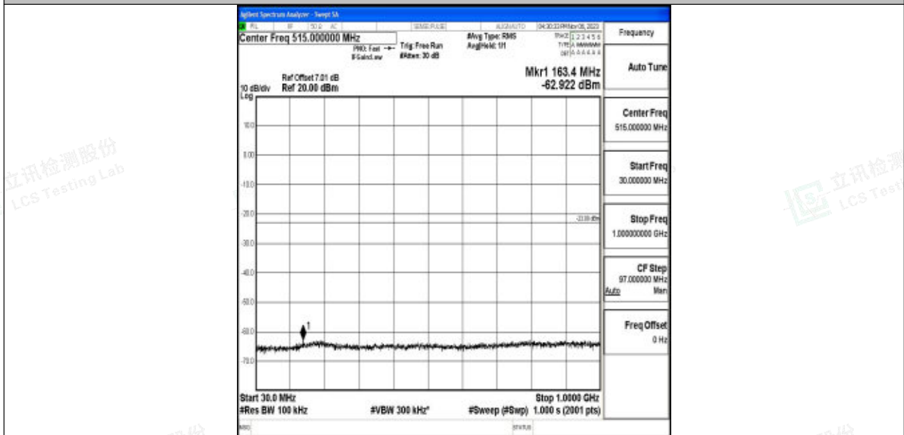
Band2_10MHz_64QAM_18900_1RB#0_30~1000_30~1000
