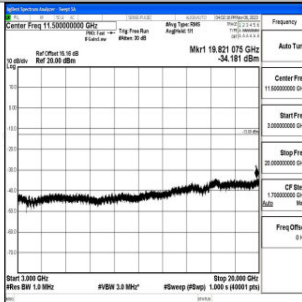
Band2_5MHz_64QAM_18625_1RB#0_3000~20000_3000~20000
