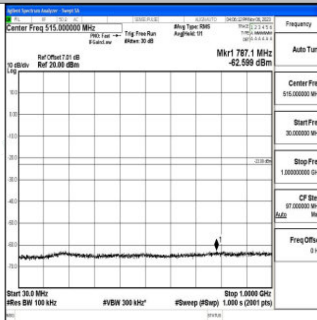
Band2_5MHz_64QAM_19175_1RB#0_30~1000_30~1000
