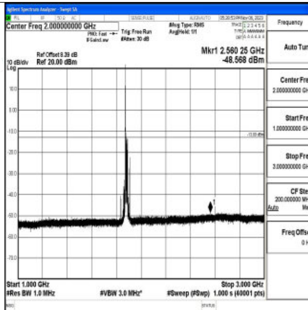
Band2_20MHz_64QAM_18900_1RB#0_1000~3000_1000~3000
