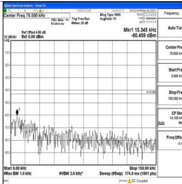
Band2_10MHz_64QAM_19150_1RB#0_0.009~0.15_0.009~0.15
