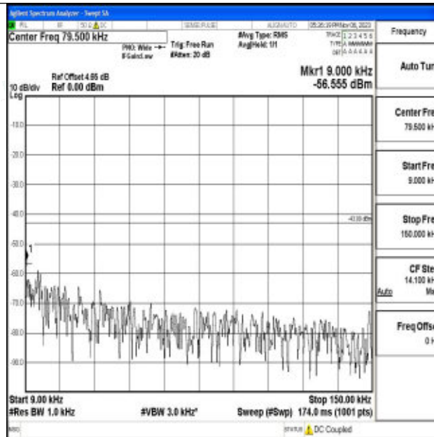
Band2_20MHz_64QAM_18700_1RB#0_0.009~0.15_0.009~0.15
