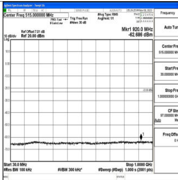
Band2_20MHz_QPSK_19100_1RB#0_30~1000_30~1000
