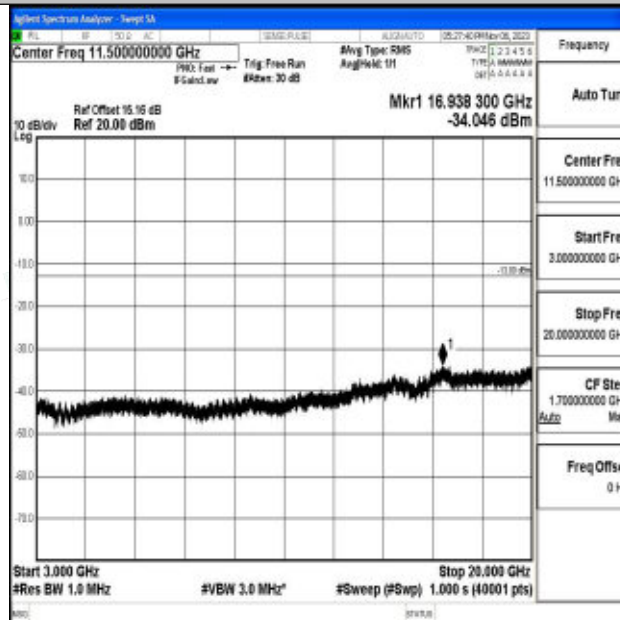
Band2_20MHz_QPSK_18900_1RB#0_3000~20000_3000~20000
