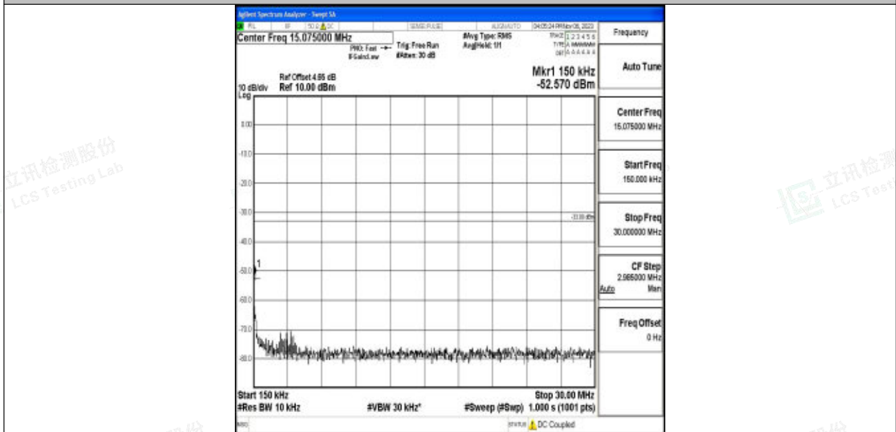
Band2_5MHz_16QAM_19175_1RB#0_0.15~30_0.15~30
