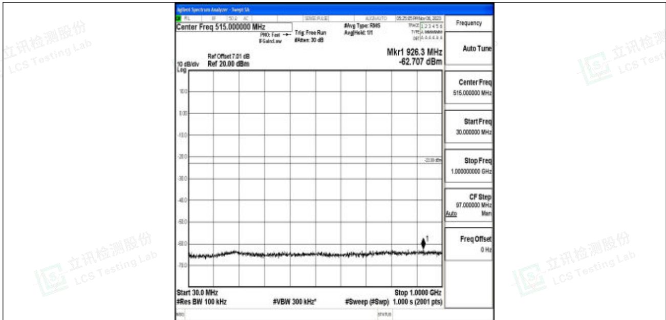
Band2_20MHz_QPSK_18700_1RB#0_30~1000_30~1000
