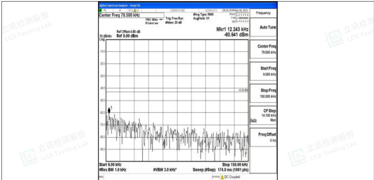
Band2_20MHz_QPSK_19100_1RB#0_0.009~0.15_0.009~0.15
