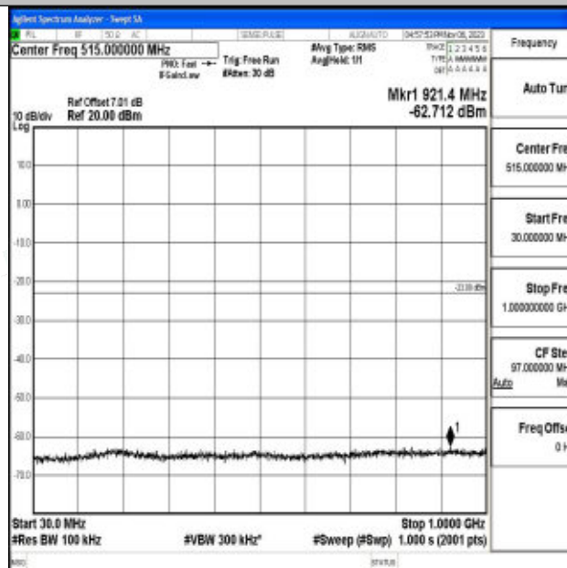
Band2_15MHz_64QAM_18675_1RB#0_30~1000_30~1000
