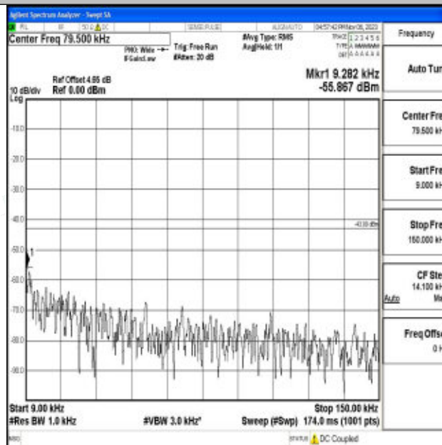
Band2_15MHz_64QAM_18675_1RB#0_0.009~0.15_0.009~0.15
