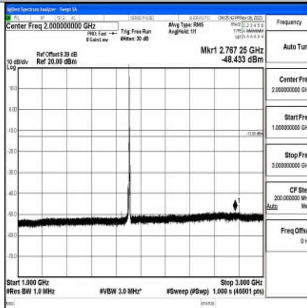
Band2_5MHz_16QAM_19175_1RB#0_1000~3000_1000~3000
