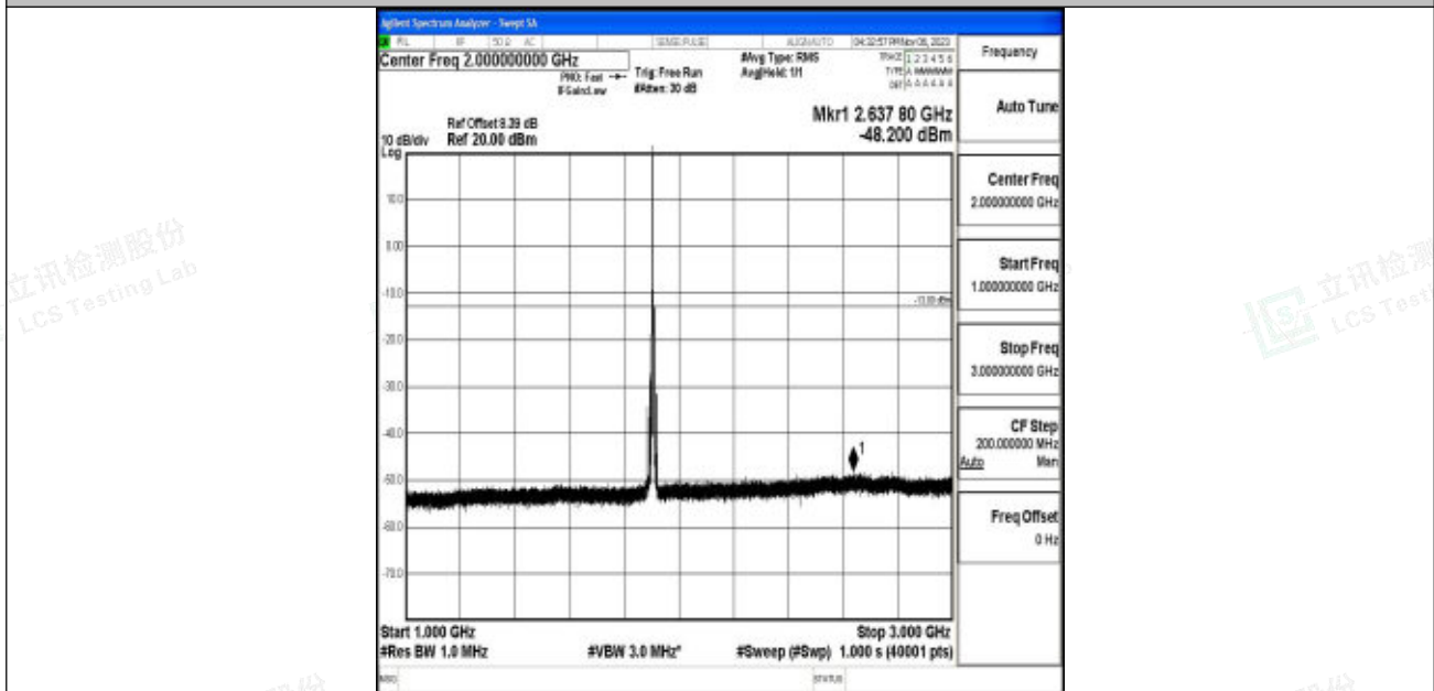
Band2_10MHz_64QAM_19150_1RB#0_1000~3000_1000~3000
