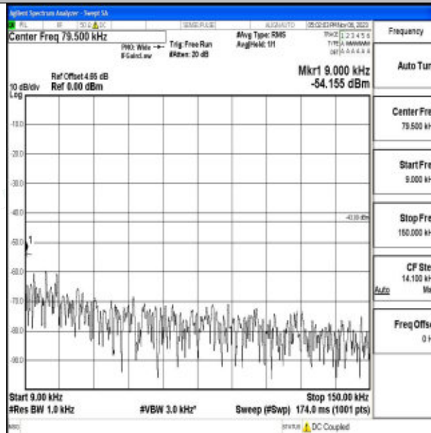
Band2_15MHz_64QAM_19125_1RB#0_0.009~0.15_0.009~0.15
