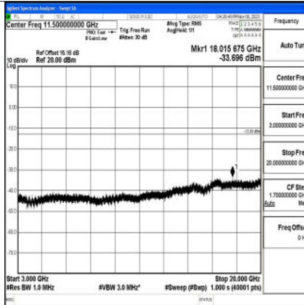
Band2_10MHz_64QAM_18650_1RB#0_3000~20000_3000~20000
