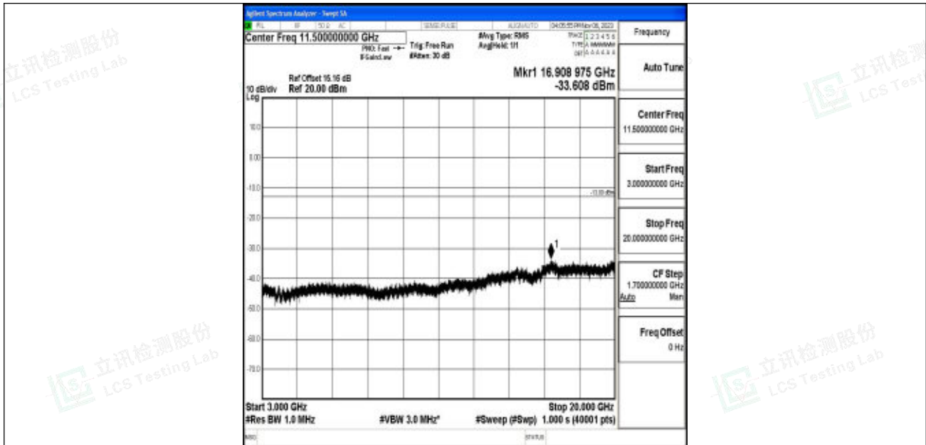
Band2_5MHz_16QAM_19175_1RB#0_3000~20000_3000~20000
