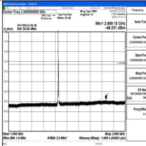
Band2_5MHz_64QAM_18625_1RB#0_1000~3000_1000~3000
