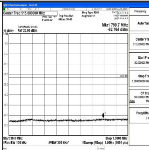
Band2_10MHz_16QAM_18650_1RB#0_30~1000_30~1000
