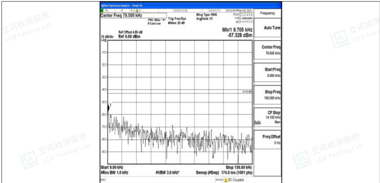
Band2_10MHz_QPSK_19150_1RB#0_0.009~0.15_0.009~0.15
