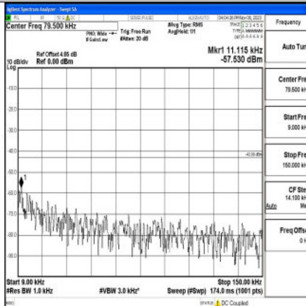
Band2_5MHz_QPSK_19175_1RB#0_0.009~0.15_0.009~0.15
