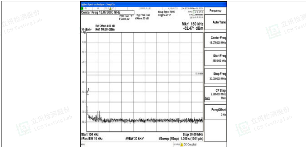
Band2_10MHz_64QAM_18900_1RB#0_0.15~30_0.15~30
