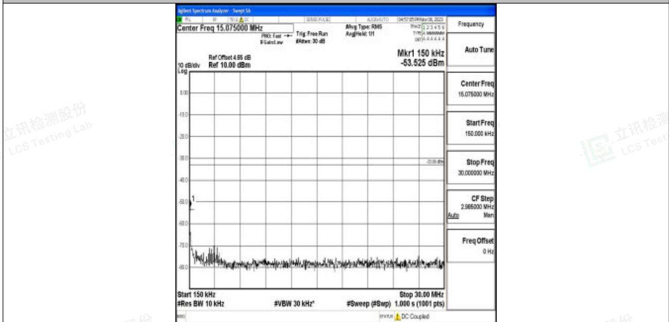
Band2_15MHz_16QAM_18675_1RB#0_0.15~30_0.15~30
