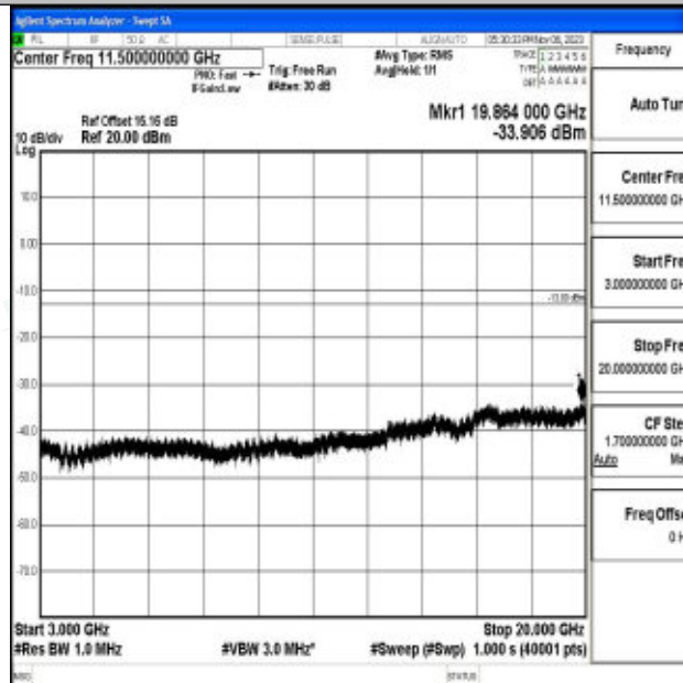
Band2_20MHz_16QAM_19100_1RB#0_3000~20000_3000~20000
