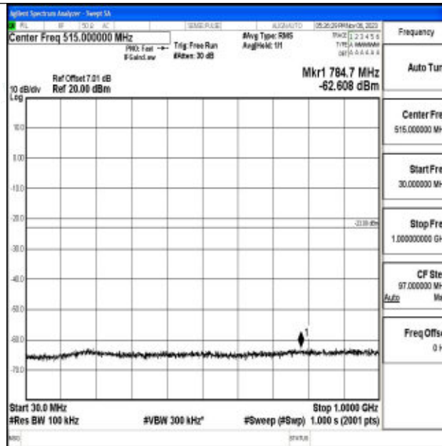
Band2_20MHz_64QAM_18700_1RB#0_30~1000_30~1000
