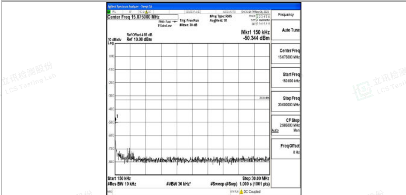
Band2_10MHz_QPSK_19150_1RB#0_0.15~30_0.15~30
