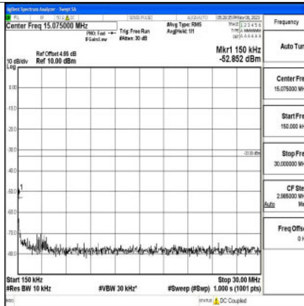
Band2_20MHz_64QAM_18900_1RB#0_0.15~30_0.15~30
