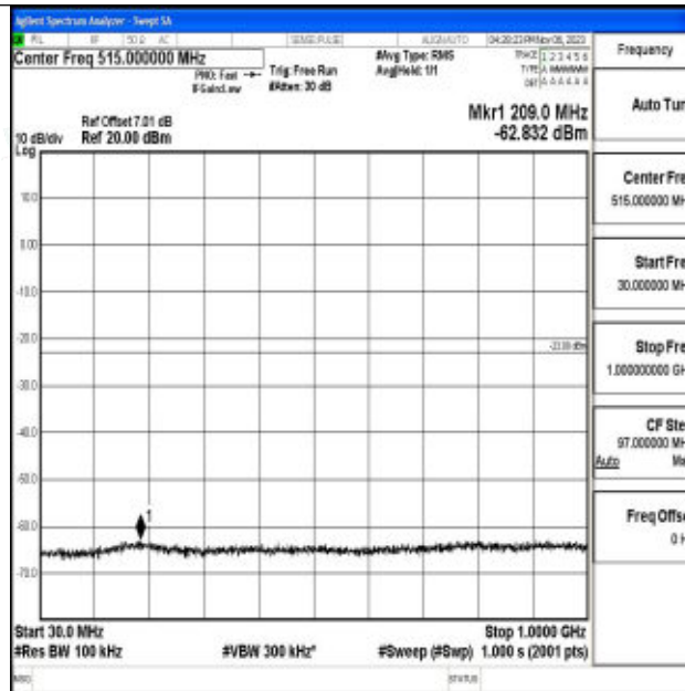
Band2_10MHz_64QAM_18650_1RB#0_30~1000_30~1000
