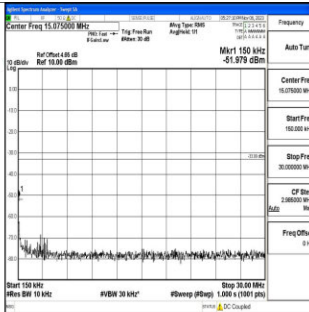
Band2_20MHz_QPSK_18900_1RB#0_0.15~30_0.15~30
