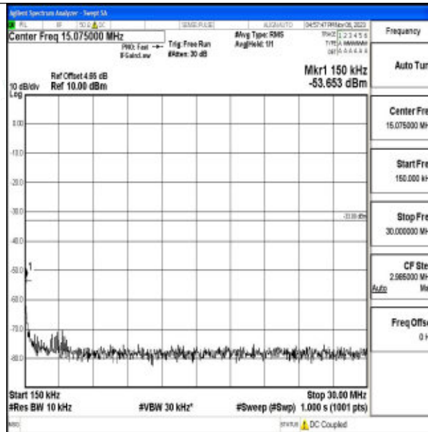
Band2_15MHz_64QAM_18675_1RB#0_0.15~30_0.15~30
