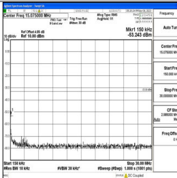
Band2_20MHz_64QAM_18700_1RB#0_0.15~30_0.15~30
