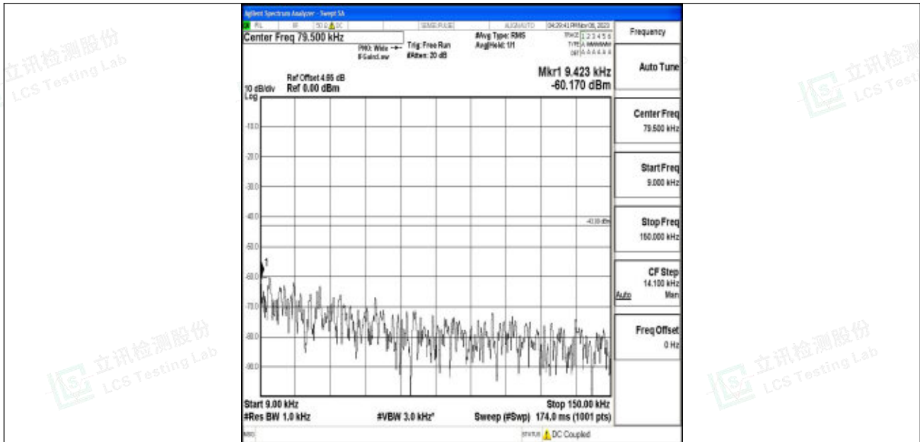
Band2_10MHz_16QAM_18900_1RB#0_0.009~0.15_0.009~0.15
