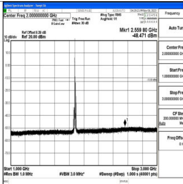
Band2_10MHz_QPSK_18900_1RB#0_1000~3000_1000~3000
