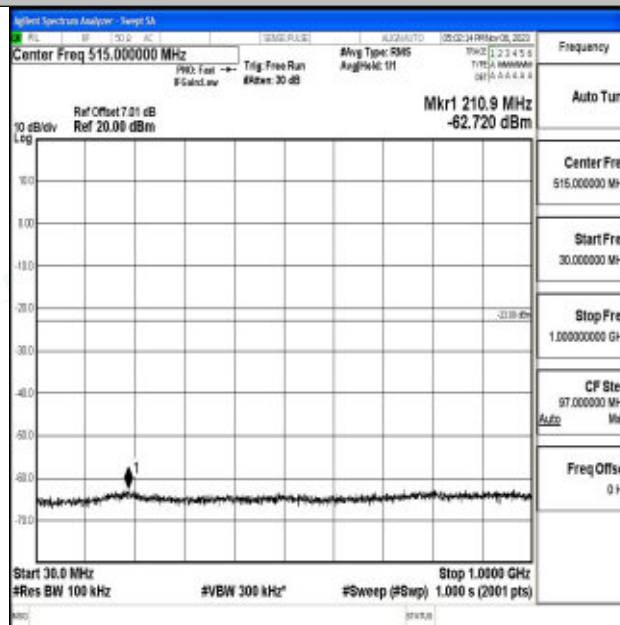
Band2_15MHz_64QAM_19125_1RB#0_30~1000_30~1000
