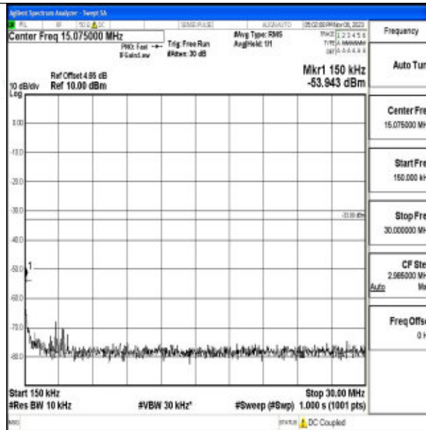
Band2_15MHz_64QAM_19125_1RB#0_0.15~30_0.15~30
