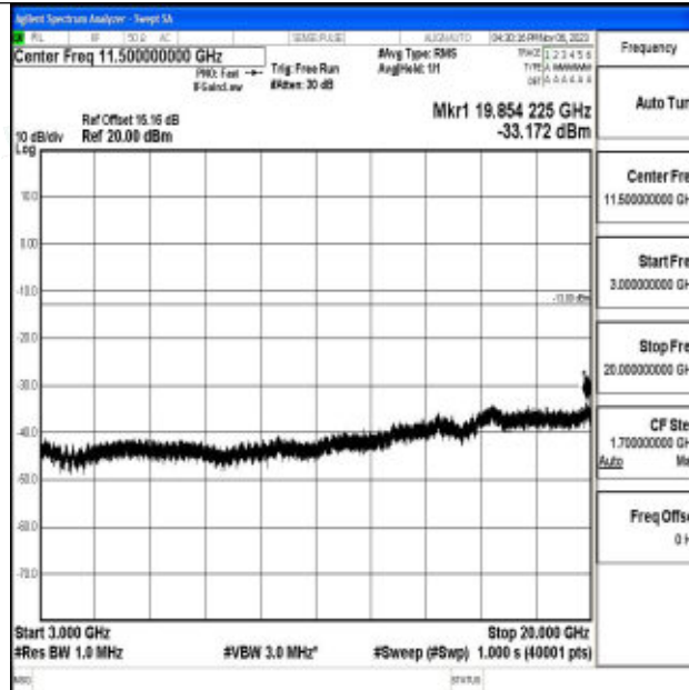
Band2_10MHz_16QAM_18900_1RB#0_3000~20000_3000~20000
