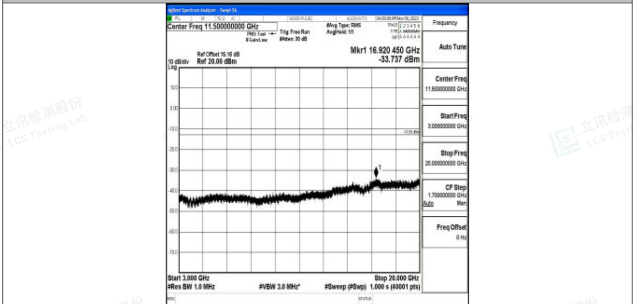
Band2_10MHz_16QAM_18650_1RB#0_3000~20000_3000~20000
