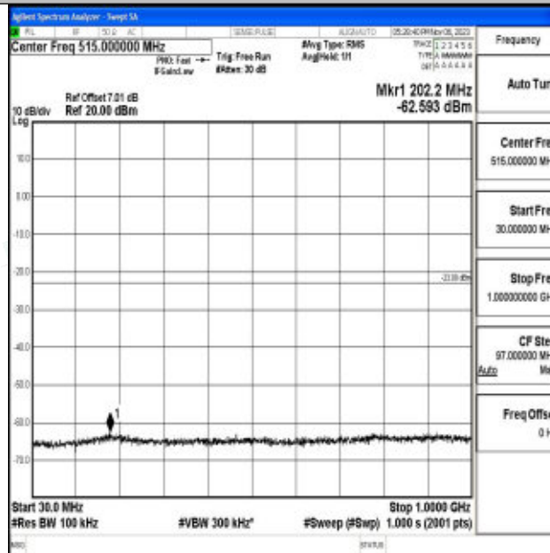
Band2_20MHz_64QAM_18900_1RB#0_30~1000_30~1000
