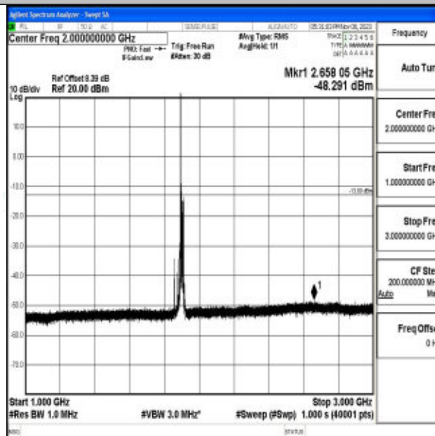
Band2_20MHz_64QAM_19100_1RB#0_1000~3000_1000~3000
