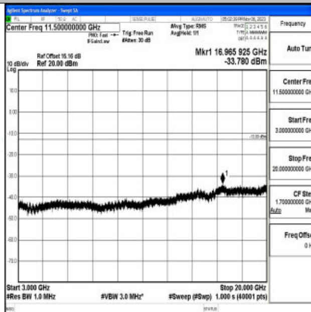
Band2_15MHz_64QAM_19125_1RB#0_3000~20000_3000~20000
