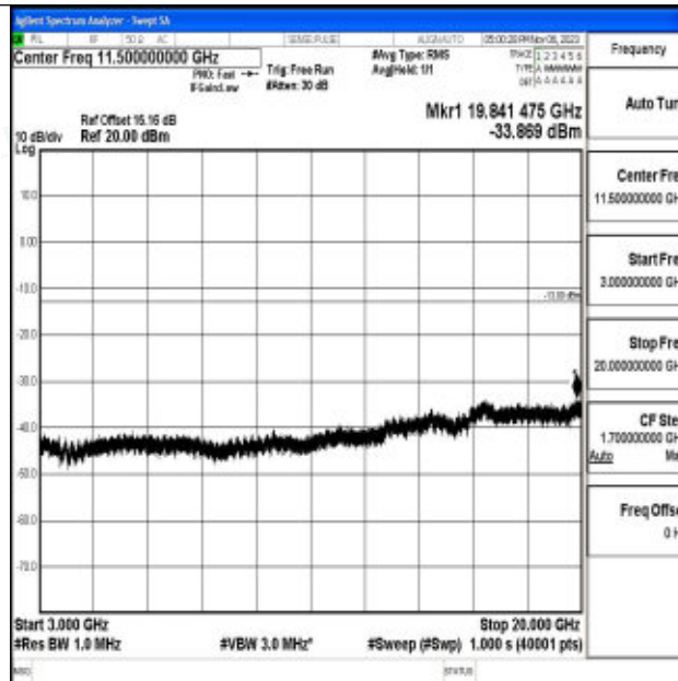
Band2_15MHz_64QAM_18900_1RB#0_3000~20000_3000~20000
