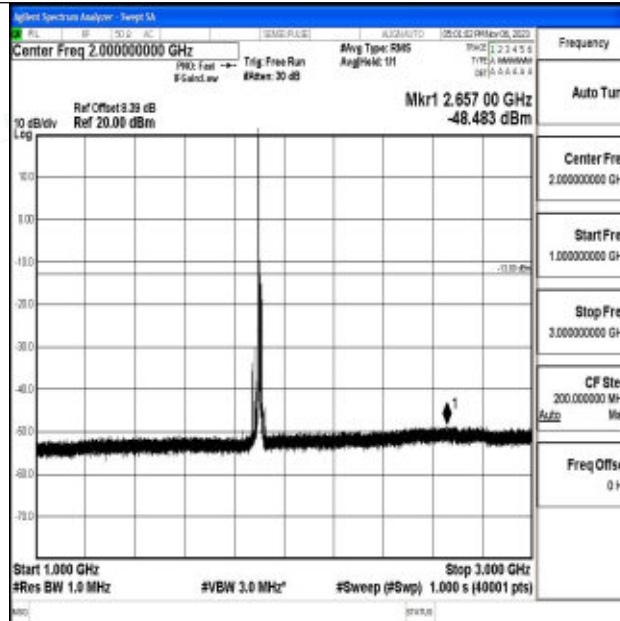
Band2_15MHz_QPSK_19125_1RB#0_1000~3000_1000~3000
