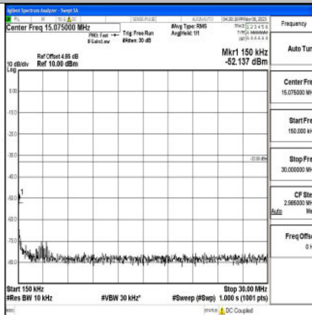
Band2_10MHz_64QAM_18650_1RB#0_0.15~30_0.15~30
