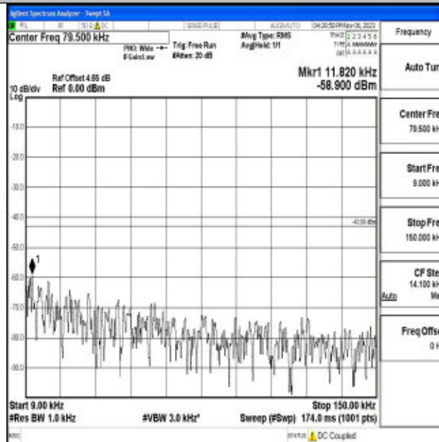
Band2_10MHz_QPSK_18900_1RB#0_0.009~0.15_0.009~0.15
