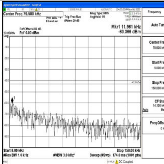
Band2_10MHz_64QAM_18900_1RB#0_0.009~0.15_0.009~0.15
