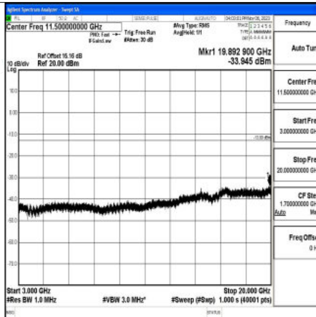
Band2_5MHz_QPSK_18900_1RB#0_3000~20000_3000~20000
