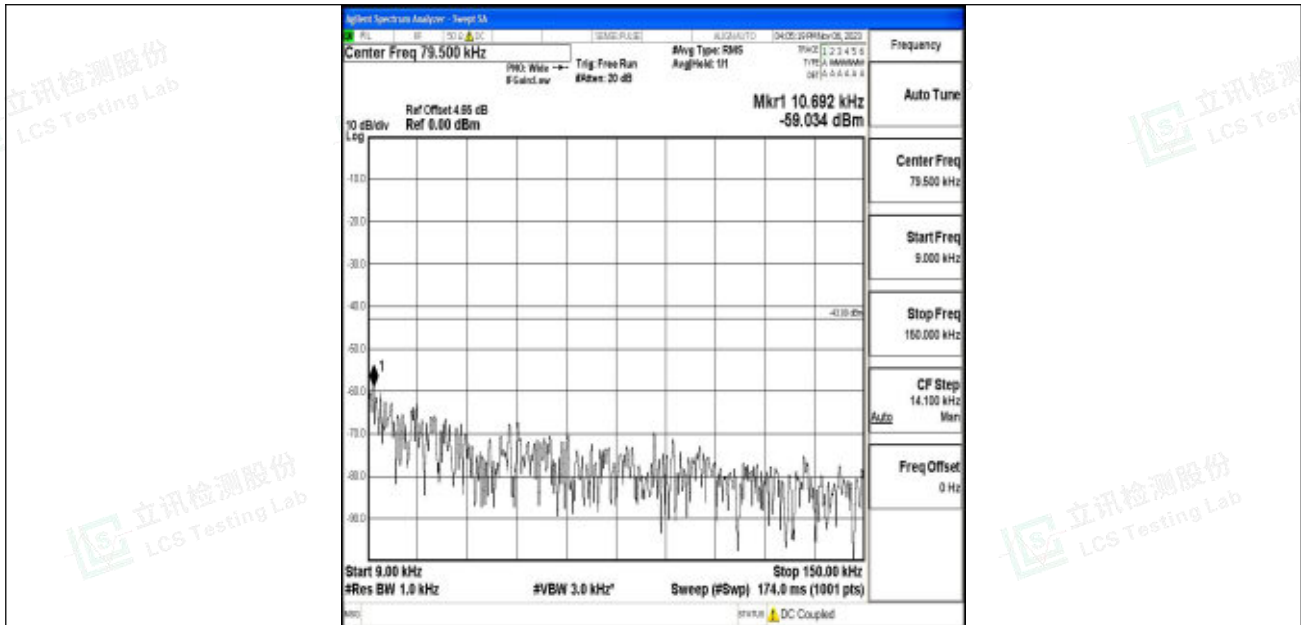
Band2_5MHz_16QAM_19175_1RB#0_0.009~0.15_0.009~0.15
