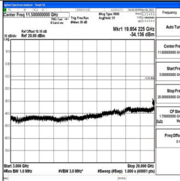
Band2_5MHz_64QAM_19175_1RB#0_3000~20000_3000~20000
