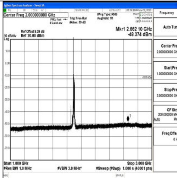
Band2_20MHz_QPSK_19100_1RB#0_1000~3000_1000~3000
