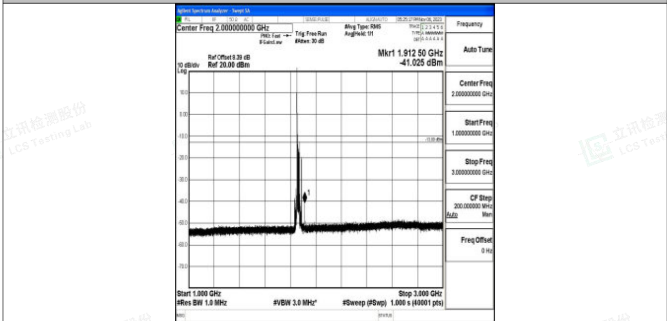
Band2_20MHz_QPSK_18700_1RB#0_1000~3000_1000~3000
