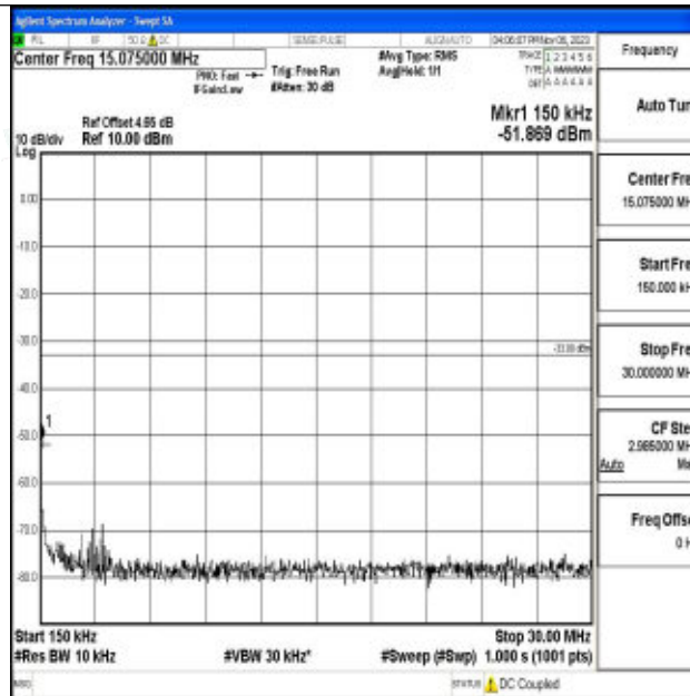
Band2_5MHz_64QAM_19175_1RB#0_0.15~30_0.15~30
