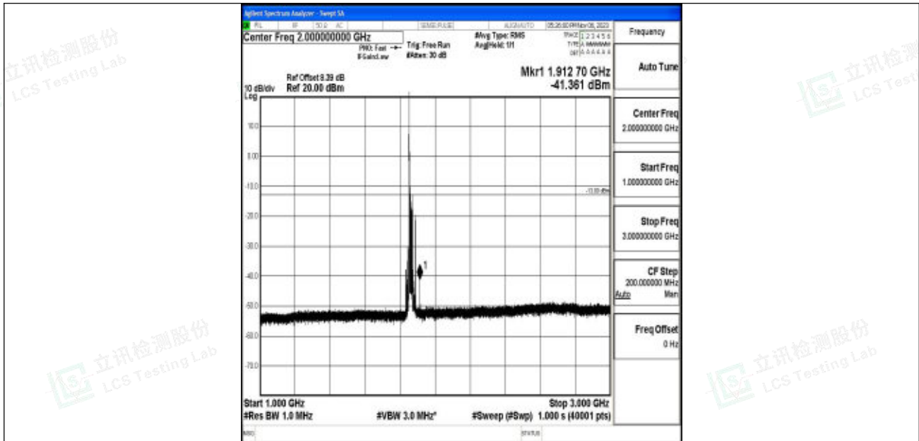
Band2_20MHz_16QAM_18700_1RB#0_1000~3000_1000~3000
