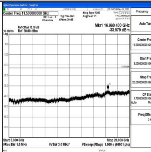
Band2_20MHz_64QAM_18900_1RB#0_3000~20000_3000~20000
