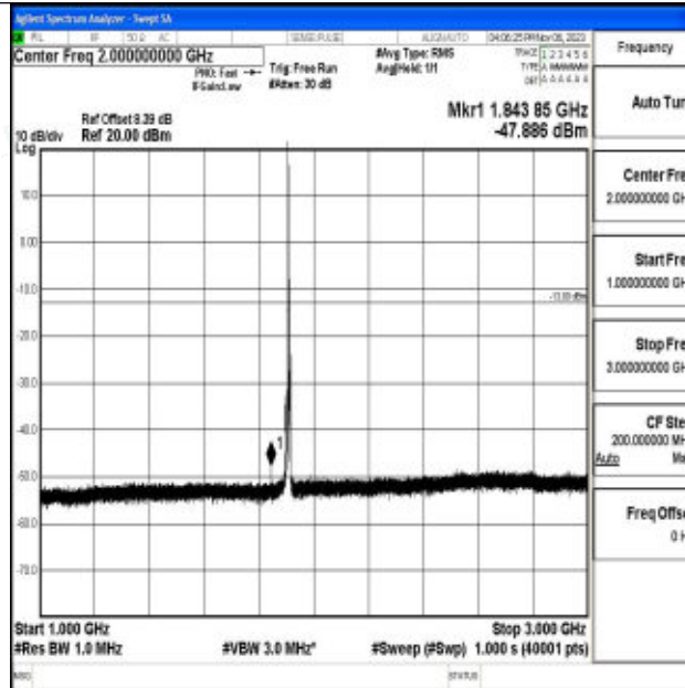
Band2_5MHz_64QAM_19175_1RB#0_1000~3000_1000~3000
