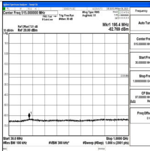
Band2_20MHz_64QAM_19100_1RB#0_30~1000_30~1000
