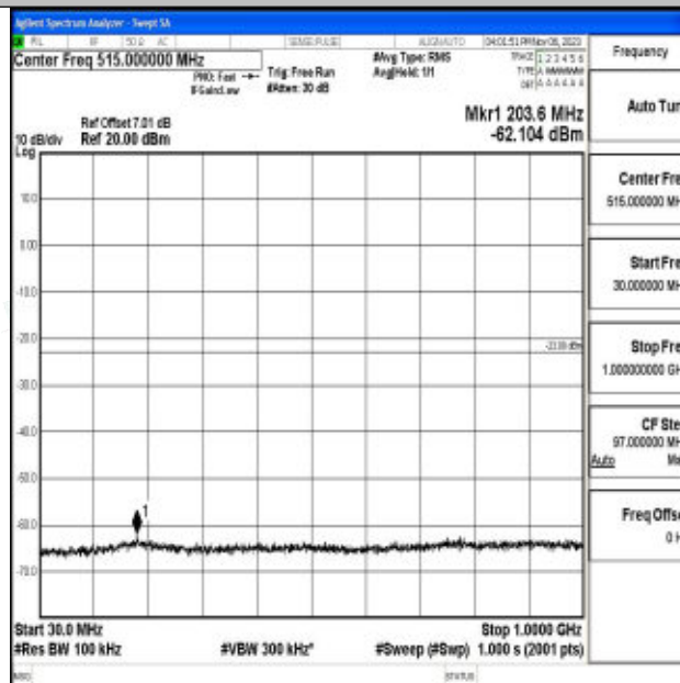
Band2_5MHz_64QAM_18625_1RB#0_30~1000_30~1000
