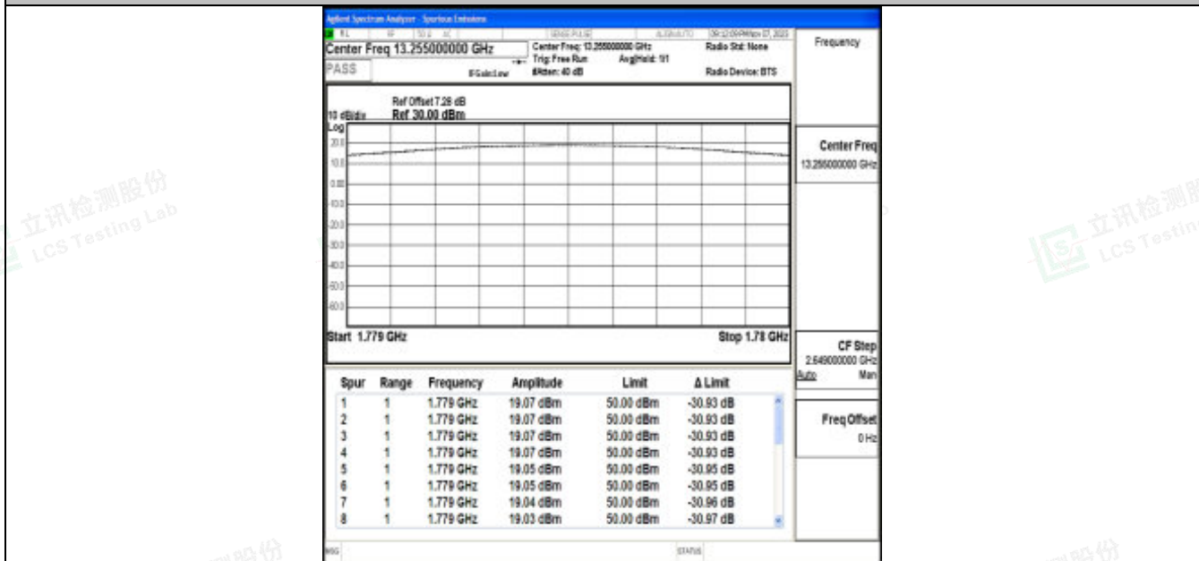
Band66_1.4MHz_QPSK_132665_6RB#0
