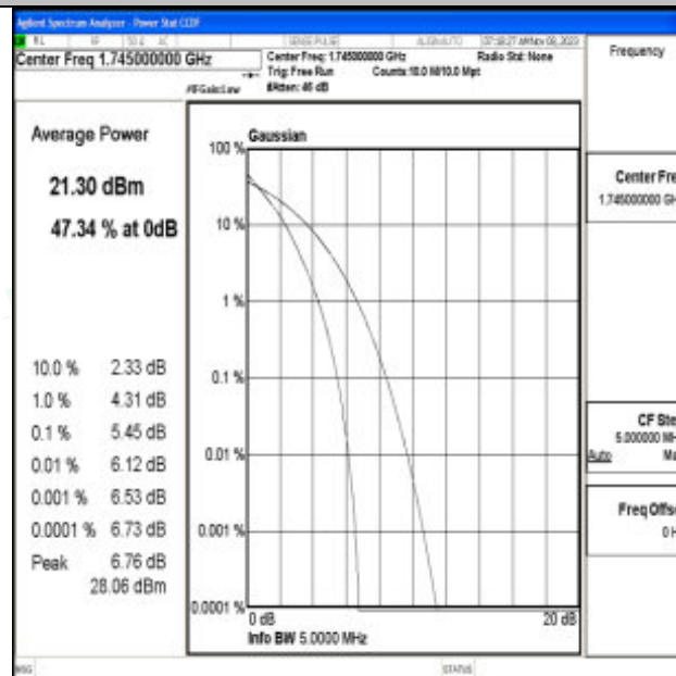
Band66-5MHz-QPSK-132322-25RB#0-PASS
