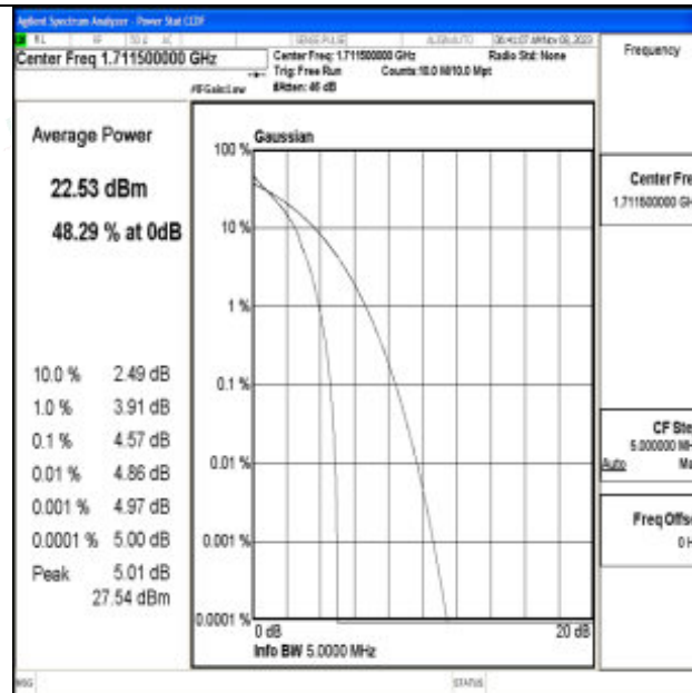
Band66-3MHz-QPSK-131987-1RB#0-PASS
