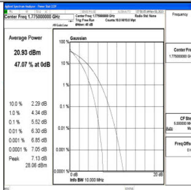
Band66-10MHz-64QAM-132622-50RB#0-PASS
