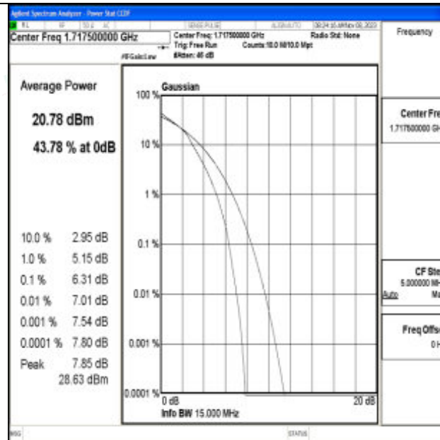
Band66-15MHz-16QAM-132047-75RB#0-PASS
