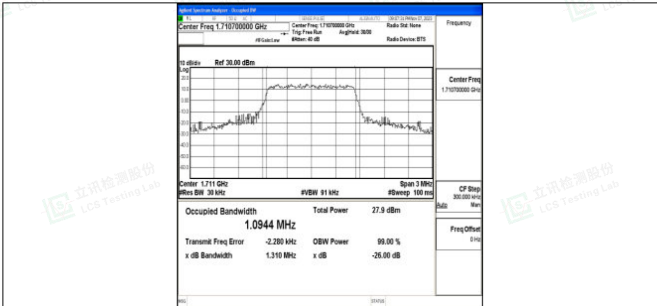
Band66-1.4MHz-QPSK-131979-6RB#0-PASS
