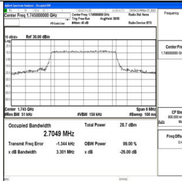
Band66-3MHz-16QAM-132322-15RB#0-PASS
