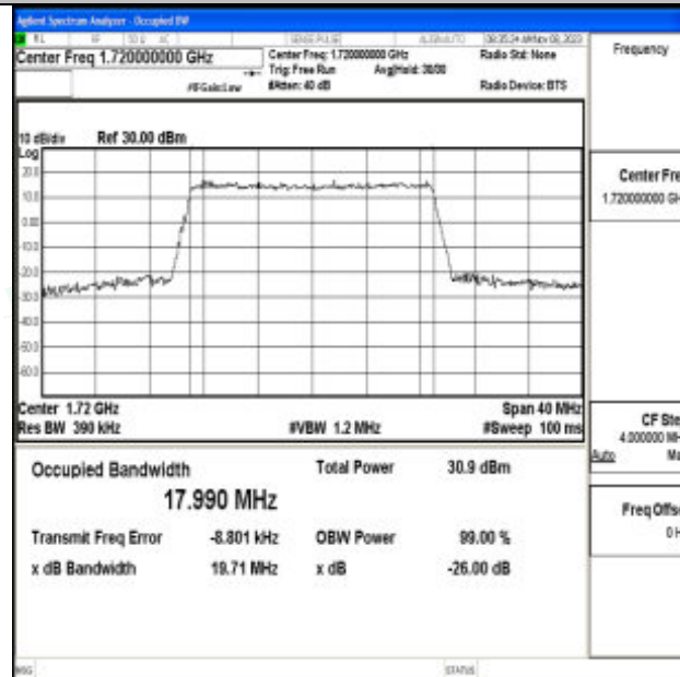
Band66-20MHz-QPSK-132072-100RB#0-PASS
