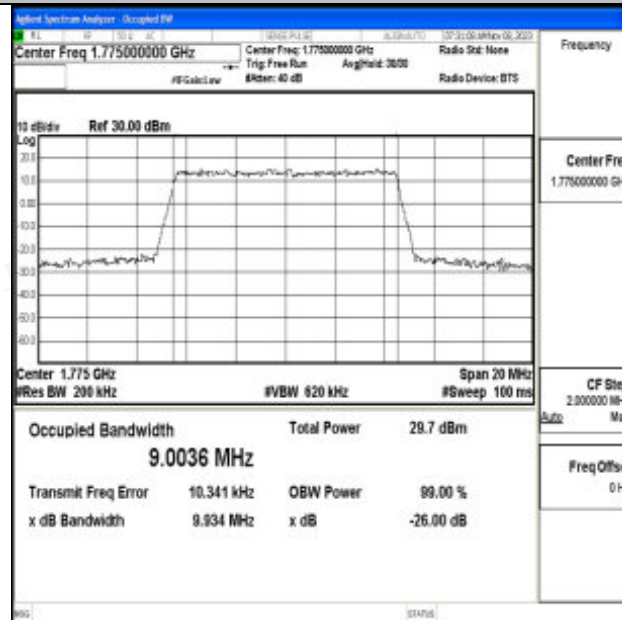
Band66-10MHz-QPSK-132622-50RB#0-PASS
