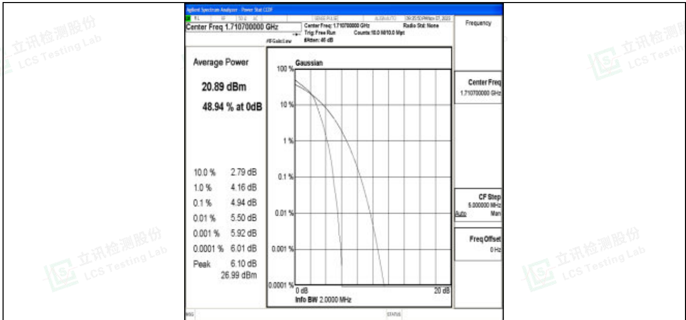
Band66-1.4MHz-16QAM-131979-6RB#0-PASS
