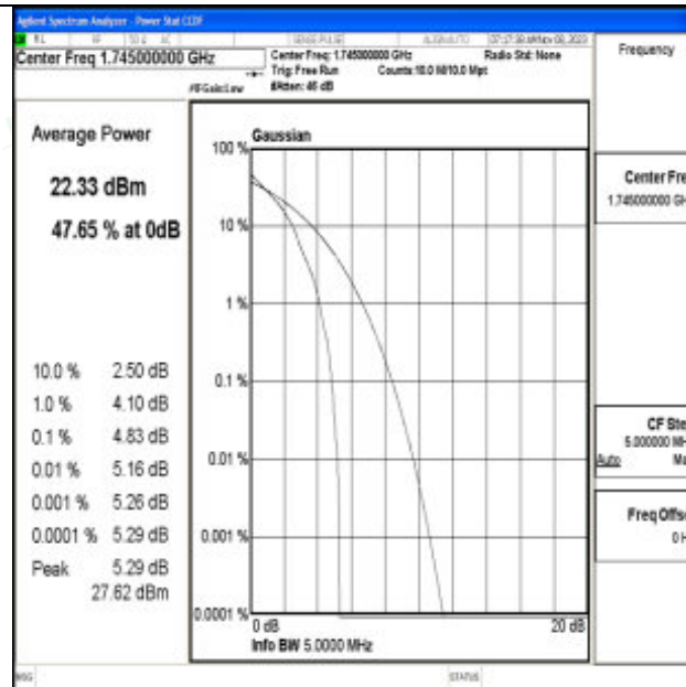
Band66-5MHz-64QAM-132322-1RB#0-PASS
