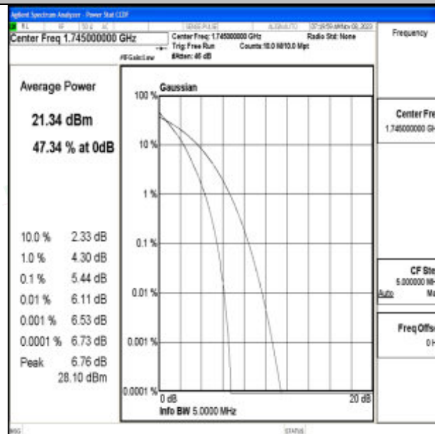
Band66-5MHz-64QAM-132322-25RB#0-PASS
