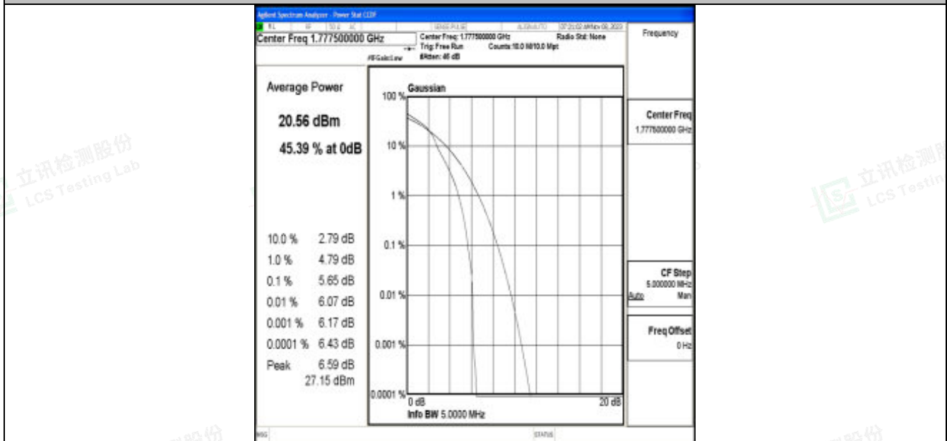
Band66-5MHz-16QAM-132647-1RB#0-PASS
