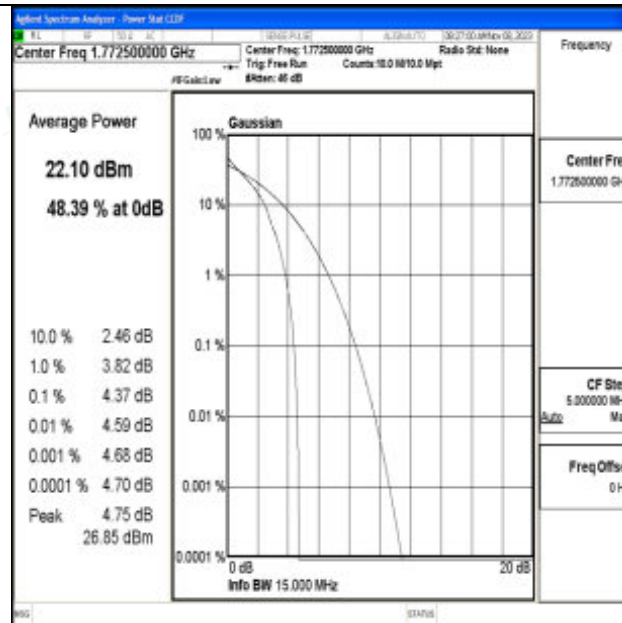
Band66-15MHz-64QAM-132597-1RB#0-PASS
