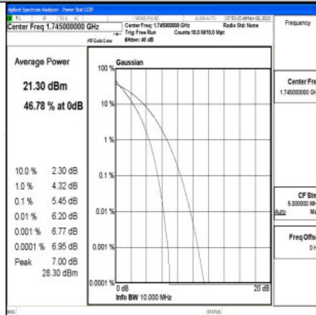
Band66-10MHz-QPSK-132322-50RB#0-PASS
