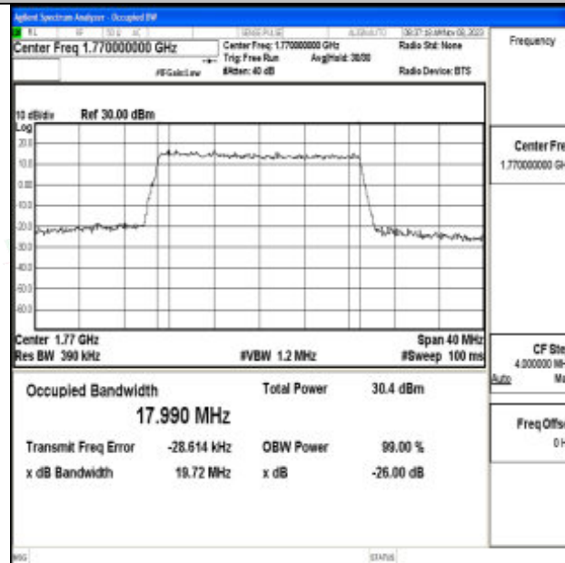
Band66-20MHz-64QAM-132572-100RB#0-PASS
