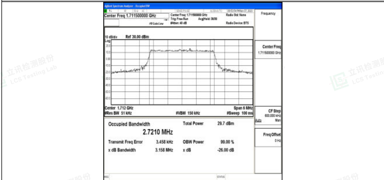
Band66-3MHz-64QAM-131987-15RB#0-PASS
