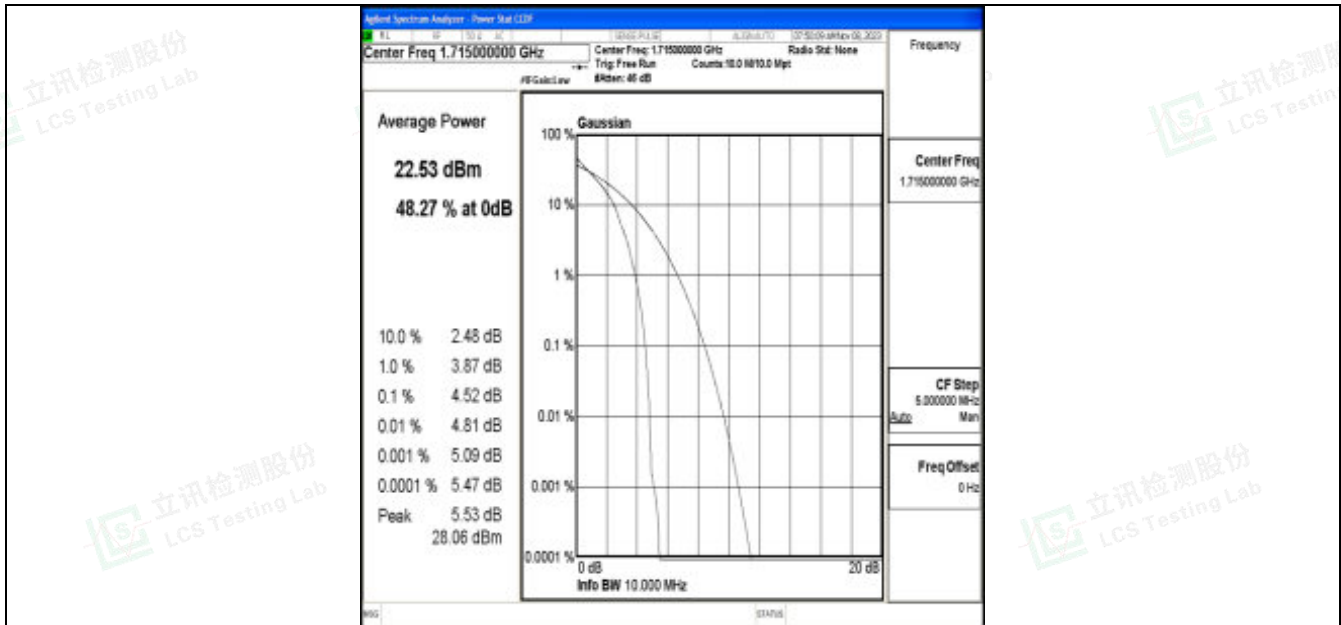
Band66-10MHz-QPSK-132022-1RB#0-PASS
