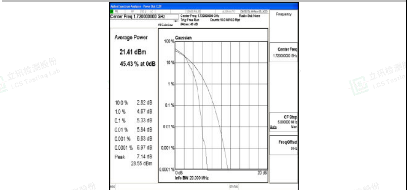
Band66-20MHz-16QAM-132072-1RB#0-PASS
