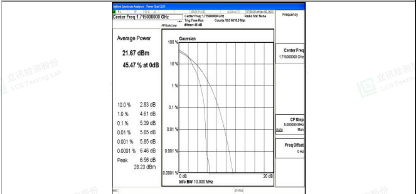
Band66-10MHz-16QAM-132022-1RB#0-PASS
