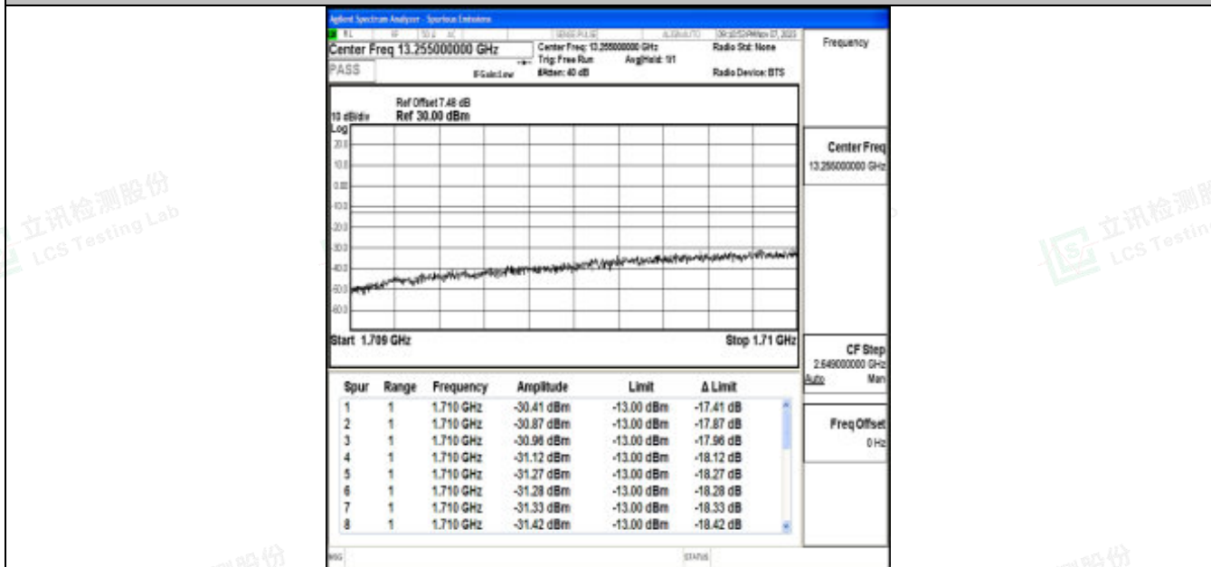
Band66_1.4MHz_16QAM_131979_6RB#0
