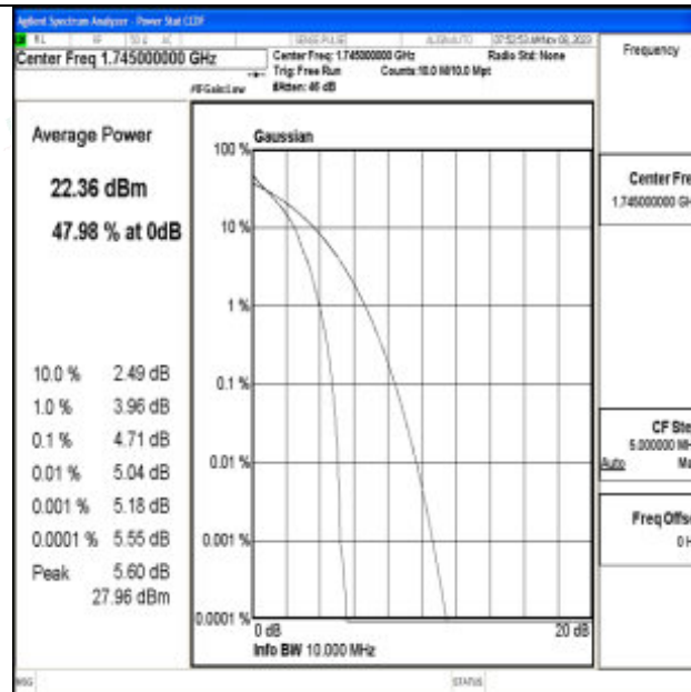
Band66-10MHz-64QAM-132322-1RB#0-PASS
