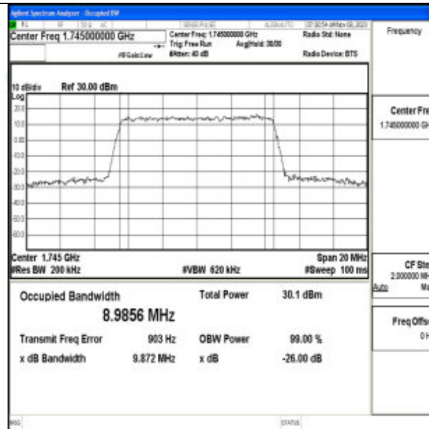
Band66-10MHz-64QAM-132322-50RB#0-PASS
