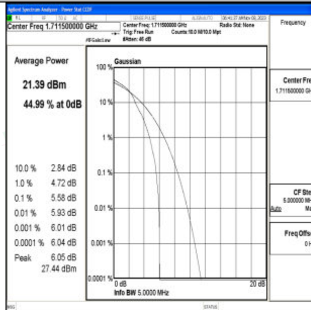
Band66-3MHz-16QAM-131987-1RB#0-PASS
