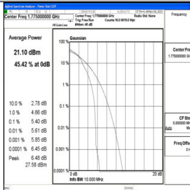
Band66-10MHz-16QAM-132622-1RB#0-PASS
