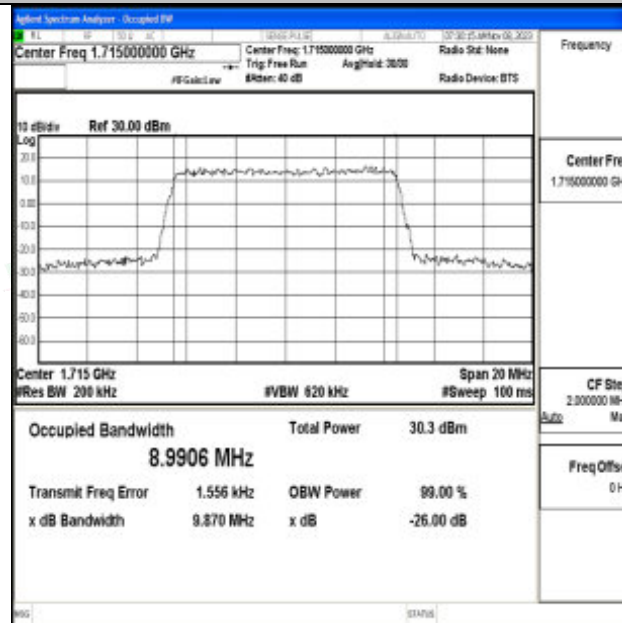
Band66-10MHz-64QAM-132022-50RB#0-PASS
