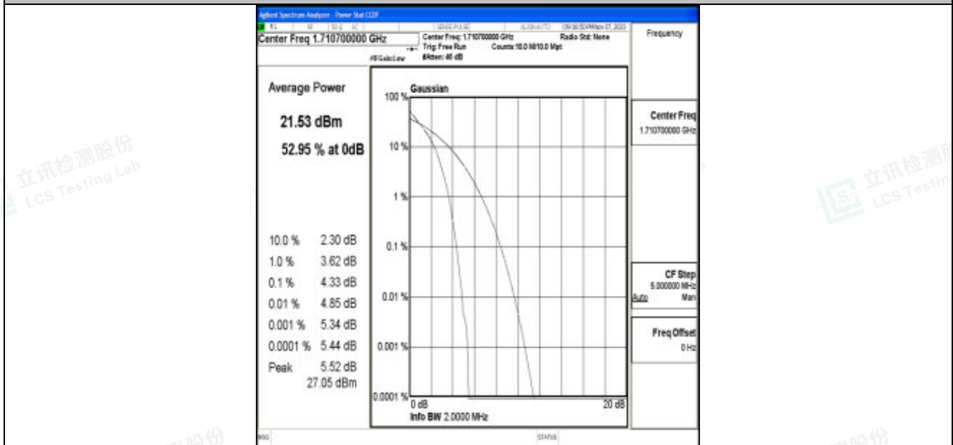
Band66-1.4MHz-64QAM-131979-6RB#0-PASS
