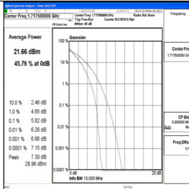
Band66-15MHz-64QAM-132047-75RB#0-PASS
