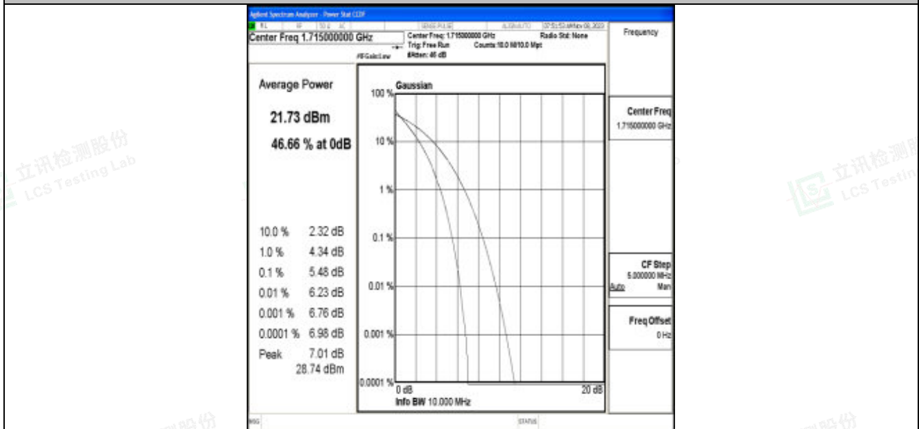
Band66-10MHz-64QAM-132022-50RB#0-PASS
