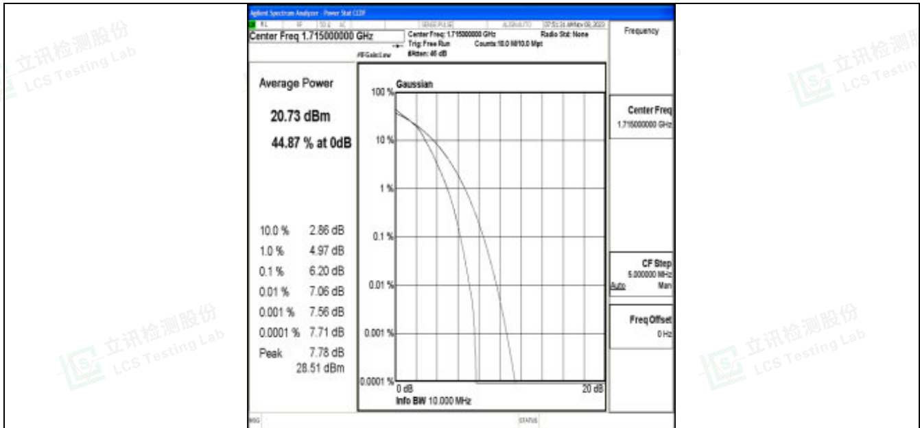
Band66-10MHz-16QAM-132022-50RB#0-PASS
