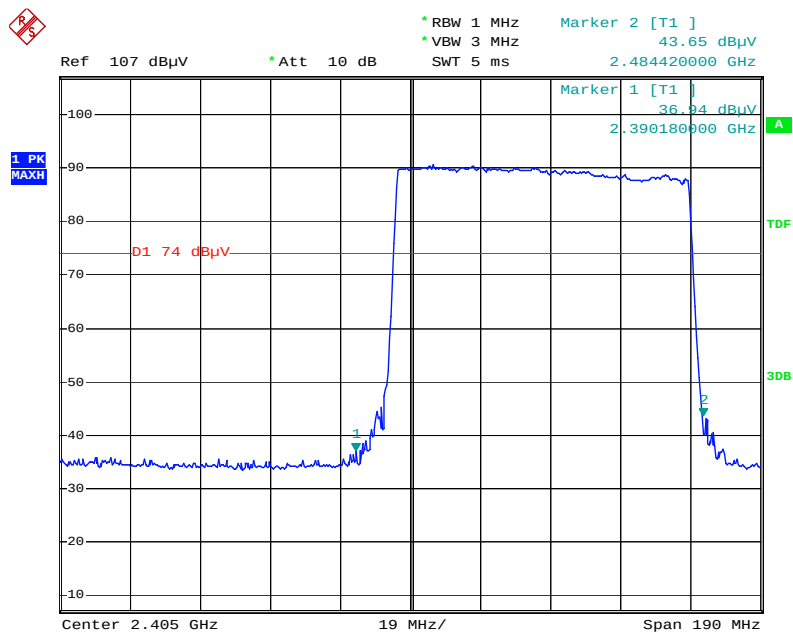
GFSK-hopping-PK
