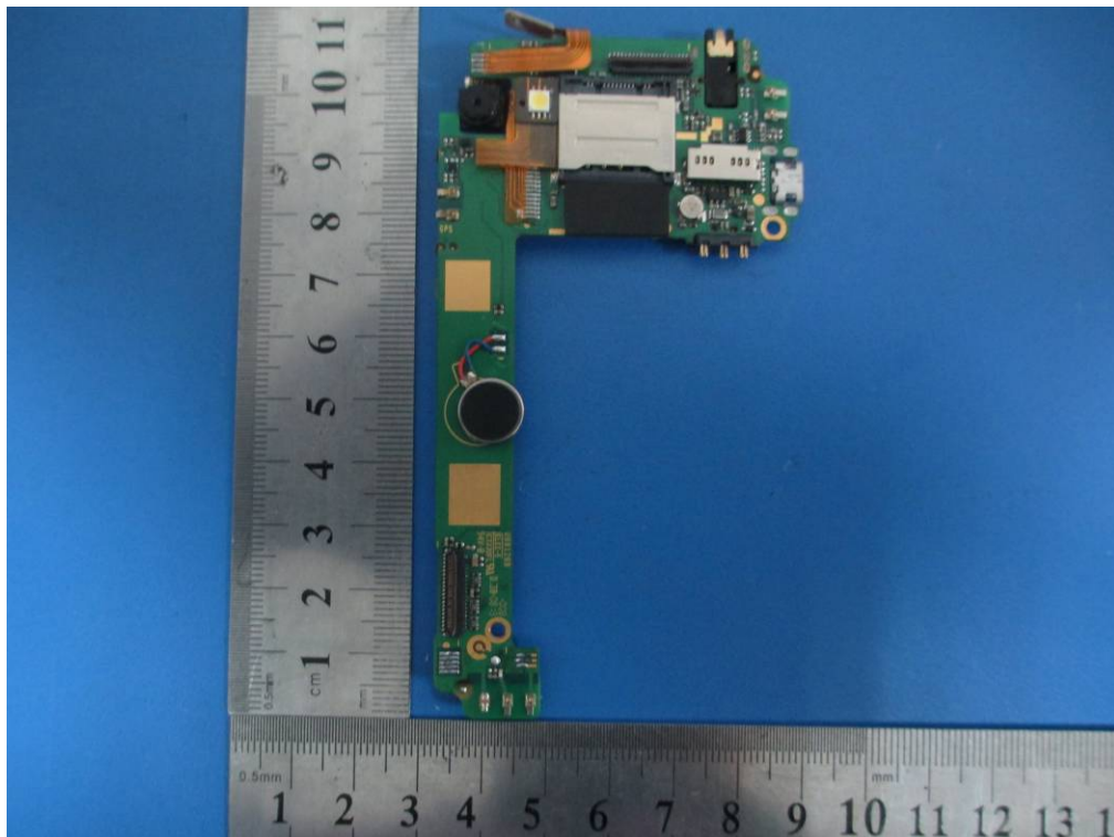
Top - PCB 1#
