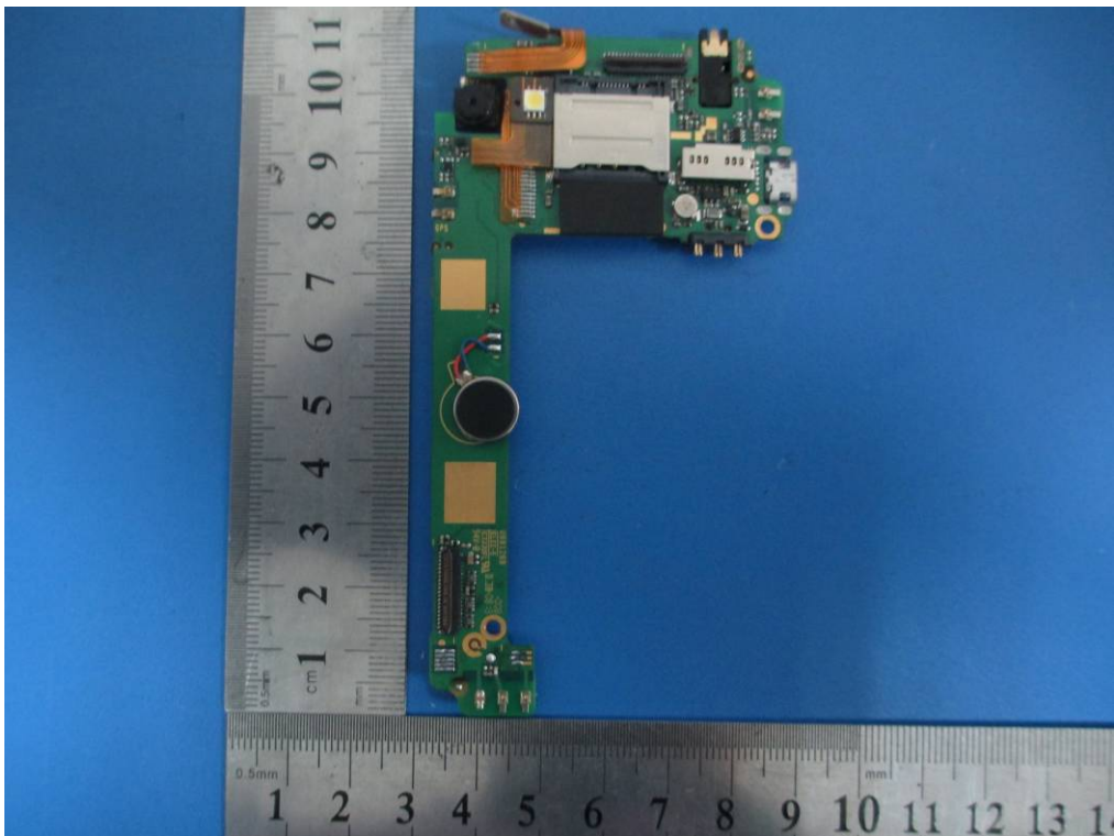
Top - PCB 1#
