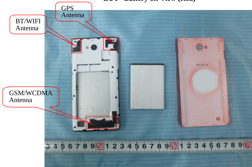
EUT –Battery off View (Red)
