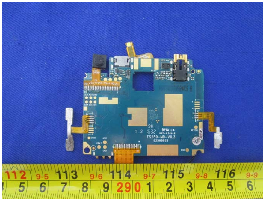
EUT –MB1 Unshield Bottom View
