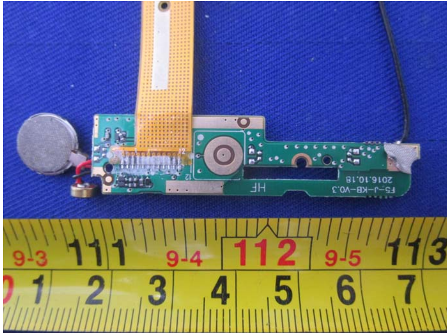
EUT –MB2 Bottom View
