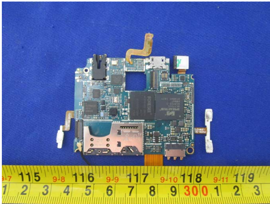
EUT –MB1 Unshield Top View
