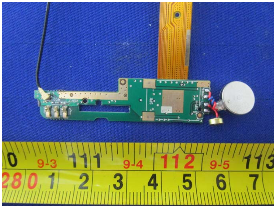
EUT –MB2 Top View
