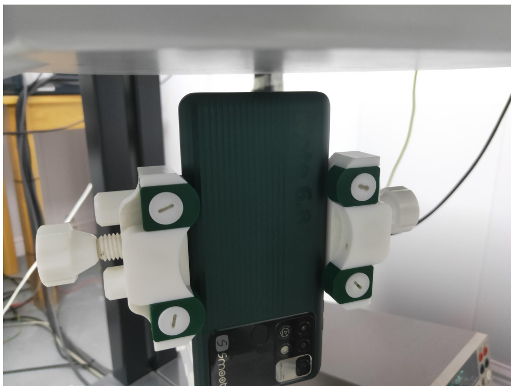
10mm body-worn Bottom Side Setup Photo (hotspot)
