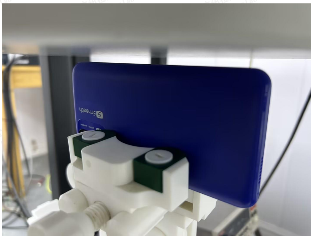
10mm body Vertical- Left Side Setup Photo
