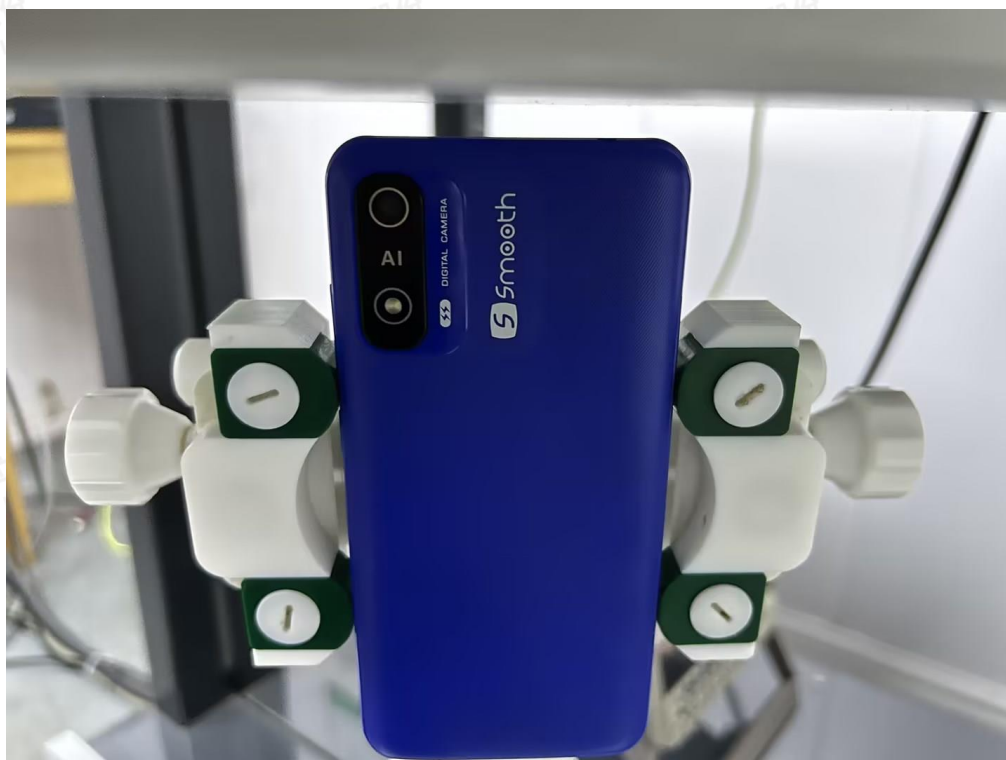
10mm body Vertical-Top Side Setup Photo
