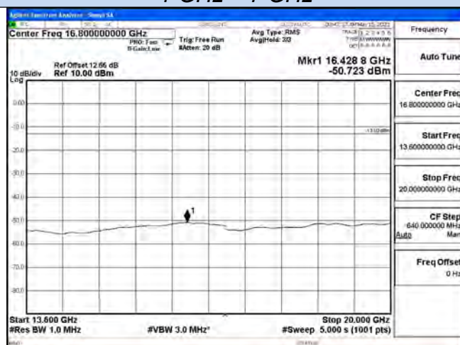
13.6 GHz – 20 GHz
