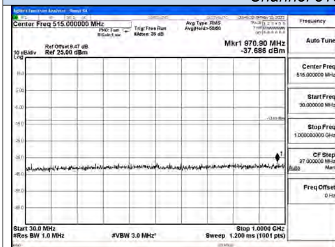
30 MHz – 1000 MHz
