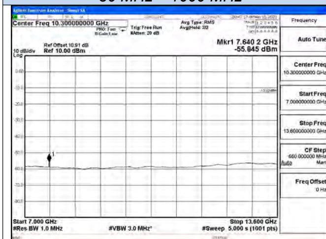
7 GHz – 13.6 GHz
