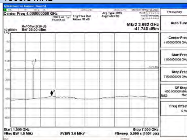
1 GHz – 7 GHz
