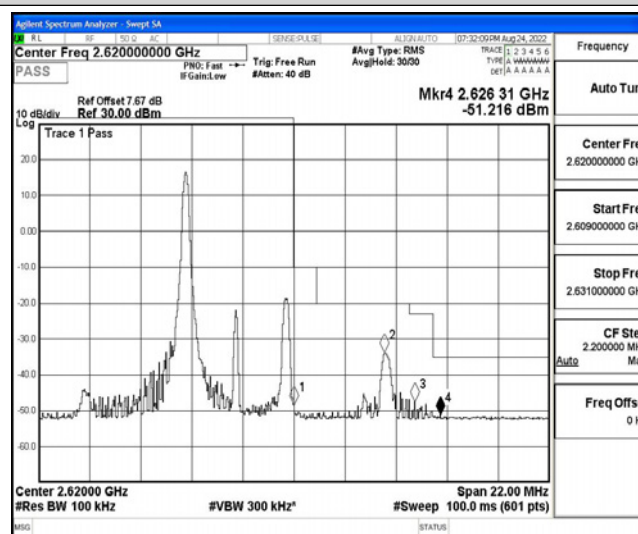
Band38-5MHz-QPSK-38225-1RB#24
