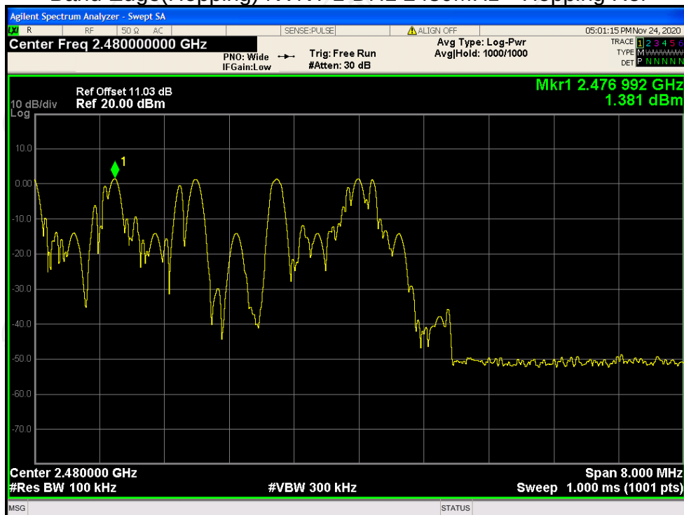
Band Edge(Hopping) NVNT 1-DH1 2480MHz Hopping Emission
