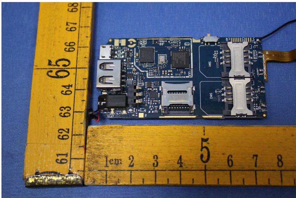
MAIN BOARD TOP VIEW 4 WITHOUT SHIELDED
