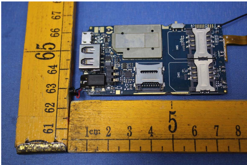
MAIN BOARD TOP VIEW WITH SHIELDED
