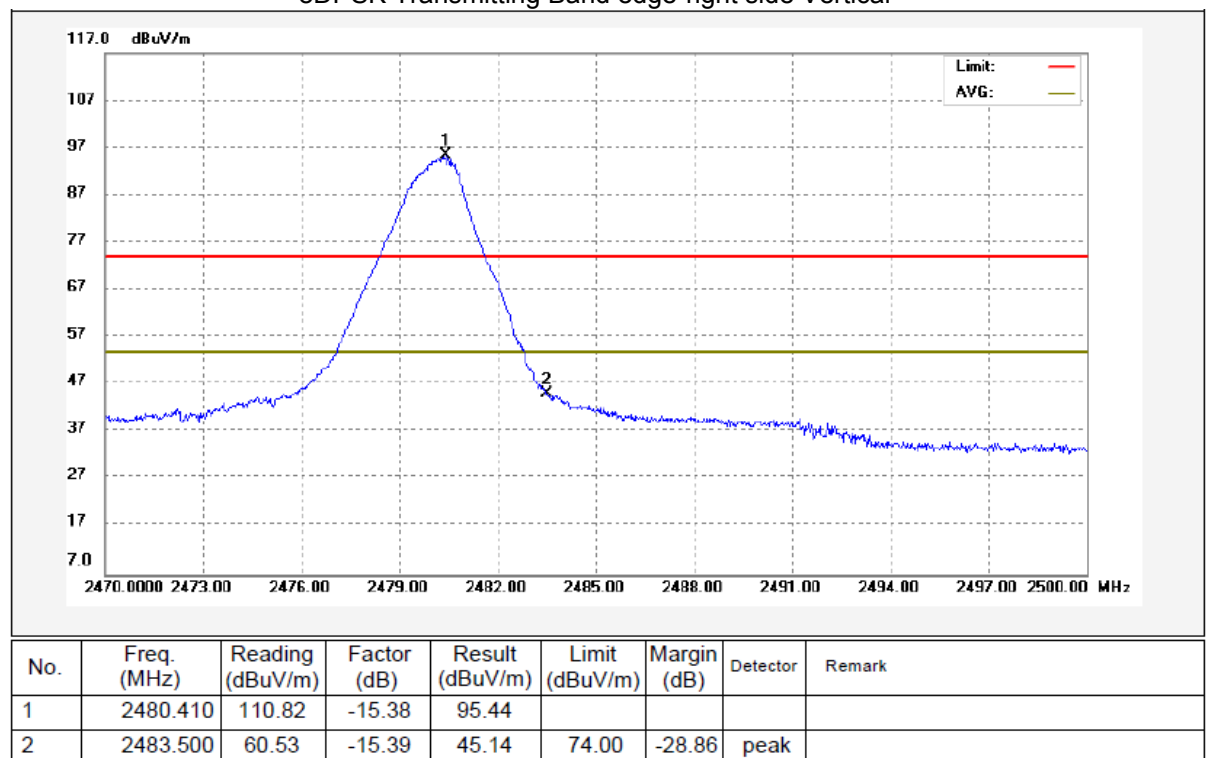
8DPSK Transmitting Band edge-right side Vertical
