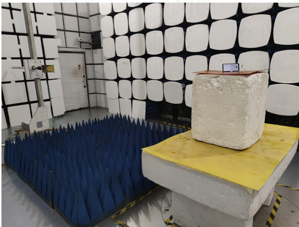
Radiated Emissions Measurement (Above 1GHz)
