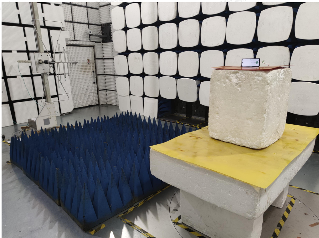
Radiated Emissions Measurement (Below 1GHz)
