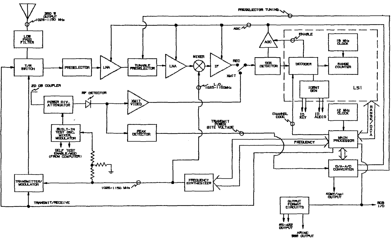
DME Module DM-850 Figure 4-1
