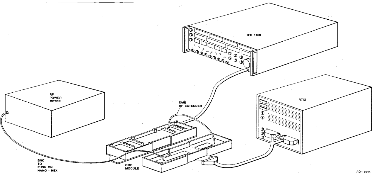
Figure B-1. Test Setup
