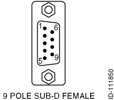
Figure 3-7. HSU Maintenance Connector (X1) Pin Layout
