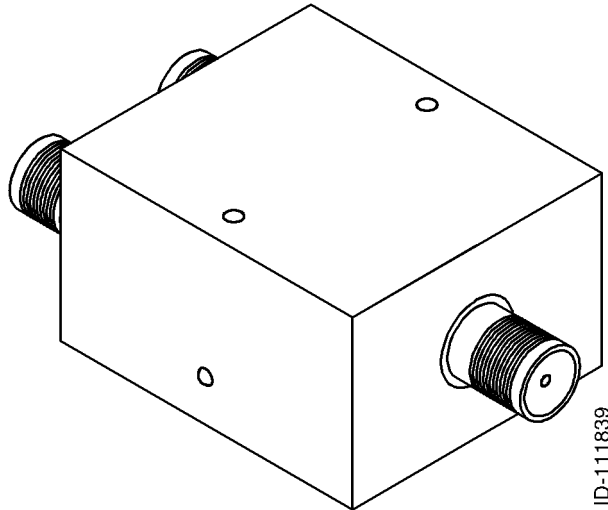
Figure 1-4. RF Splitter/Combiner
