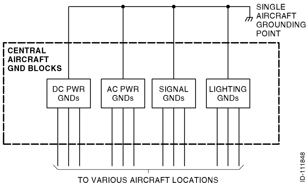
Figure 3-5. Aircraft Grounding
