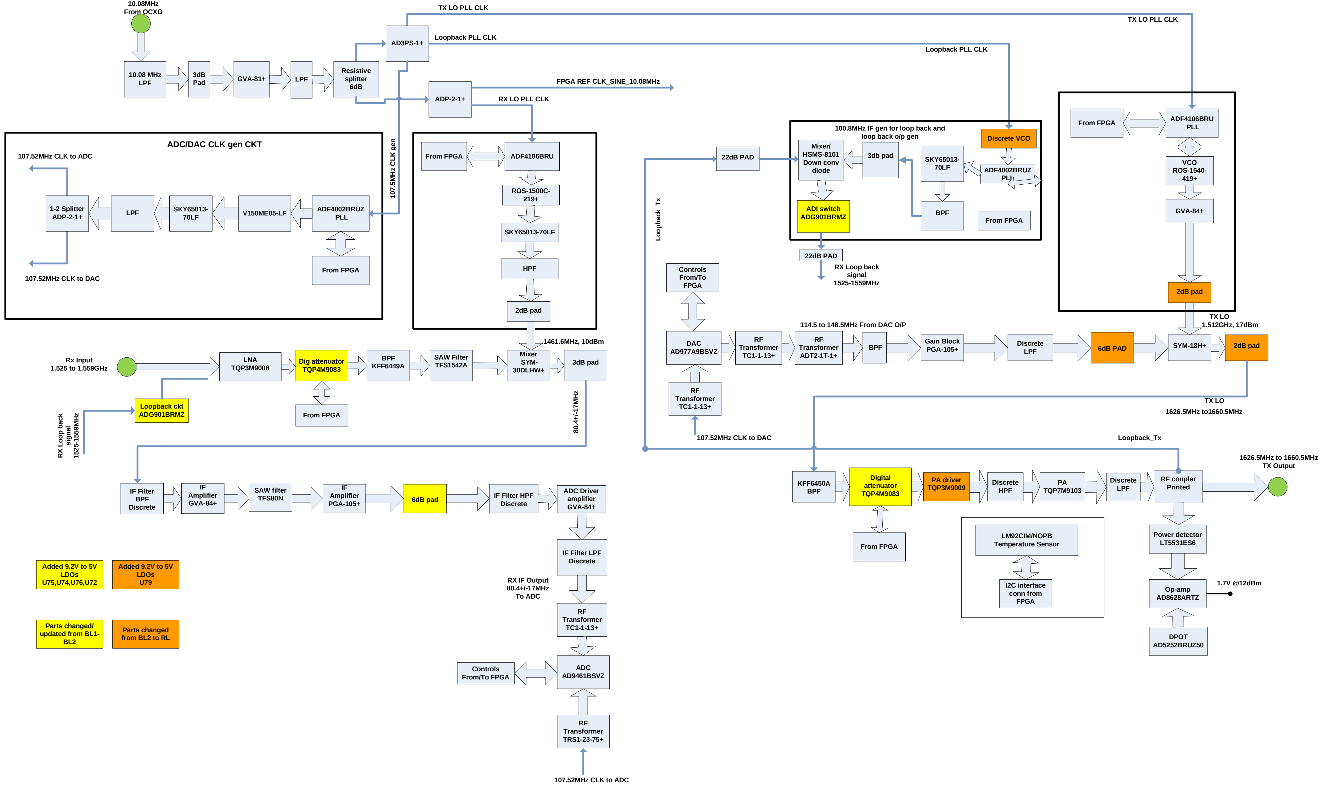
MCS-7000 DRFM Integrated RF Block Diagram
