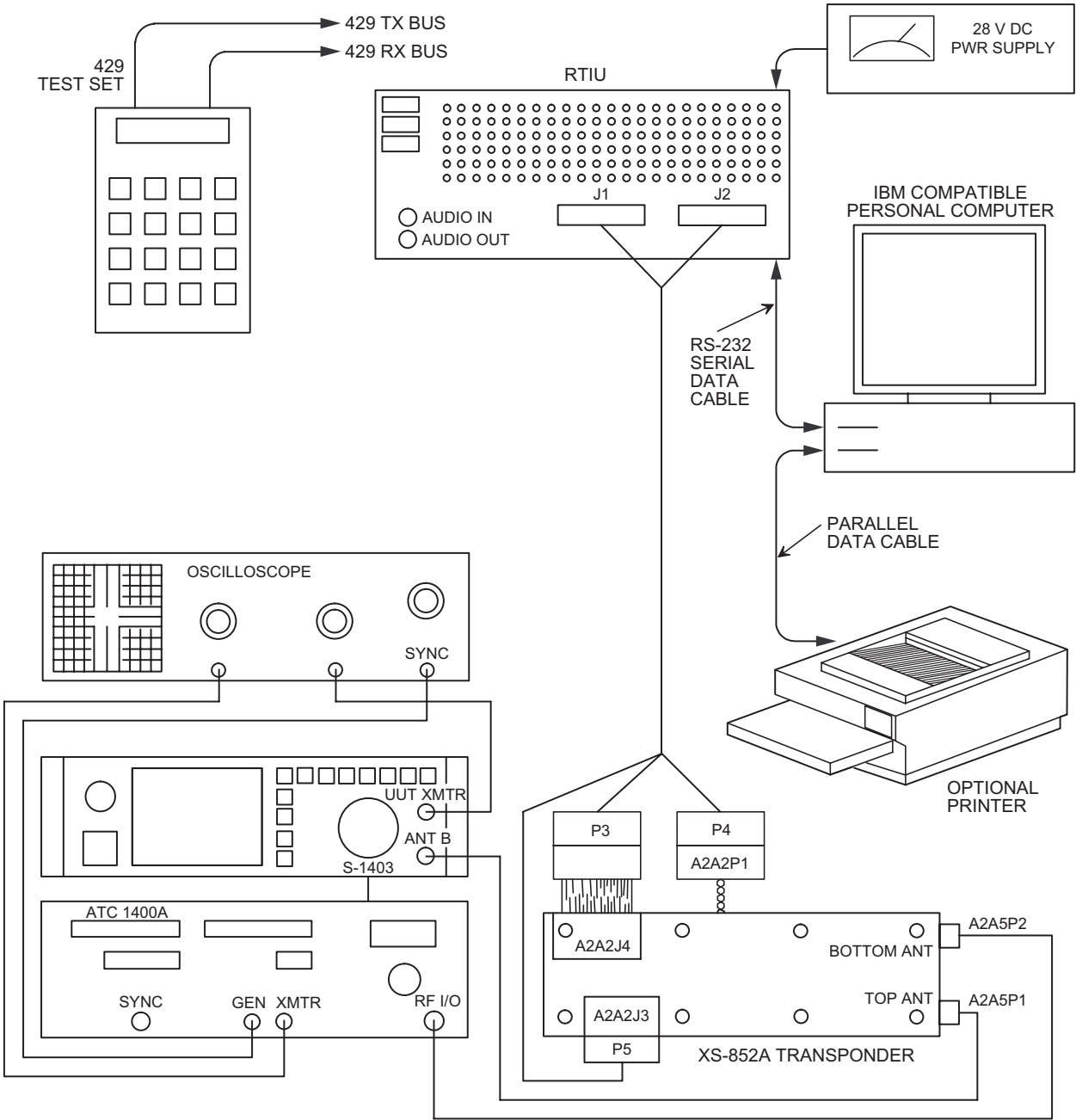
Figure 2. Test Equipment (-902, -903, -904)
