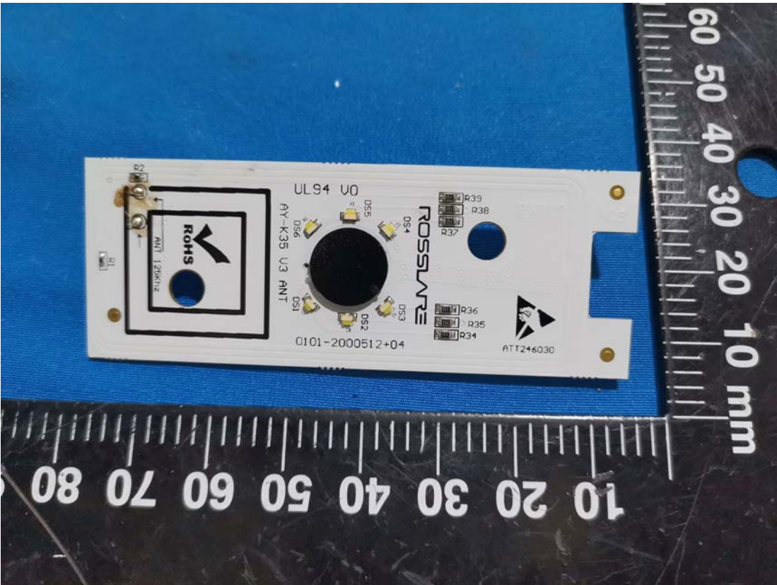
RFID Antenna Board
