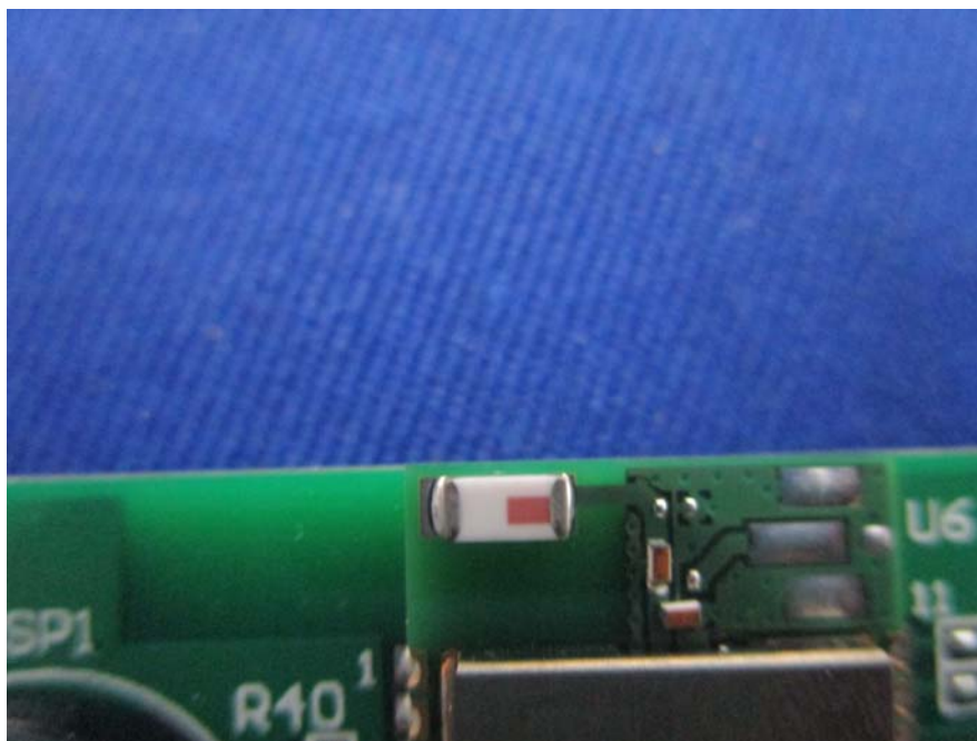
EUT – Bluetooth LE Module Antenna View
