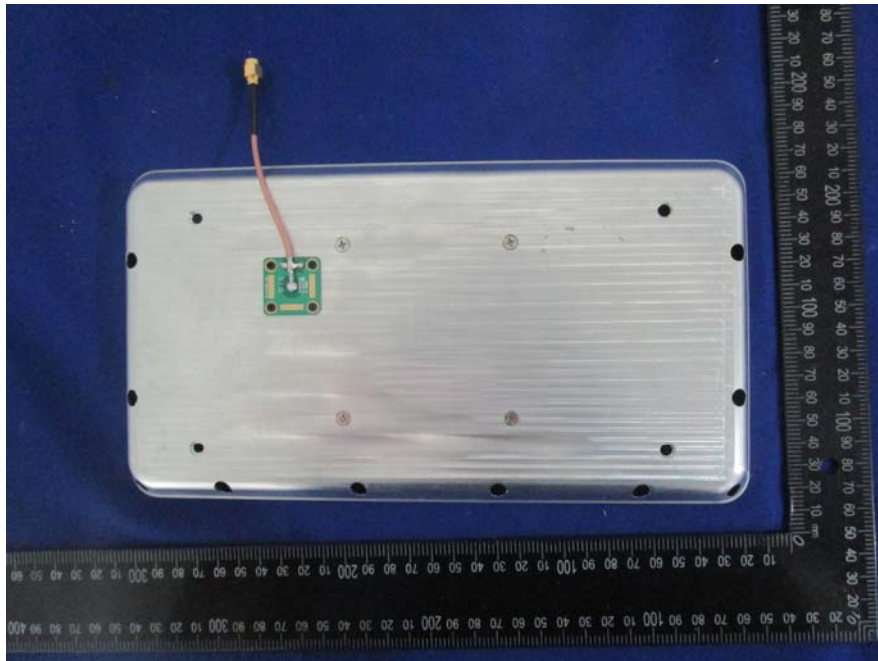
EUT – 915MHz Module Antenna Bottom View
