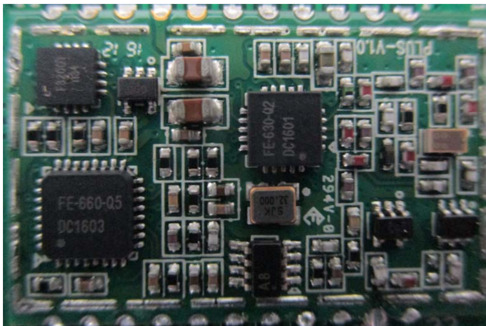
EUT – 915MHz Module Unshielded View
