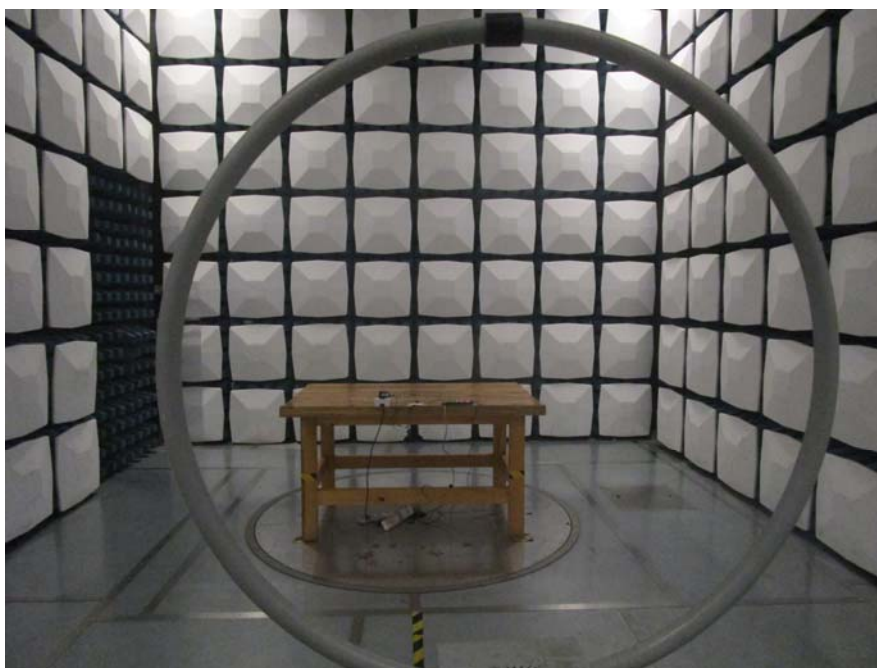
Radiated Emission Rear View (Below 30 MHz)
