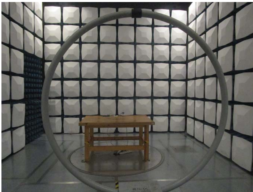
Radiated Emission Front View (Below 30 MHz)
