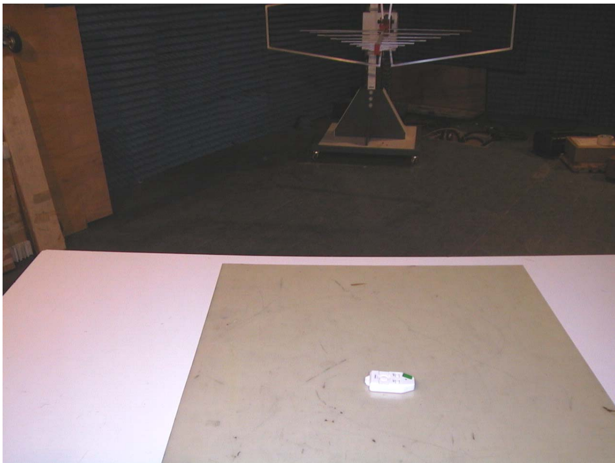
Radiated Emission Test Setup
