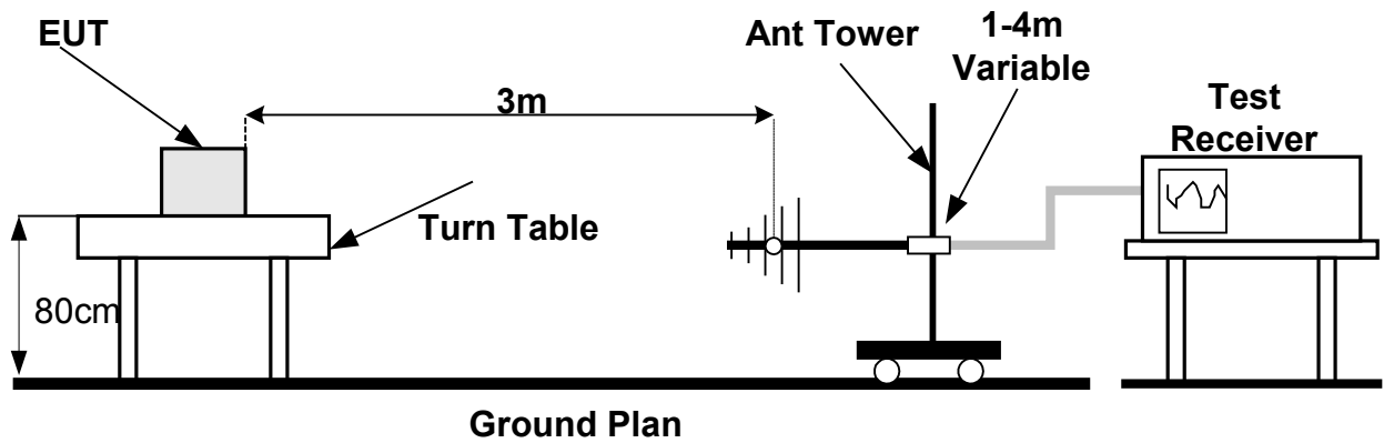
Figure 11 Radiated Emission Set up
