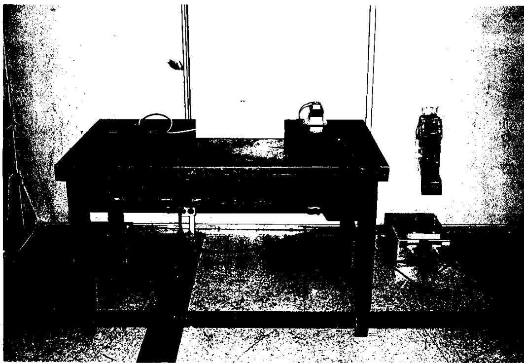
TEST SETUP FOR CONDUCTED EMISSIONS MEASUREMENT MAXIMIZED FOR MEASUREMENT OF WORST CASE EMISSIONS
