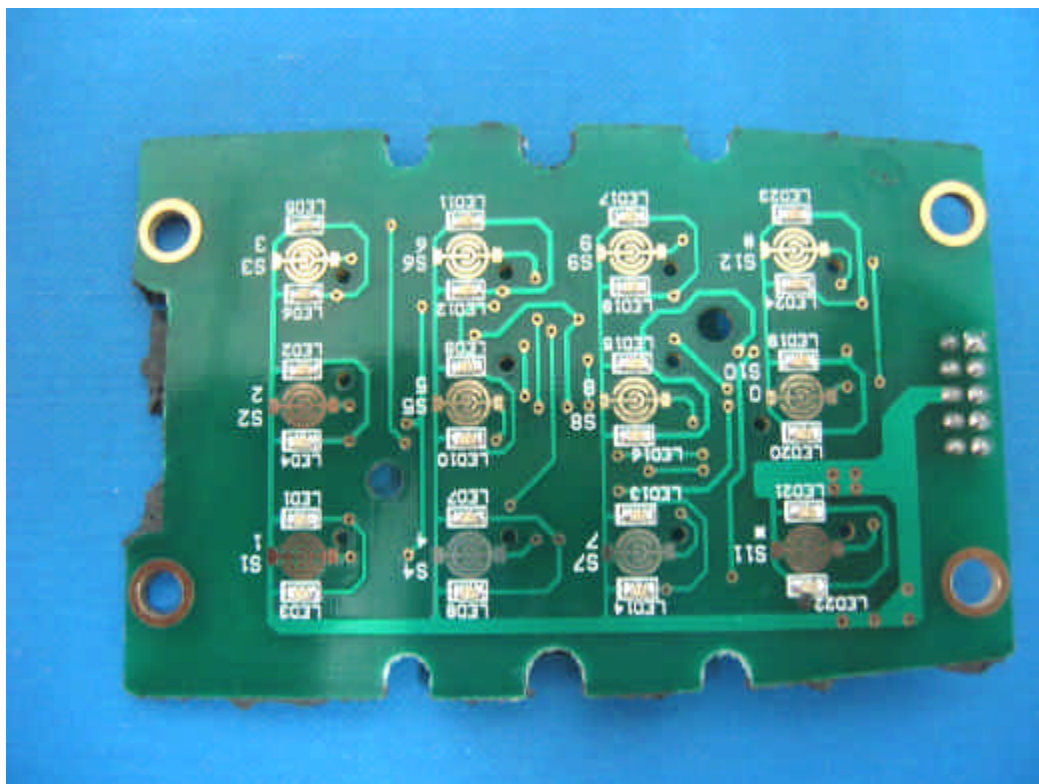
Photograph No.7 AYC-F64 keypad PCB second side view
