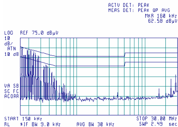
Plot 7.3.6 Conducted emission measurements
