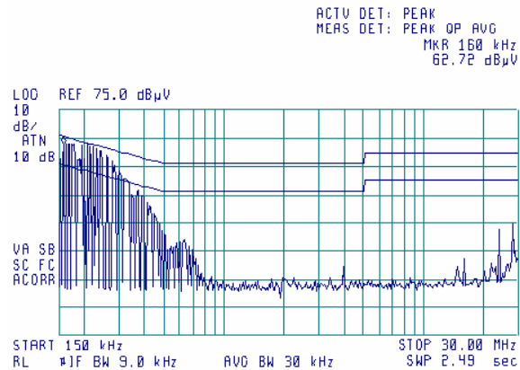
Plot 8.1.4 Conducted emission measurements
