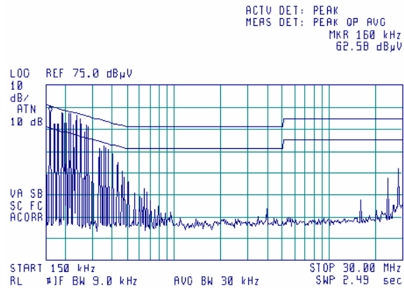
Plot 8.1.6 Conducted emission measurements
