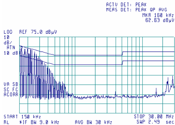
Plot 8.1.2 Conducted emission measurements
