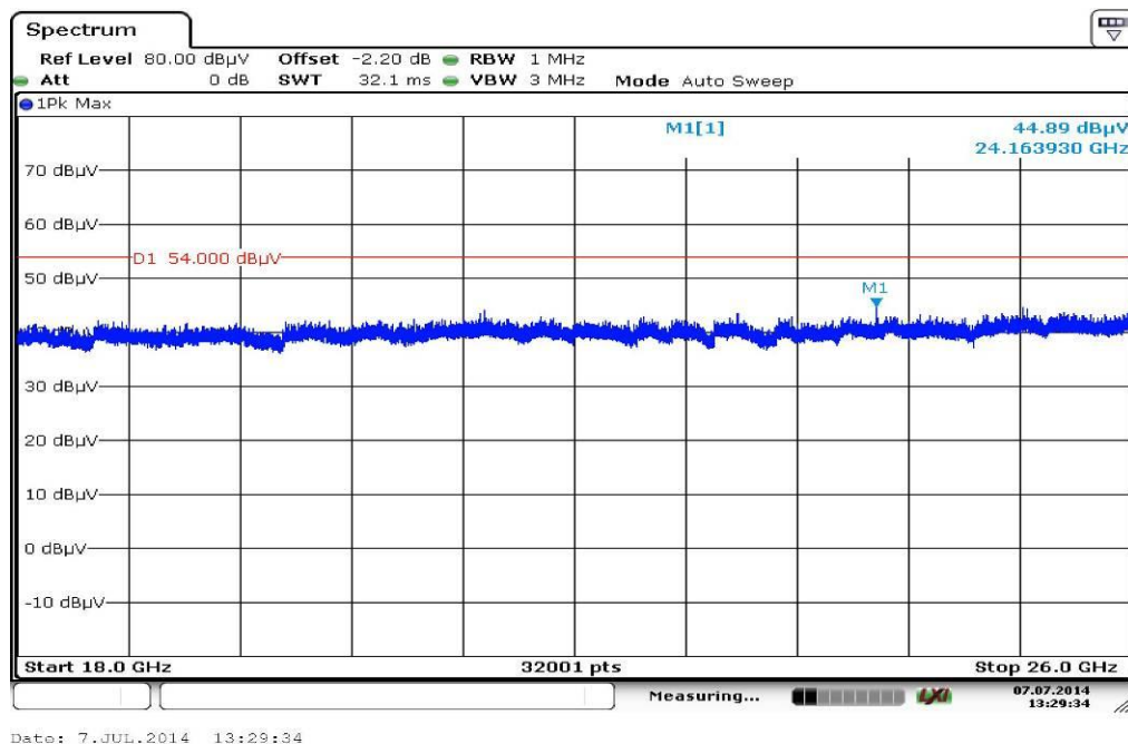
Plot 4: 18 - 26 GHz
