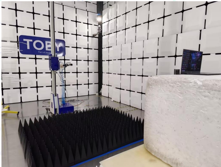
Photo of Setup for Radiated Emission (Above 18-40 GHz)
