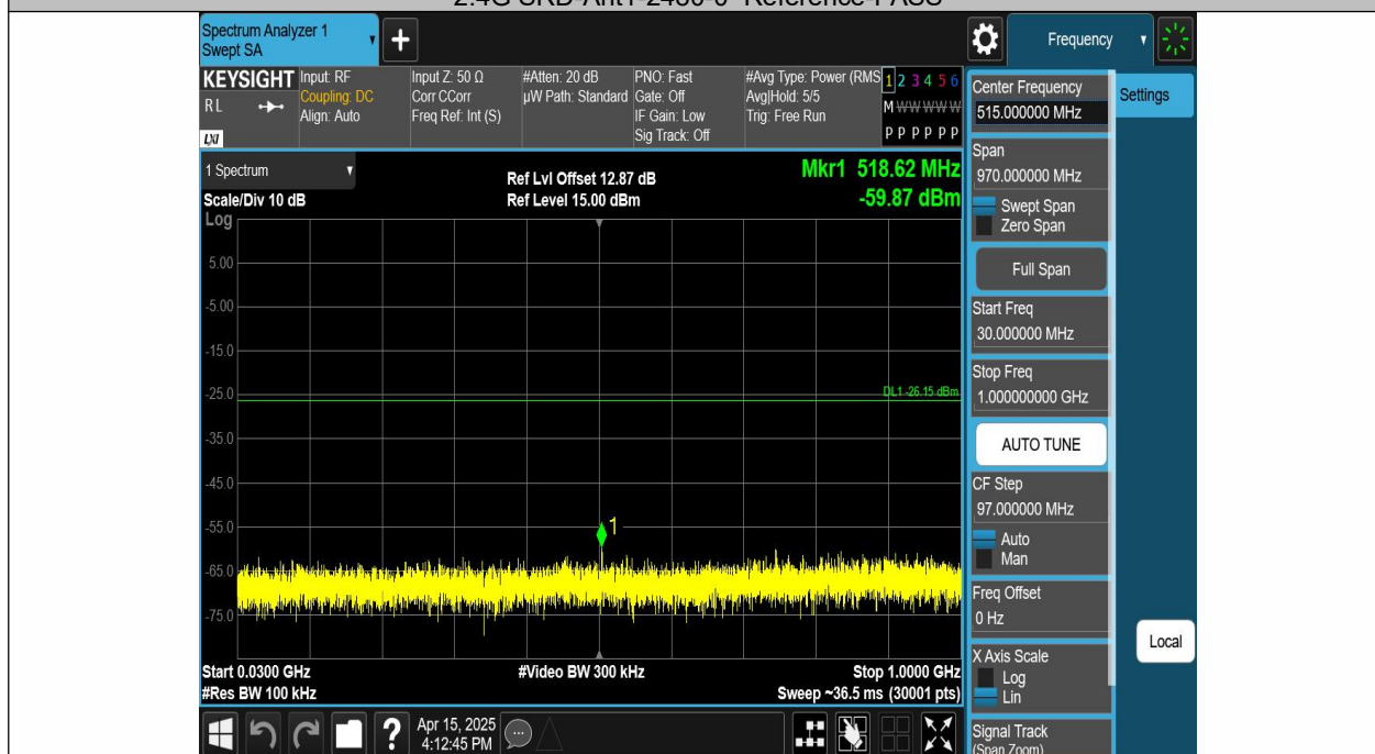
2.4G SRD-Ant1-2480-30~1000-PASS
