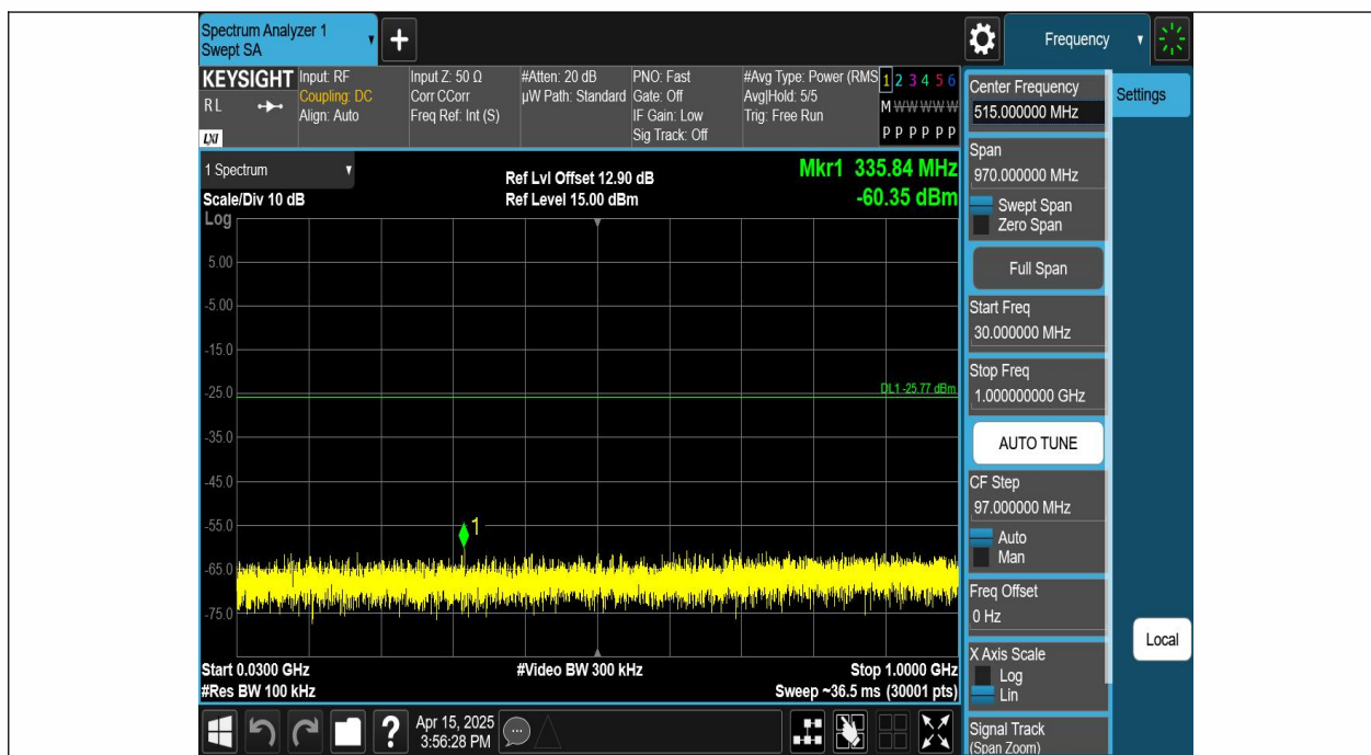
2.4G SRD-Ant1-2440-30~1000-PASS
