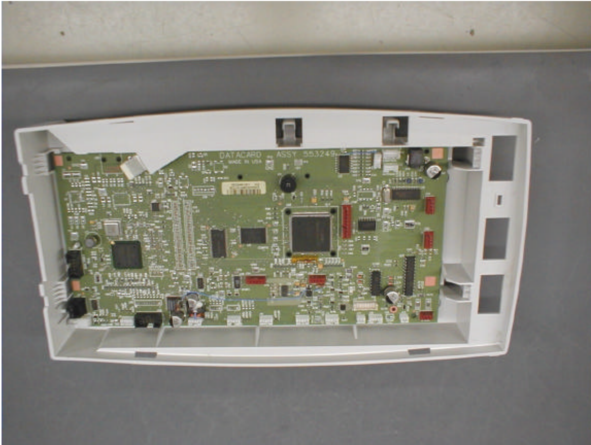
Main board front, in case
