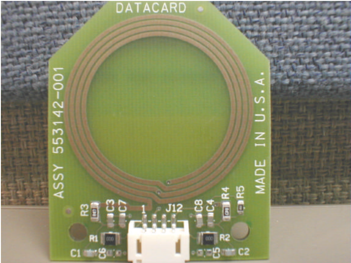
Antenna board front
