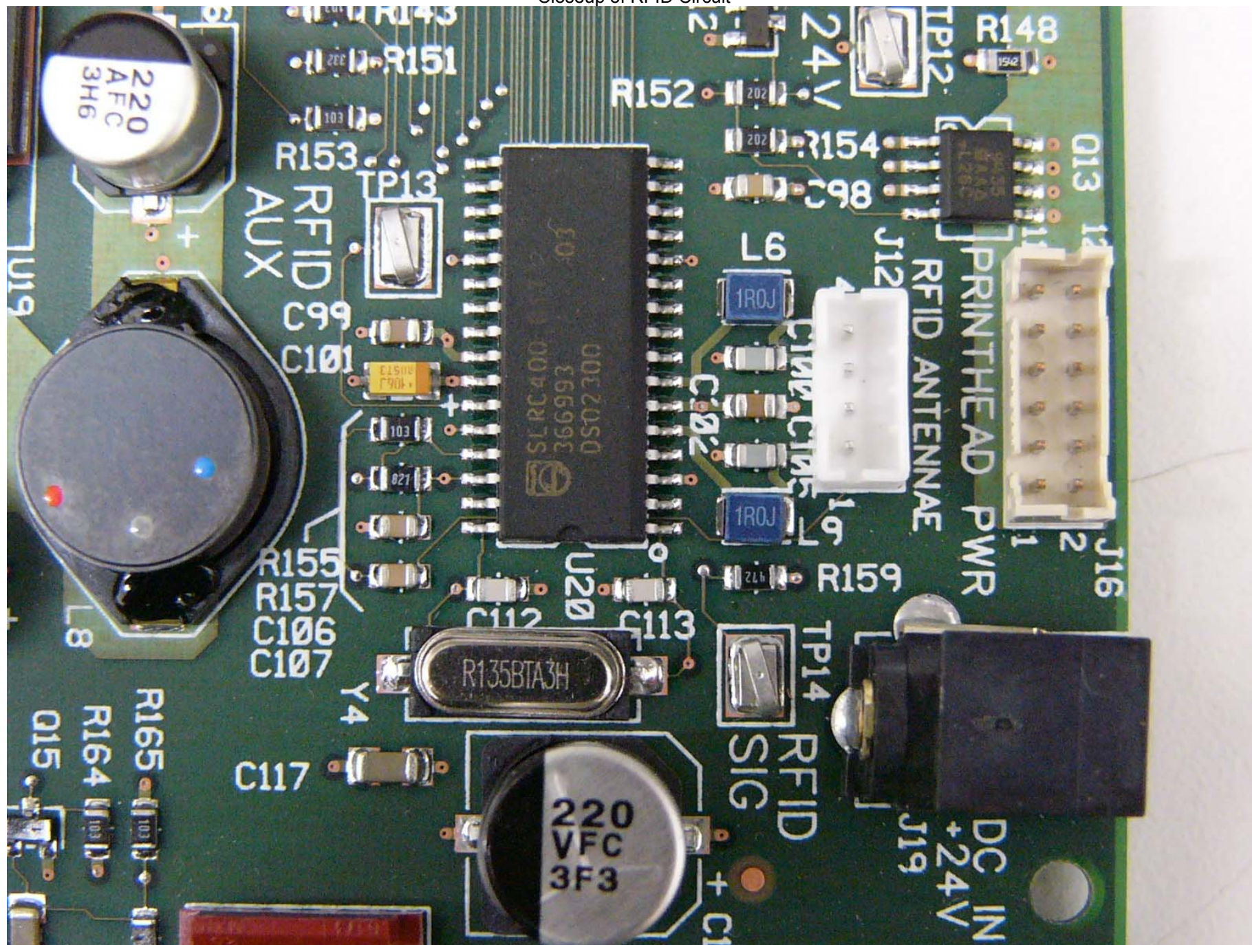
Closeup of RFID Circuit
