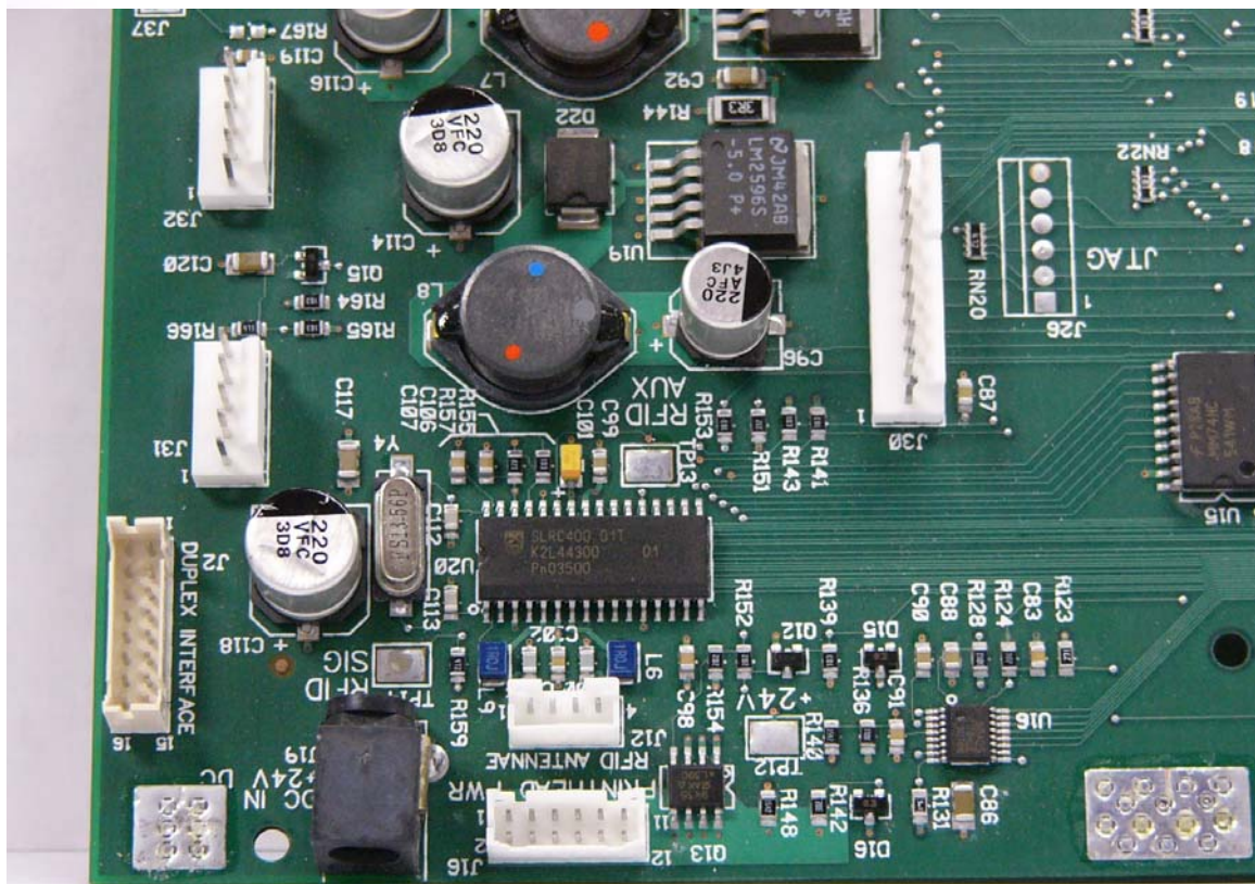
Printing Printed Wiring Board - Top Side - Lower Right
