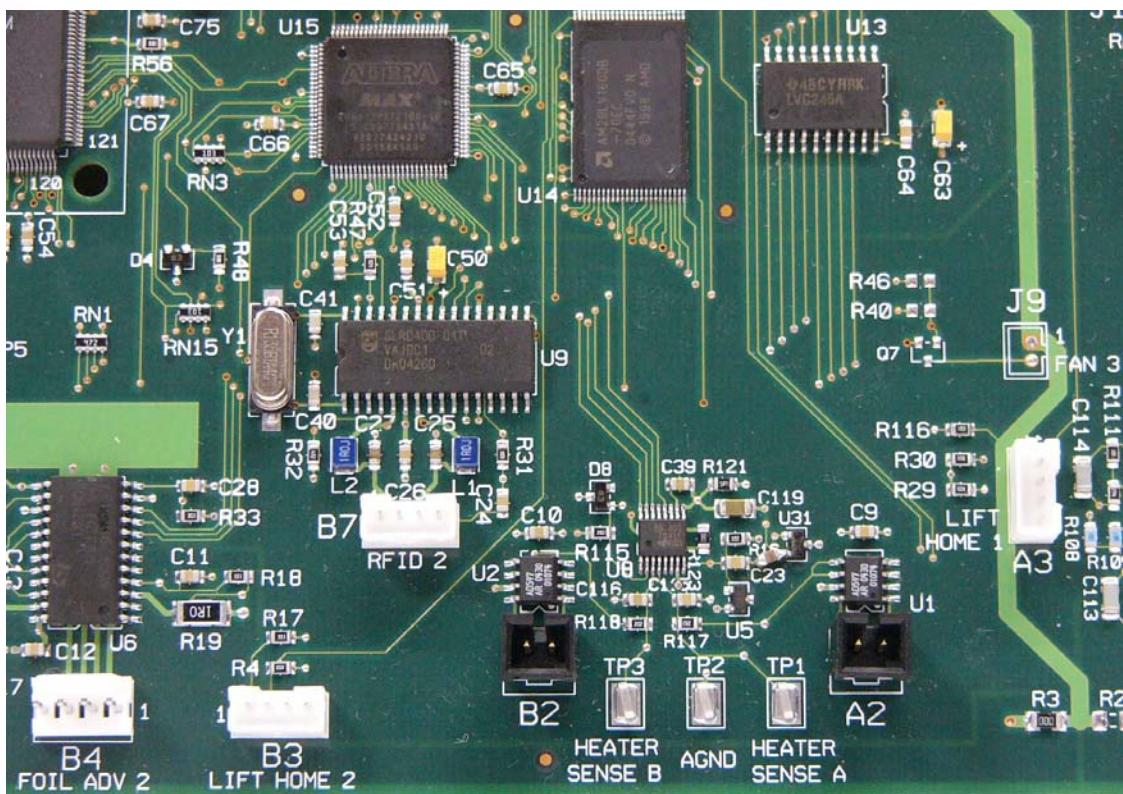
Laminator Printed Wiring Board - Top Side - Lower Center
