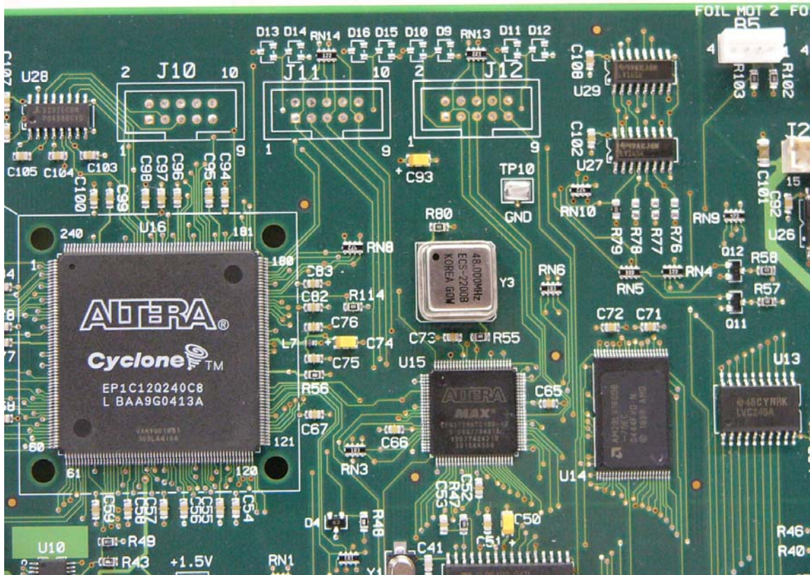
Laminator Printed Wiring Board - Top Side - Upper Center
