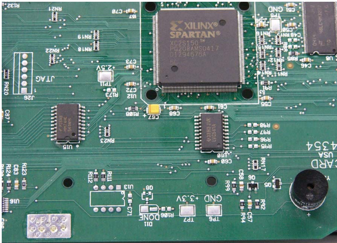
Printing Printed Wiring Board - Top Side - Lower Center
