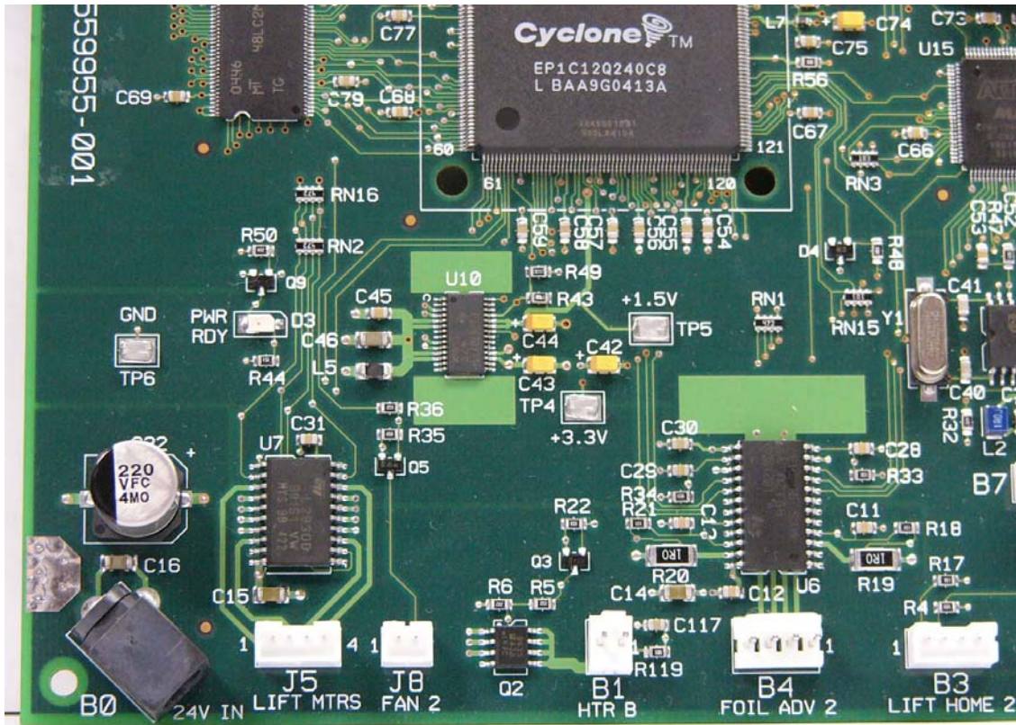
Laminator Printed Wiring Board - Top Side - Lower Left
