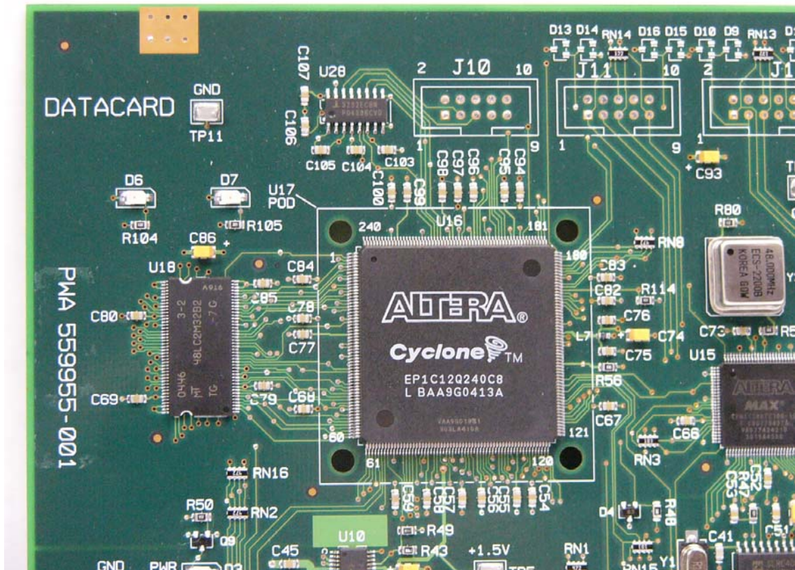
Laminator Printed Wiring Board - Top Side - Upper Left
