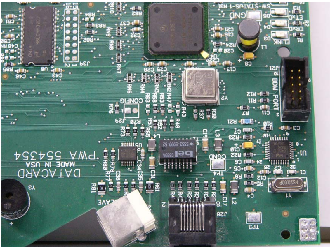
Printing Printed Wiring Board - Top Side - Lower Left
