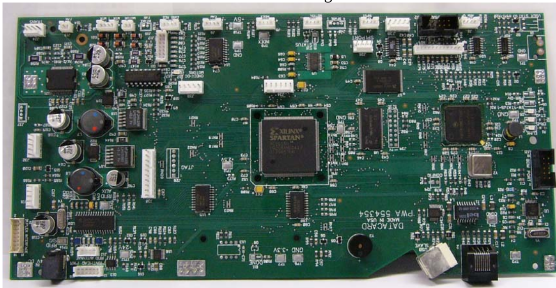
Component Side
