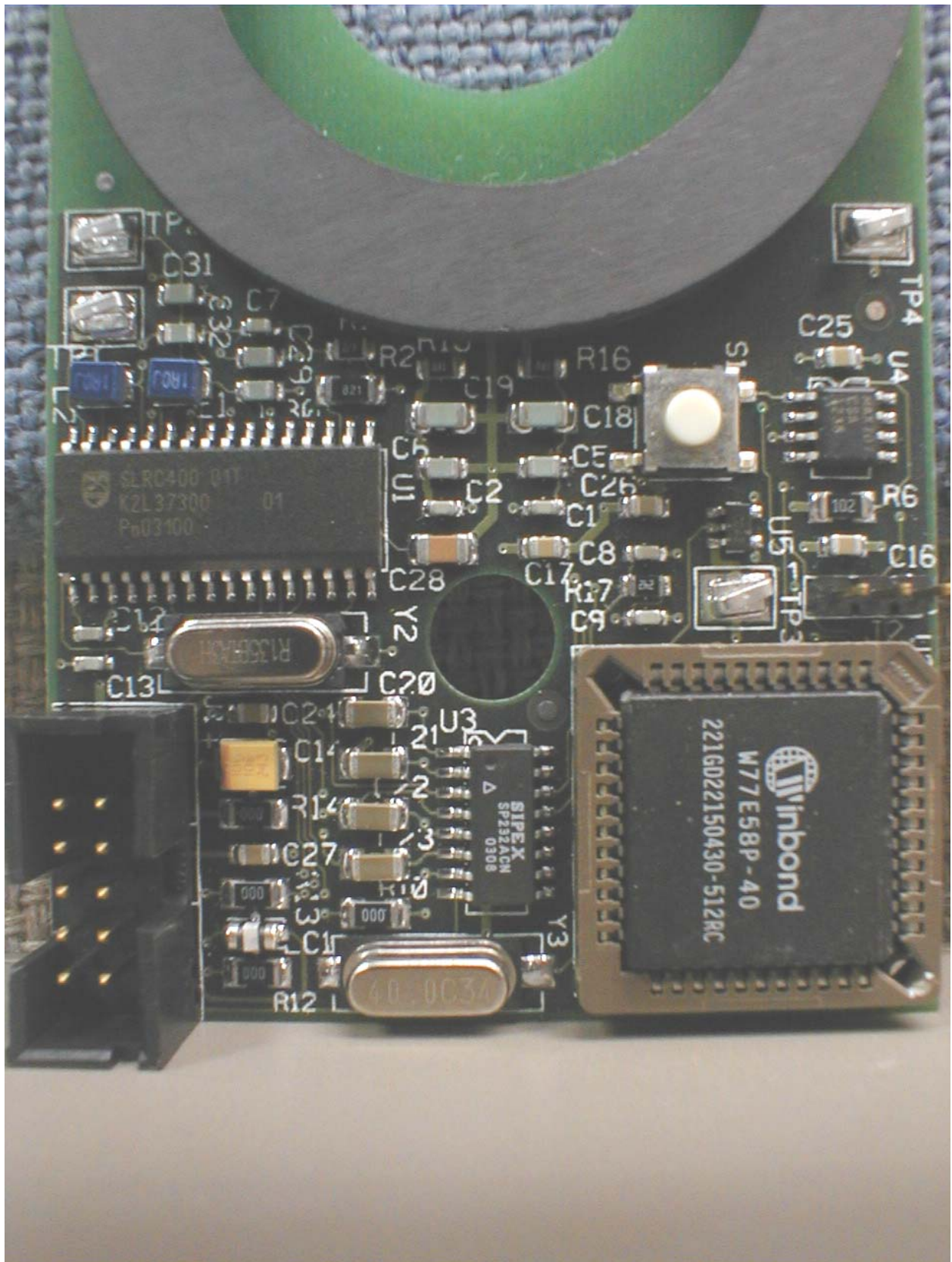
Figure 3 Component Placement for Supplies ID Circuit Board
