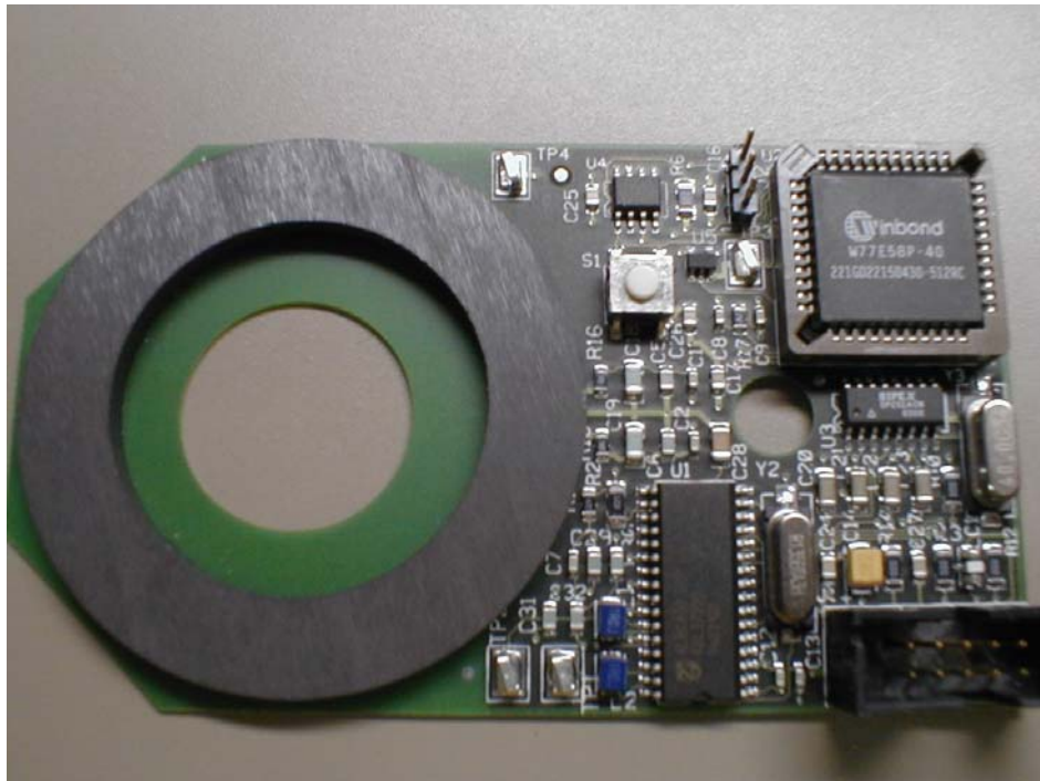
Figure 1 Overall Component side of the Supplies ID Circuit Board
