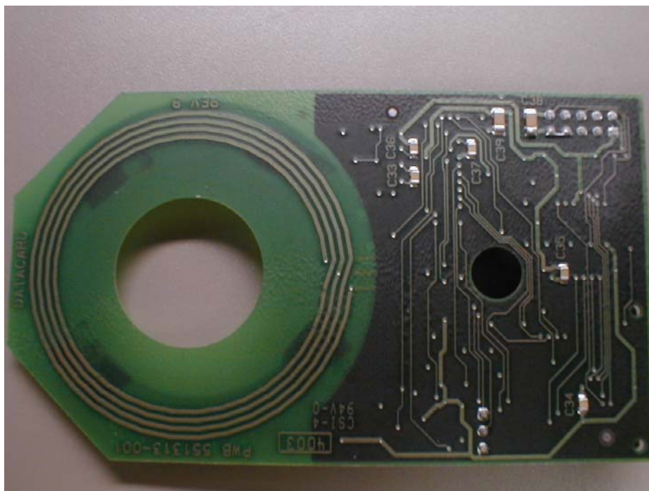
Figure 2 Overall Solder side of the Supplies ID Circuit Board
