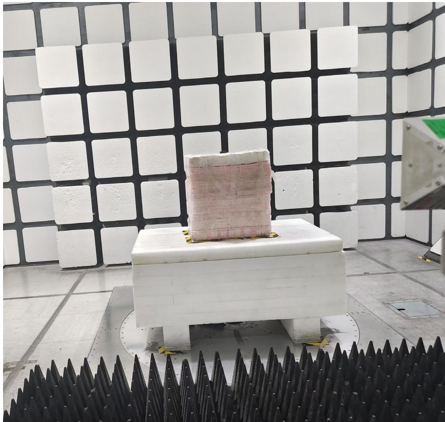
Radiated Emissions View (18-25 GHz)
