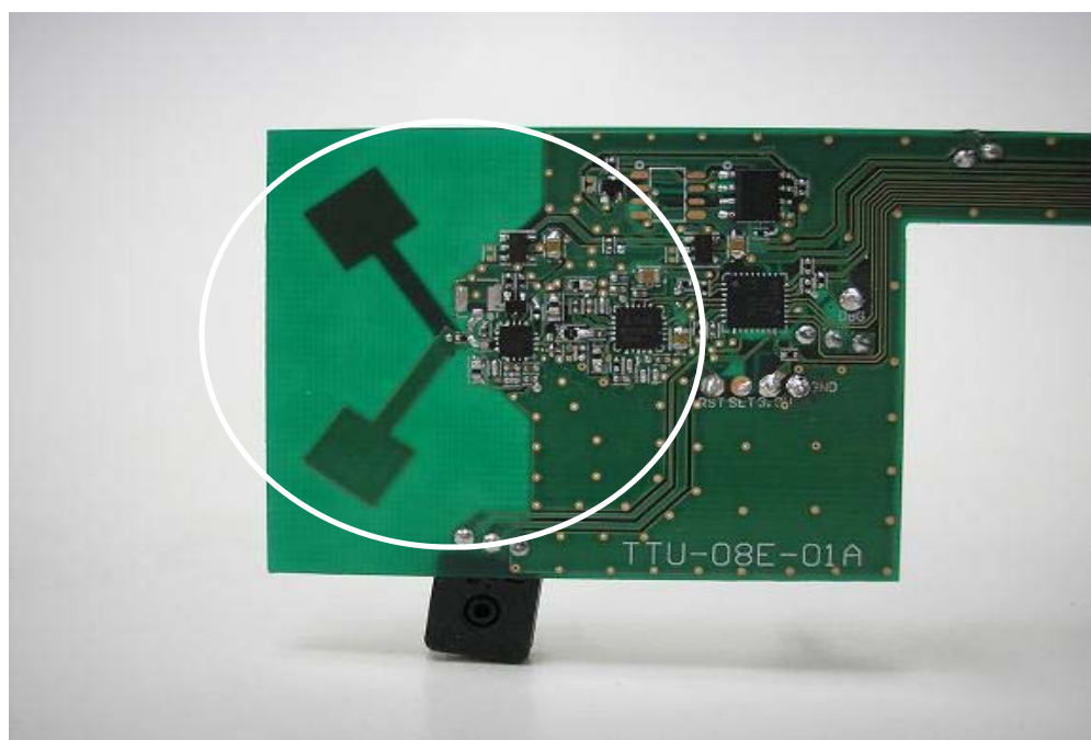
RF Section
