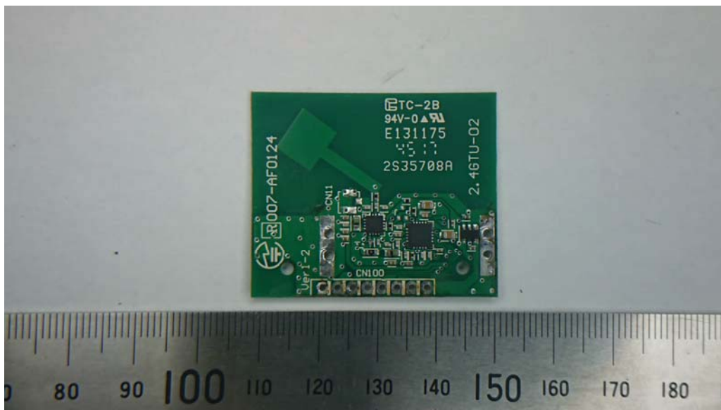
Main PCB (without shield)
