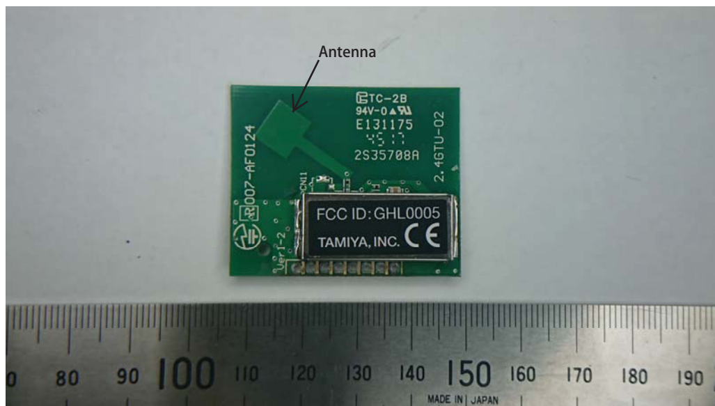
Main PCB (Front)
