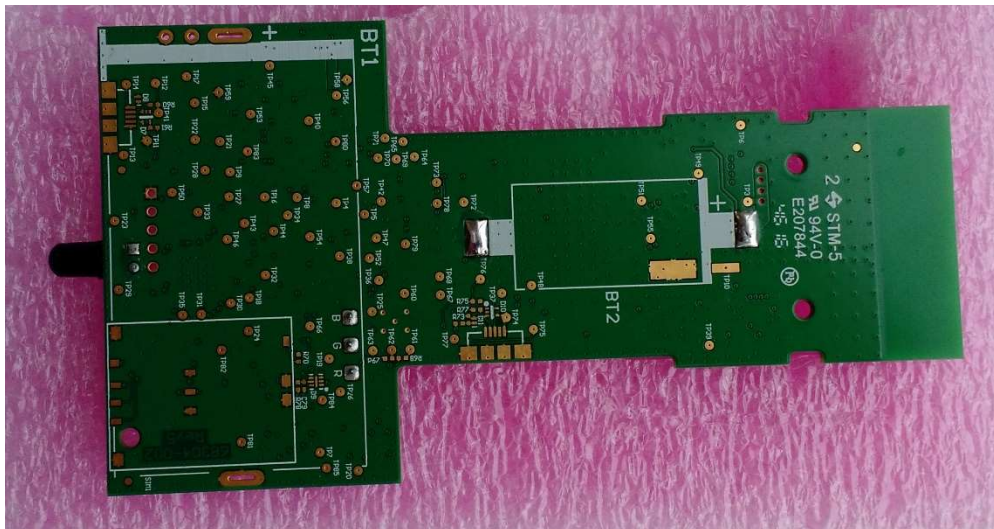
Figure 2 Solder side
