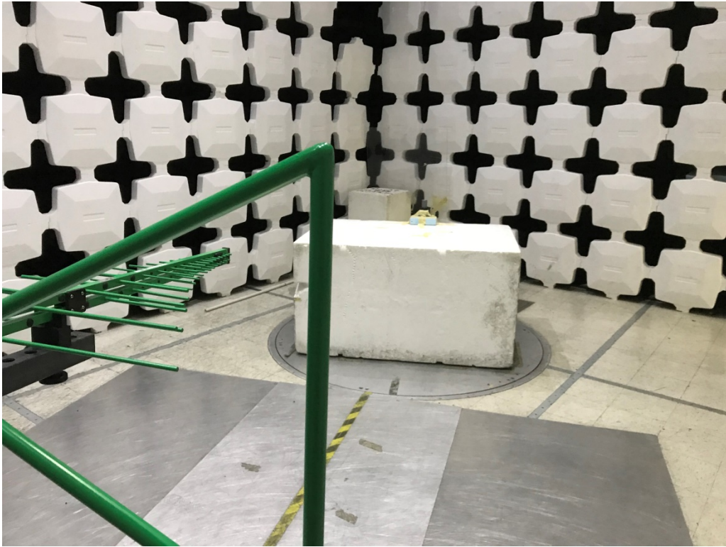
Figure 3 – Receiver Test Setup for Radiated Emissions – 30MHz to 1000MHz, Horizontal Polarization
